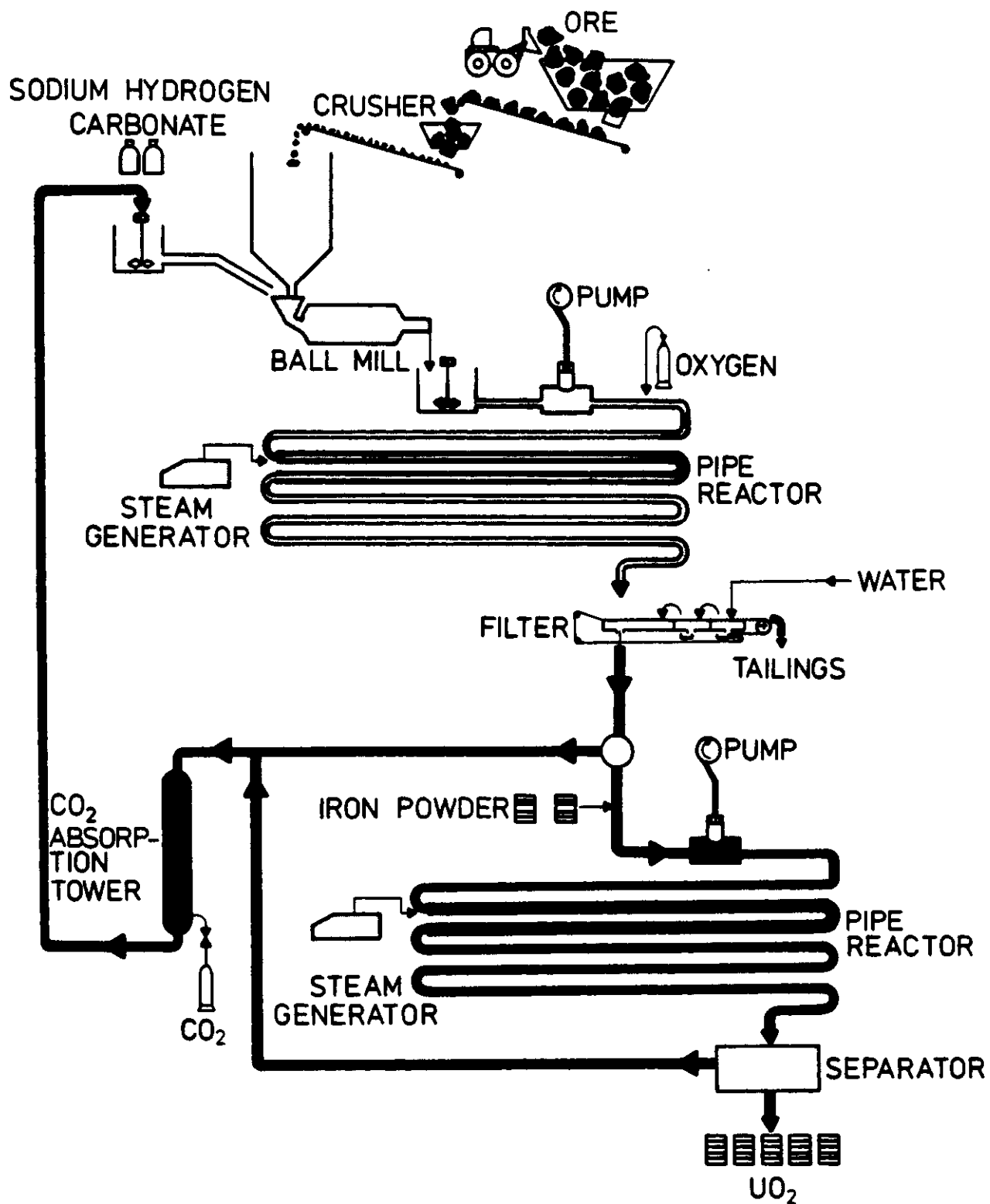
Figure 4-4: Flow-sheet for the uranium extraction process.
