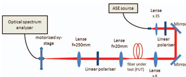
Fig. 1 Experimental S^2 imaging setup.
