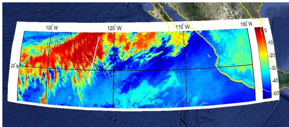
Fig. 1. Structure of a convective system in the eastern Pacific ocean (2 February 2008). Colors denote GOES brightness temperature difference between the 6.5 micron and 11 micron channels, with red denoting high, cold clouds. The black line is the GPS RO tangent point and the white line is the CALIPSO track.
