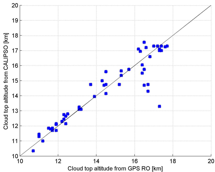
Fig. 4. Scatter plot showing correlation between cloud top height derived from GPS RO (identified from the maximum bending angle anomaly) and the maximum cloud top height from CALIOP.
