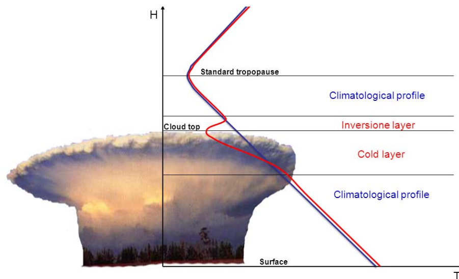
Fig. 9. Atmospheric thermal structure associated with intense convective systems, as observed by GPS RO. The blue line shows a background climatological temperature profile and the red line is the temperature profile during the convective systems.
