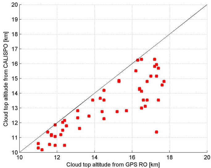
Fig. 5. Scatter plot between cloud top height from GPS ROs (as in Fig. 4) and the average cloud top height (averaged along the satellite orbit track) from CALIOP.
