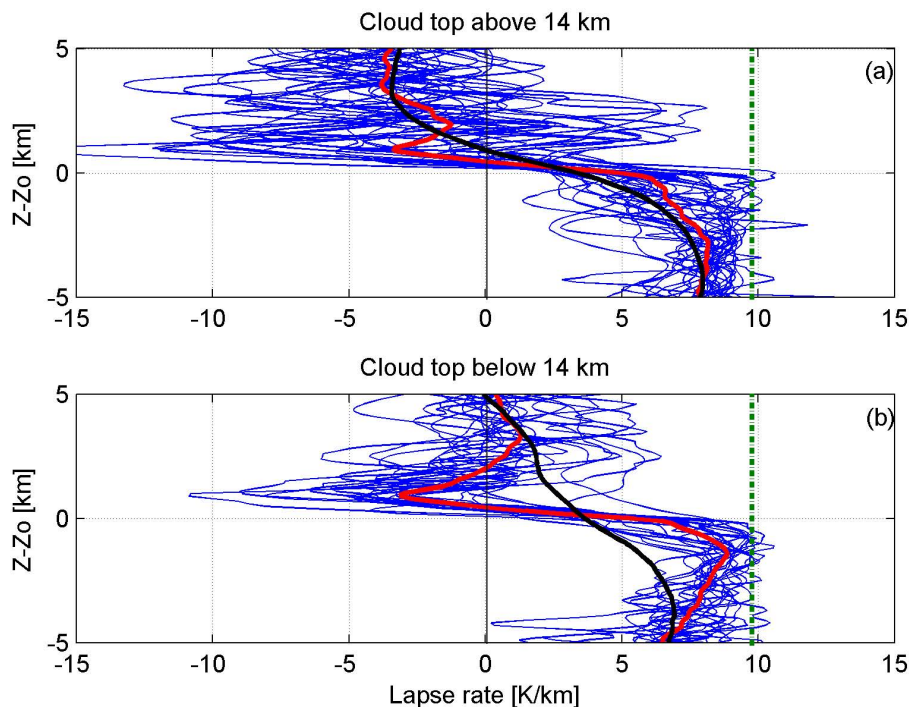
Fig. 8. Vertical profile of the GPS lapse rate ( -dT/dz ) calculated with respect to the altitude of the cloud top derived from the corresponding CALIOP measurements for 53 convective systems (blue lines). The red line is the convective systems average, the black line is the averaged climatological lapse rate and the dotted vertical green line is the dry adiabatic lapse rate ( 9.8 \text{ K km}^{-1} ).
