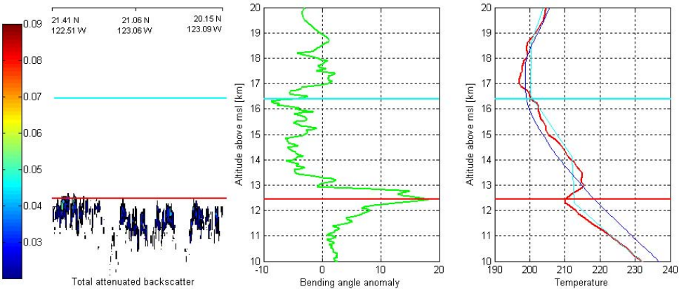
Fig. 2. Vertical profile associated with the convective system identified in Fig. 1 (2 February 2008). The left panel shows the total attenuated backscatter at 532 nm from CALIOP, along the orbit track shown in Fig. 1. The right panels show the bending angle anomaly profile (green) and the temperature profile (red) from GPS RO during the storm. The temperature plot also shows the profile from the ECMWF analysis (cyan) and the climatological temperature profile (blue). The horizontal cyan line is the altitude of the standard tropopause and the horizontal red line is the altitude of the coldest point and the bending angle anomaly spike.
