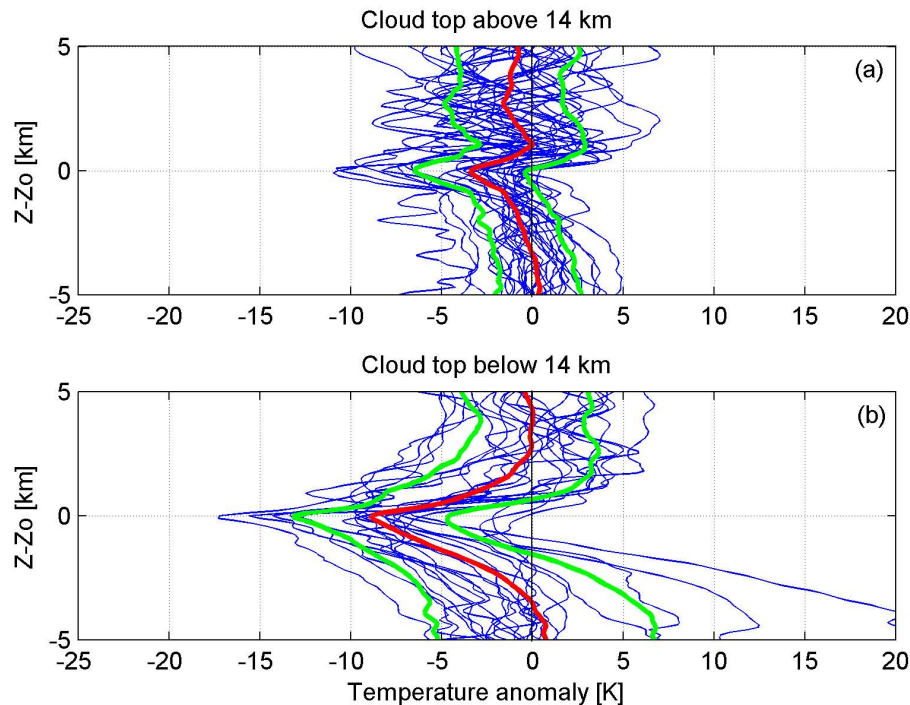
Fig. 7. Vertical profile of the GPS temperature difference between the convective system and the background climatology, calculated with respect to the altitude of the cloud top derived from the corresponding CALIOP measurements. Blue lines show each of the 53 cases, separated according to cloud top above and below 14 km. The red line is the average and the green lines are the average one standard deviation.
