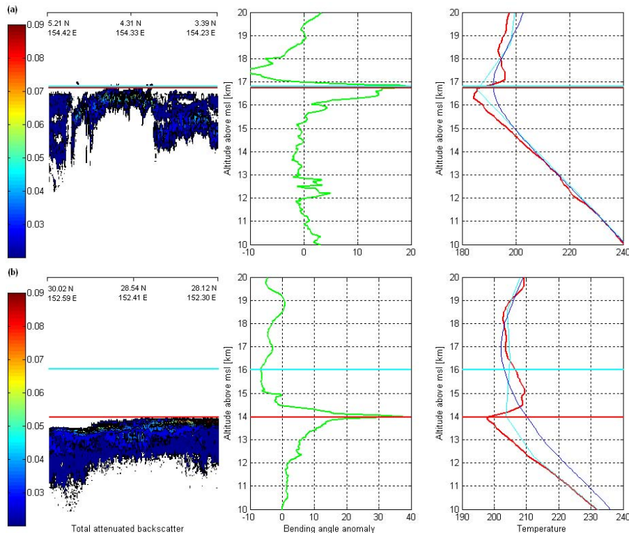
Fig. 3. Two examples of convective systems reaching different altitude: 22 January 2008 (top panel) and 14 April 2008 (bottom panel). The left panels show the total attenuated backscatter at 532 nm from CALIOP, and the right panels show the bending angle anomaly profile (green), the temperature profile from GPS RO during the storm (red), the temperature profile from ECMWF analysis (cyan) and the climatological temperature profile (blue). The horizontal cyan line is the altitude of the standard tropopause and the horizontal red line is the altitude of the coldest point and the bending angle anomaly spike.
