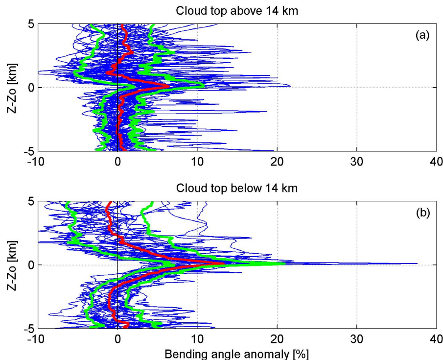
Fig. 6. Vertical profile of the GPS bending angle anomaly, calculated with respect to the altitude of the cloud top derived from the corresponding CALIOP measurements. Blue lines show each of the 53 cases, separated according to cloud top above and below 14 km. The red line is the average and the green lines are the average one standard deviation.
