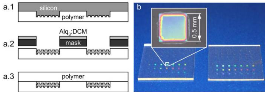
Fig. 1. Scheme of the main fabrication steps of all-polymer chips comprising encapsulated organic semiconductor lasers. (a.1) Thermal nanoimprint. (a.2) Evaporation of \text{Alq}_3 :DCM. (a.3) Hermetic sealing by thermal bonding. (b) Photograph of two chips of the size of a microscope cover slip ( 18 \times 18 \text{ mm}^2 ) with encapsulated lasers and a microscope image of a laser (inset). The lasers can be identified by light diffracted from the nanostructures. The left chip consists of PMMA the right one of COC.
