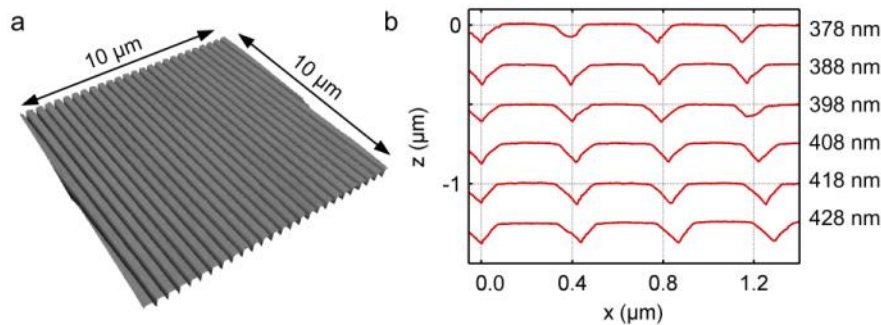
Fig. 2. (a) Exemplary atomic force micrograph of a nanoimprinted DFB grating on a HesaGlas ® VOS PMMA substrate. The depth of the trenches is 140 nm. (b) Atomic force micrographs of six different PMMA gratings with varying period on one substrate.
