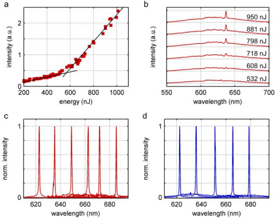
Fig. 3. (a) Input-output curve of an encapsulated PMMA laser and (b) corresponding spectra of the same laser for selected pump energies. (c) Spectra of different lasers pumped well above threshold all integrated on one PMMA chip. Grating periods are 378, 388, 398, 408, 418, and 428 nm. (d) Spectra of lasers on one COC chip for grating periods of 378, 388, 398, 408, and 418 nm.
