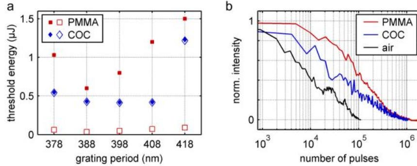
Fig. 4. (a) Threshold of PMMA and COC lasers for grating periods from 378 nm to 418 nm. The device thresholds are plotted with solid symbols. As the polymer material absorbs the pump light partially estimated laser thresholds are plotted using open symbols. (b) Lifetime measurements of an encapsulated PMMA laser and an encapsulated COC laser in comparison to an unencapsulated laser.
