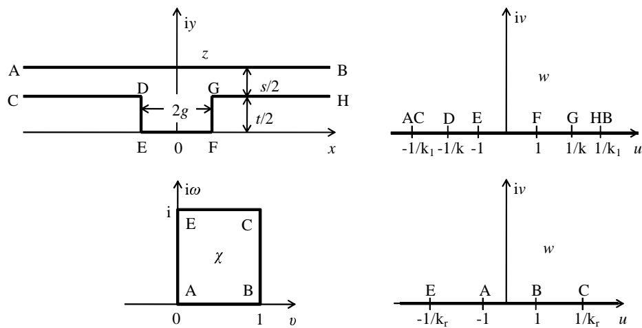
Fig. 1. Sketch of the rib ARROW waveguide cross-section in the z -plane and the upper half-plane w to which the rib ARROW structure is mapped conformally. Below, the square in the \chi -plane to which the upper half-plane w is mapped in a second conformal mapping step.
