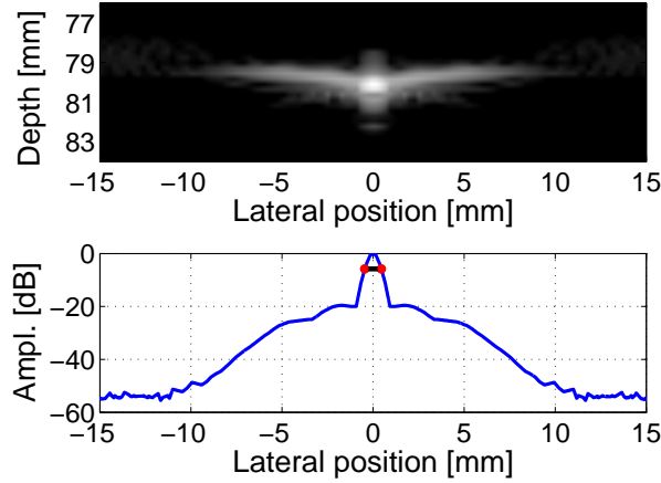
Figure 2.2: Illustration of a B-mode image of a point spread function (top) and lateral beam profile (bottom). The black line and the two red dots indicate the distance FWHM.
