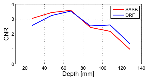
Figure 4.21: Measured CNR for the B-mode images shown in Fig. 4.20.
