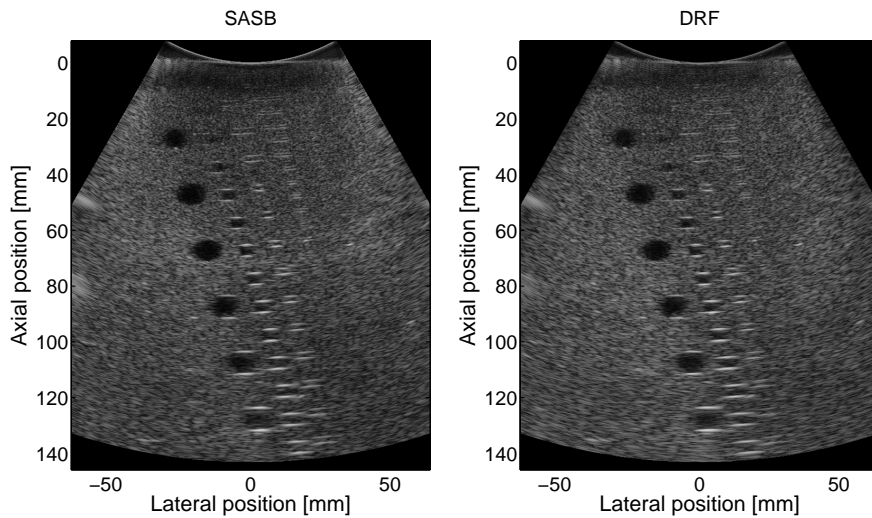
Figure 4.20: B-mode images of the contrast phantom, Model 571, using SASB and DRF. Dynamic range is 60 dB. A digital TGC is applied on both images for a uniform speckle level through depth. The median speckle level of each image is normalized to each other.
