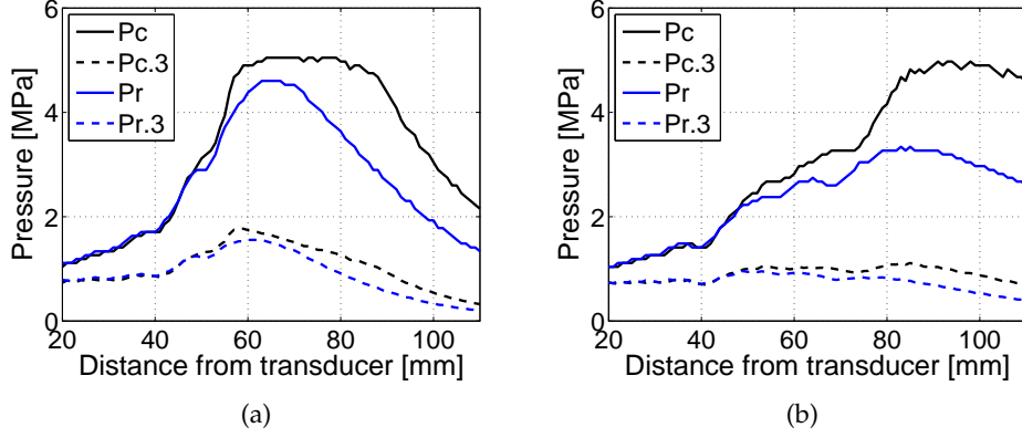
Figure 5.9: Measured peak compressional and rarefactual pressure as function of distance from the transducer. (a) for the SASB configuration and (b) for the DRF configuration. The profiles are shown for both the water measurement and derated using an attenuation coefficient of 0.3dB/cm/MHz.
