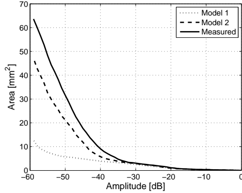
Fig. 7. Area covered by the point spread function from the scatter at 79.4 mm.
