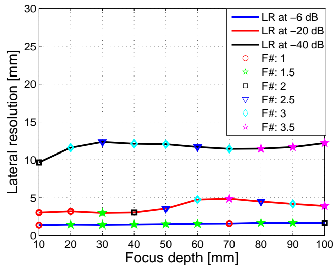
Figure 4.8: Simulated avg. lateral resolution as function of focus depth, and F#. The avg. lateral resolution for each configuration is calculated as an avg. from 14 point targets ranging from 10 to 140 mm. For each focus depth the configuration with the best lateral resolution is shown. The markers indicate which F# that is used in the respective configurations. The blue line indicate the FWHM, the red line the lateral resolution at -20 dB, and the black line the lateral resolution at -40 dB.
