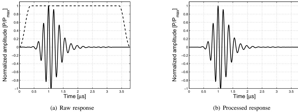
Fig. 4. Measured pulse echo response for the center element. In (a) the solid line indicates the raw response and the dashed line the applied Tukey window, (b) shows the averaged and Tukey windowed response.
