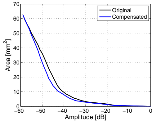
Figure 6.7: Area covered by the point spread function from the scatter at 79.4 mm, pre and post compensation for the phase error.
