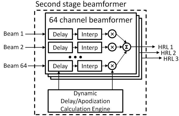
Figure 4.4: Block diagram of the second stage beamformer. The beamformer has 64 input channels for local storage in the beamformer. The delay and apodization of each channel is controlled by the dynamic delay and apodization control unit. The beamformer can generate 3 output lines.
