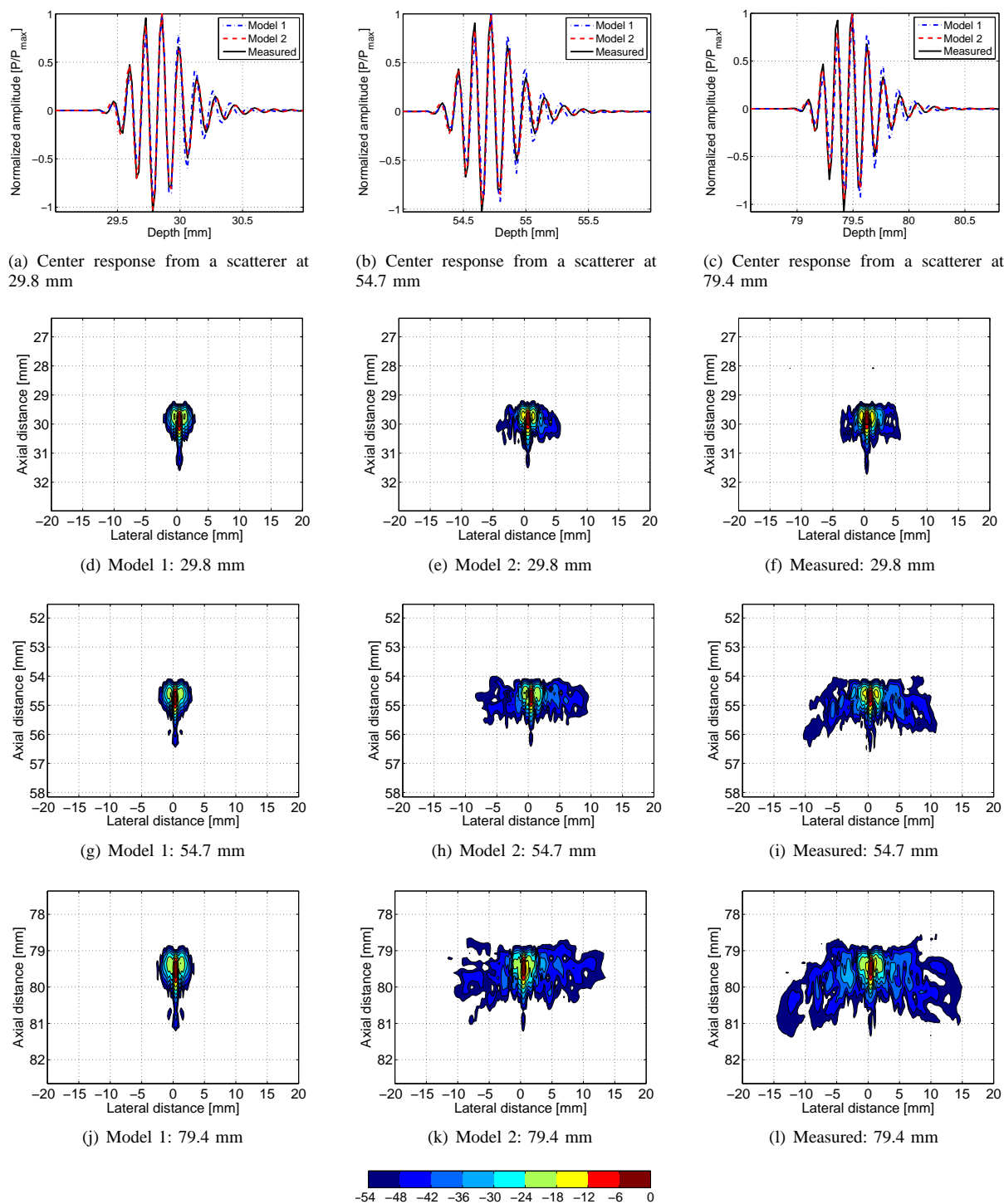
Fig. 6. Fig. (a) to (c) illustrates the measured and simulated second stage SASB responses from the center scan line from three scatterers at (a) 29.8 mm, (b) 54.7 mm, and (c) 79.4 mm from the transducer surface. Fig. (d) to (l) illustrates contour plots with 6 dB contour coloring for the three scatterers using Model 1 in (d,g,j), Model 2 in (e,h,k), and measured response in (f,i,l).
