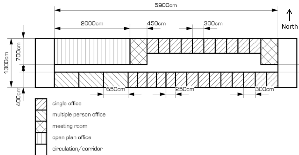
Figure 36. Typical floor plan with a total heated area of 3.068 m 2 (from Leenknecht and Vandermaesen [74]).
