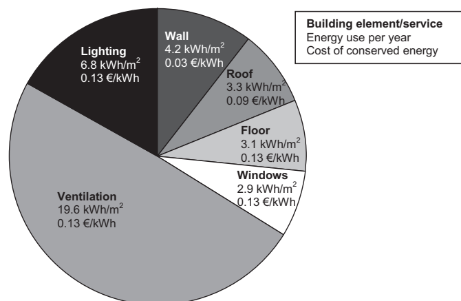
Fig. 7. The distribution of the energy uses in the economically optimal solution for the case example.
