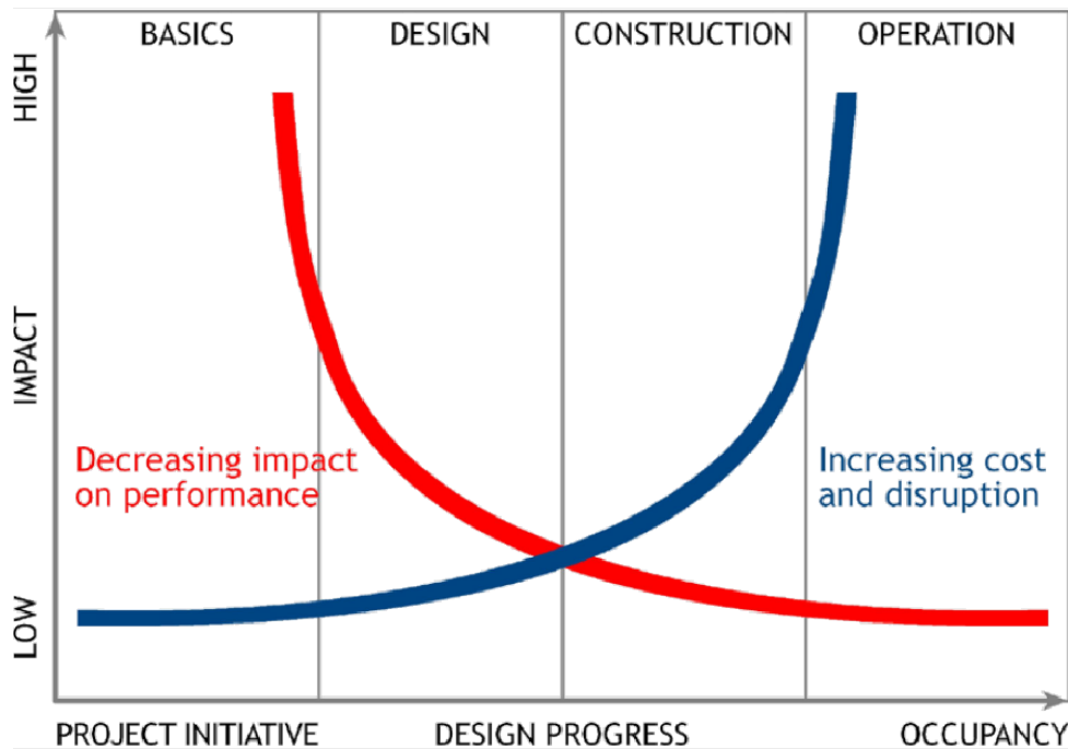
Figure 2. Relation between life of building and design decisions' impact on performance and cost (from IEA task 23 [29]).
