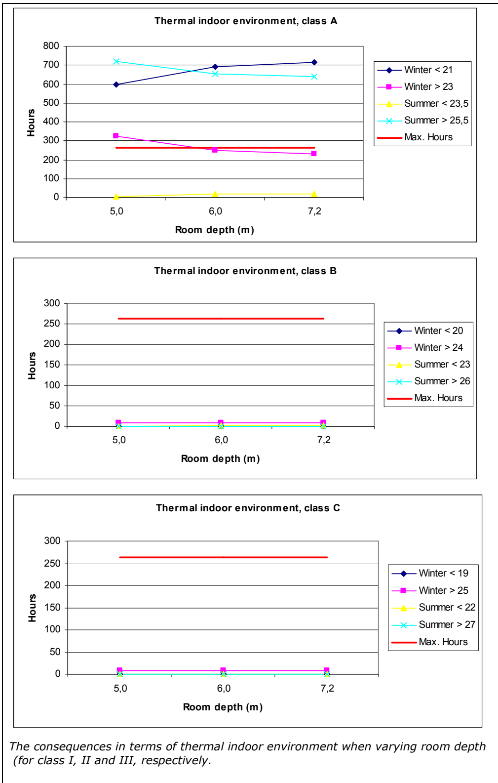
Figure 16. Output from an early version of the tool (2006). The result of a parameter variation was manually generated by copy/pasting simulation results in to an Excel spreadsheet.
