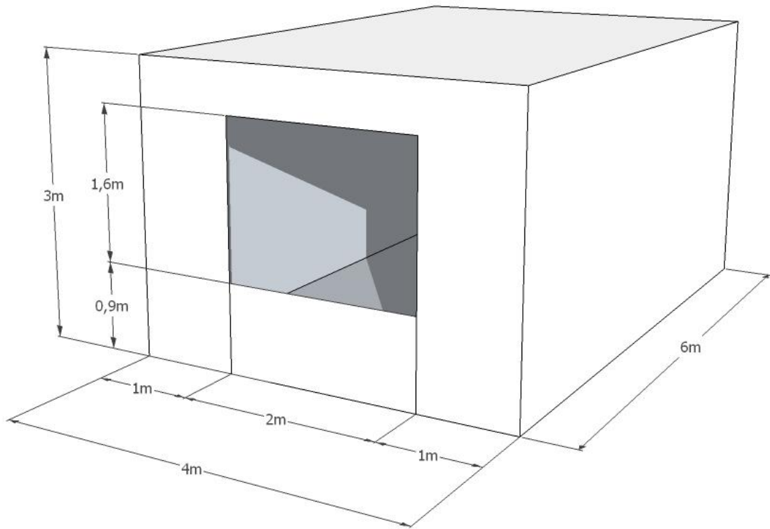
Figure 4. Dimensions of the validated room.
