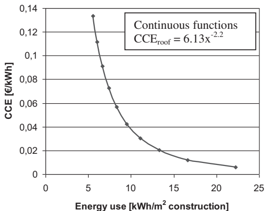
Fig. 2. Example of a continuous function for a continuous measure.
