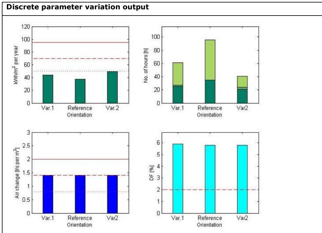
Figure 20. Overview of output from parameter variation (discrete measure), iDbuild version 2.4.2 (2007).
