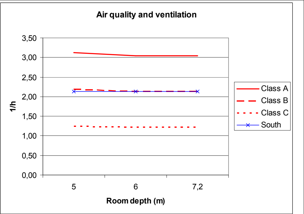
The consequence in terms of air quality when varying room depth.
