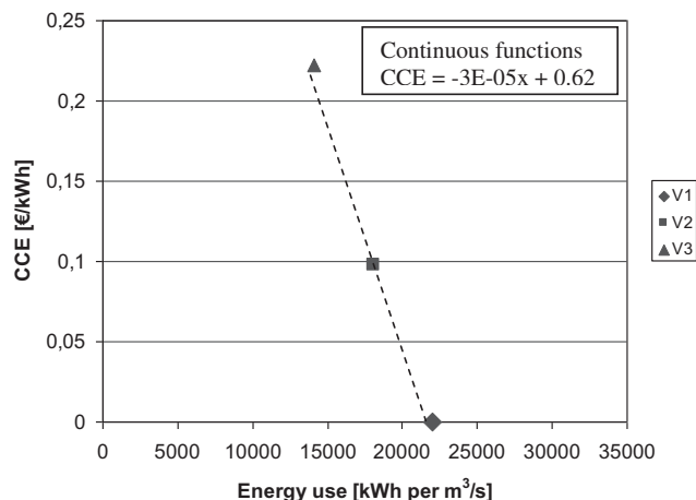
Fig. 5. CCE as a function of energy use for mechanical ventilation.
