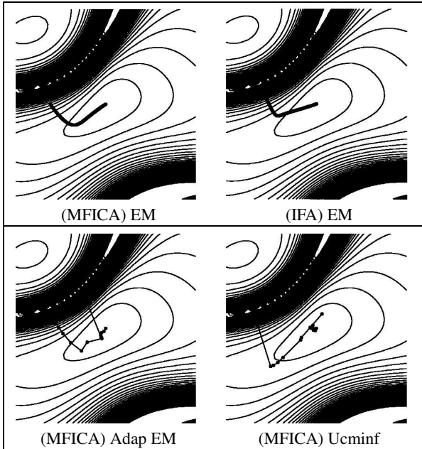
Fig. 3. The (projected) path in A-space for different optimization techniques on the example of Sec. 3.
