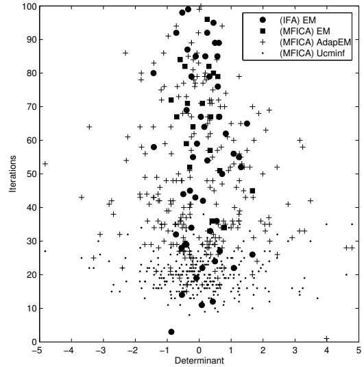
Fig. 4. The influence on the iterations of the determinant for 2x2 mixing matrices. On the first axis is \det(\mathbf{A}) and on the second axis is number of iterations for EM (MFICA).
