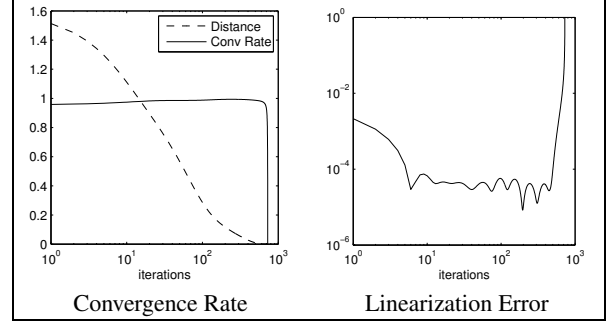
Fig. 2. MFICA: An example of EM slowdown. Left: The convergence rate. Right: The error induced when applying the approximation of Eq. 1
