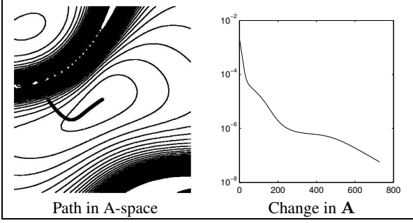
Fig. 1. MFICA: An example of EM slowdown. Left: The (projected) path of EM in A-space. Right: The change of \mathbf{A} over iterations.
