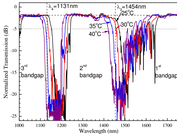
Fig. 5. Transmission spectra at 25^\circ\text{C} (black), 30^\circ\text{C} (red), 35^\circ\text{C} (blue), and 40^\circ\text{C} (purple) of the central-line sample infiltrated with 1.68-RI liquids.
