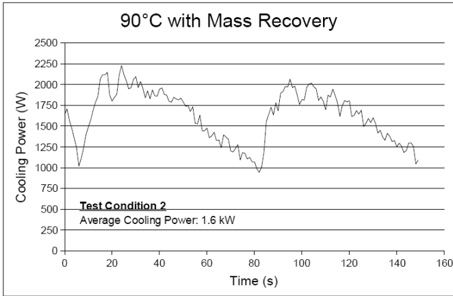
Figure 7: Variation of cooling production Figure 7: Variation de la production frigorifique
