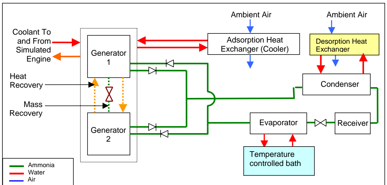
Figure 4: Schematic diagram of Laboratory MACS
