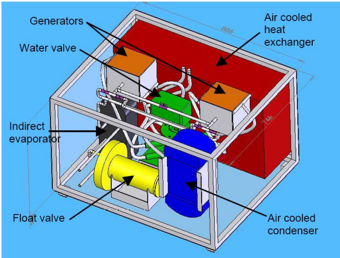
Figure 10: New MACS laboratory prototype – Version 2 Figure 10: Nouveau prototype de laboratoire de la MACS – Version 2
