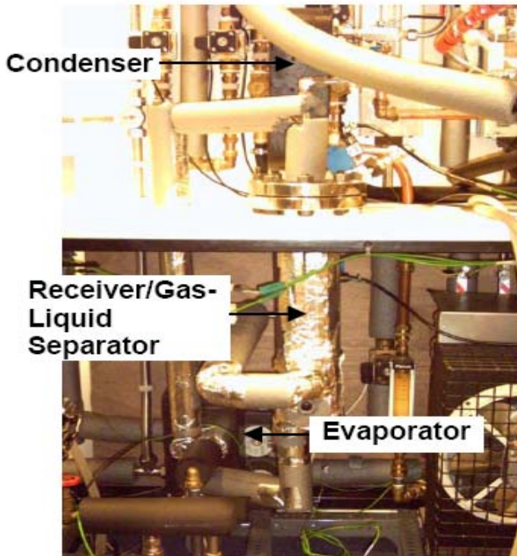
Figure 6: Laboratory MACS: Evaporator and condenser view
