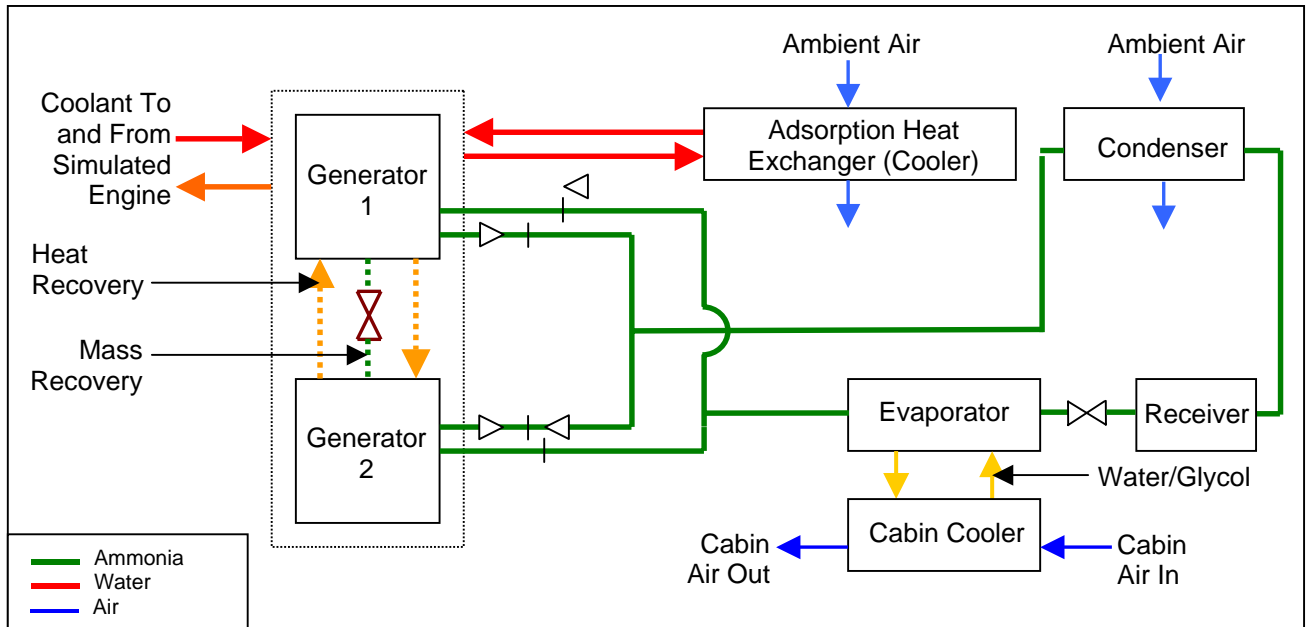
Figure 9: Laboratory MACS – Version 2 Figure 9: MACS en laboratoire – Version 2
