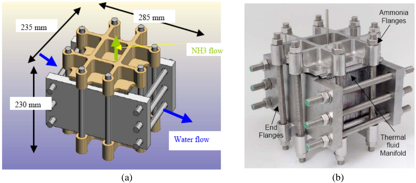
Figure 3: Novel compact sorption generator – (a) Concept design – (b) Experimental prototype
