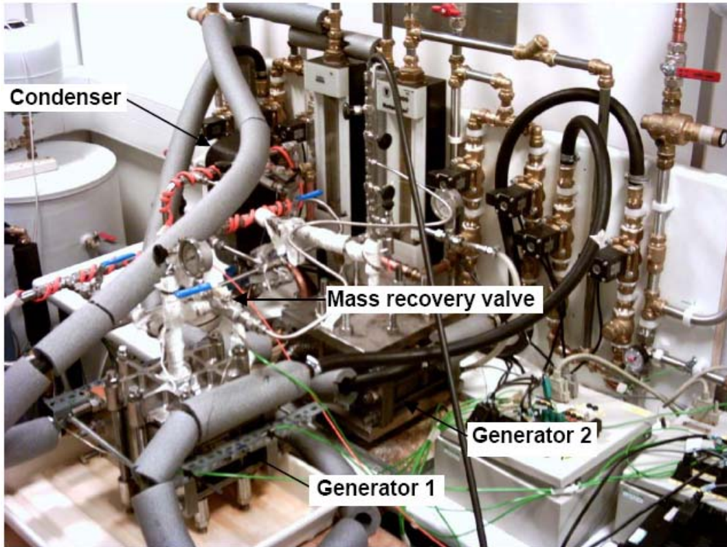
Figure 5: Lab MACS: Generators and condenser view
