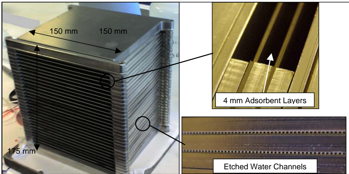
Figure 2: Plate heat exchanger generator design
