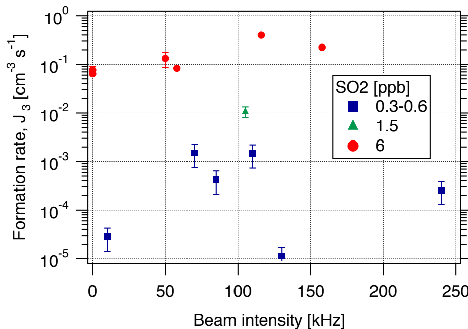
Fig. 7. Particle formation rate, J_3 , vs. beam intensity for several SO 2 concentrations. Where the error bars are not seen, they are smaller than the size of the data points. Although the data show no correlation with beam intensity – with the exception of the measurements taken at 6 ppb [SO 2 ] (see Fig. 8) – the experimental variables (such as [H 2 SO 4 ] and background organic vapours) were not well enough controlled to exclude the presence of ion-induced nucleation on the basis of this plot.
