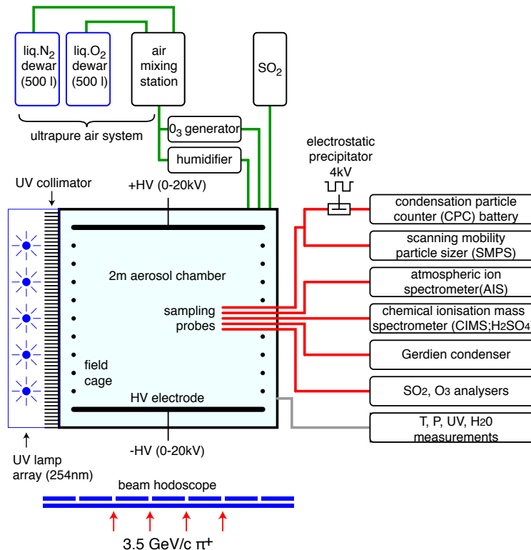
Fig. 1. Schematic diagram of the 2006 pilot CLOUD experiment.
