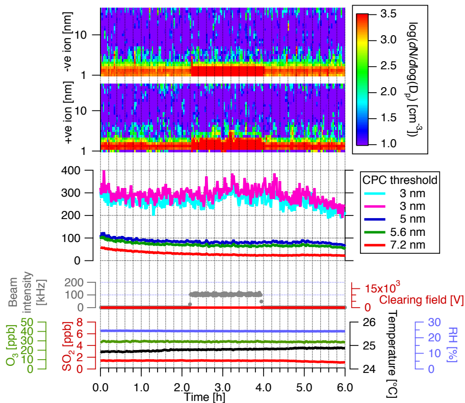
Fig. 6. Time evolution of run 28. At 02:12 h the \pi^+ beam was turned on at 100 kHz rate (grey curve). However only a mild increase was observed in the particle concentration (magenta and cyan curves in the centre panel), indicating negligible ion-induced nucleation. The other chamber conditions (including UV intensity, which is not shown) remained steady throughout this run.
