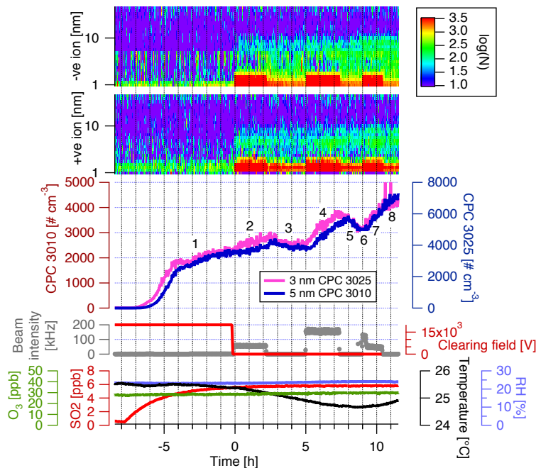
Fig. 4. Time evolution of run 35 (the final run of the campaign). A neutral nucleation burst begins about 7 h before the beam is first turned on at 00h00. Subsequently, the correlation of the beam hodoscope counts (grey curve) and the aerosol particle concentrations (magenta and blue CPC curves) suggests an additional component from ion-induced nucleation. A zoom of the measurements from the individual instruments in the CPC battery is shown in Fig. 5. The numbered regions correspond to the aerosol formation rate measurements summarised in Table 1.
