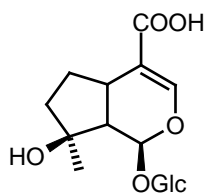
2; Mussaenosidic acid
