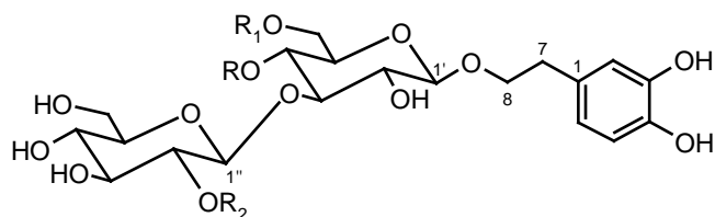
9; R=Caffeoyl; R 1 =H; R 2 =Glc; Chionoside J 10; R=H; R 1 =Feruloyl; R 2 =Glc; Scroside C 11; R=H; R 1 =Caffeoyl; R 2 =Glc; Isochionoside J 12; R=H; R 1 =Caffeoyl; R 2 =H; Plantamajoside
