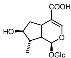
3; 8-Epiloganic acid
