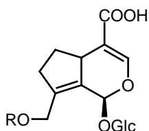
5; R=H; Arborescosidic acid 5a; R=Acetyl; Alpinoside
