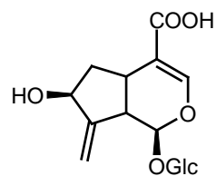
4; Gardoside
