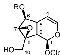
7; R=H; Catalpol 7a; R=Benzoyl; Veronicoside 7b; R=3,4-di-OH-Benzoyl; Verproside 7c; R=Vanilloyl; Amphicoside 7d; R=Caffeoyl; Verminoside
