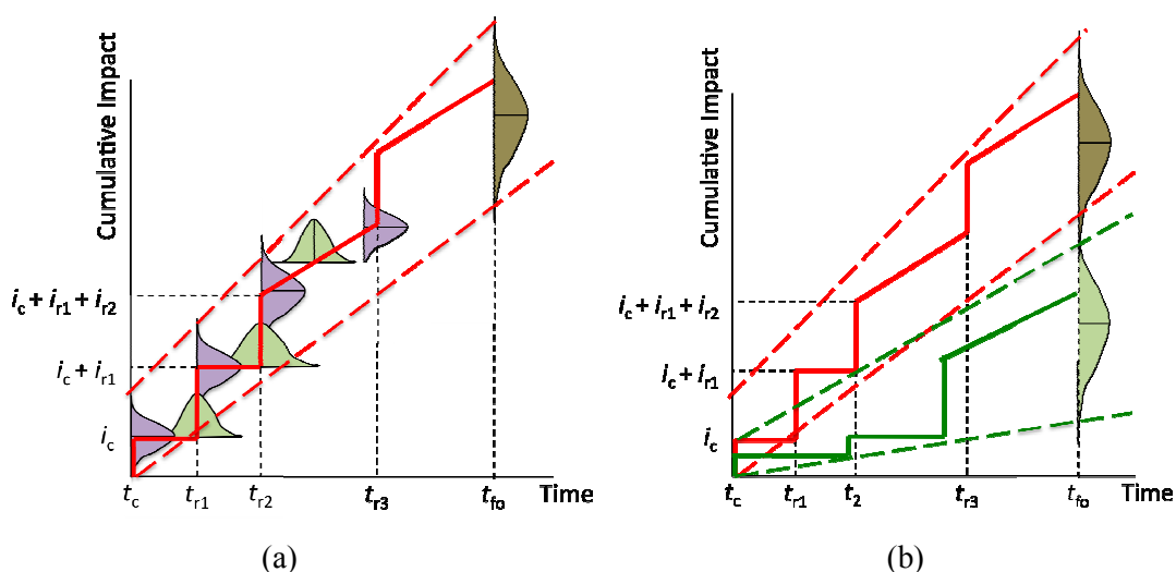
Fig. 1 (a) Cumulative sustainability impact from initial construction to functional obsolescence and (b) comparison of probabilistic envelopes for initial construction ( t_c ) to functional obsolescence ( t_{fo} ) for two alternative construction/repair technologies and associated timelines
