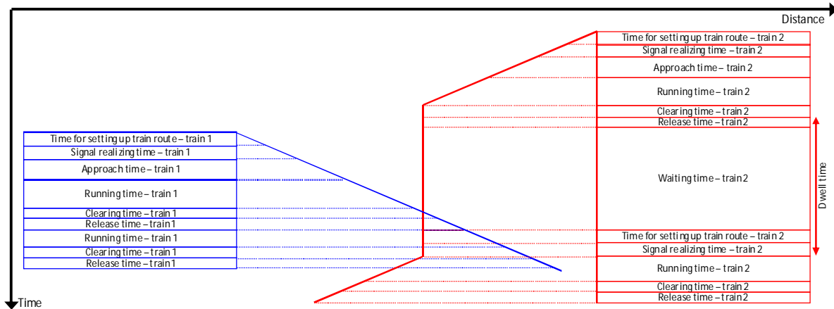
Figure5: Detailed block occupation time for tracks of a crossing station. Based on [8].
