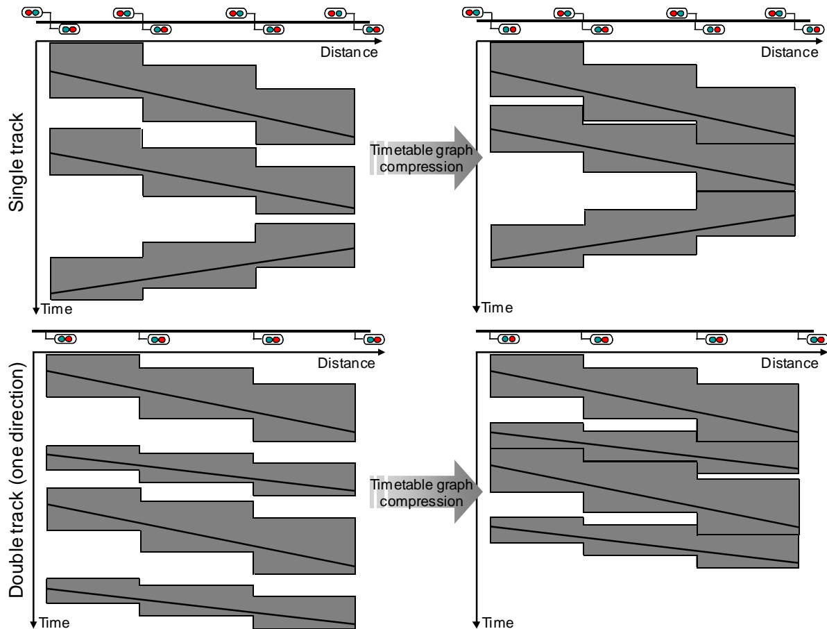
Figure 1: Compression of timetable graphs according to the UIC406 capacity method. Based on [9].
