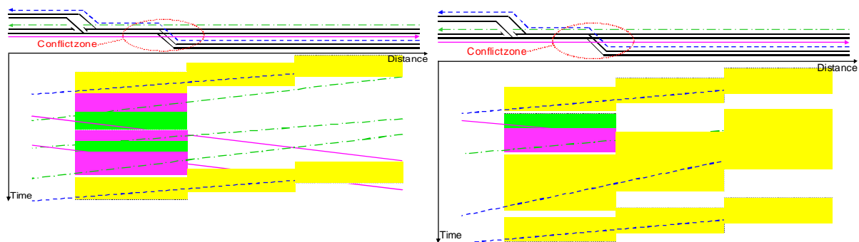
Figure 7: Capacity limitations in junction result in reduced capacity on railway line (left) and capacity in junction limited by railway lines (right).
