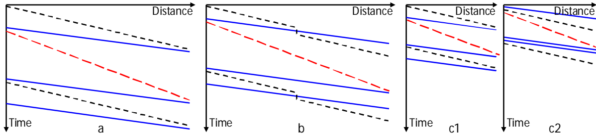
Figure 8: Capacity consumption for line section (a), line section with overtaking (b) and divided line section due to overtaking (c1 and c2)[11].
