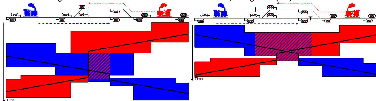
Figure 4: Crossing station without (left) and with (right) parallel movement facility [8].
