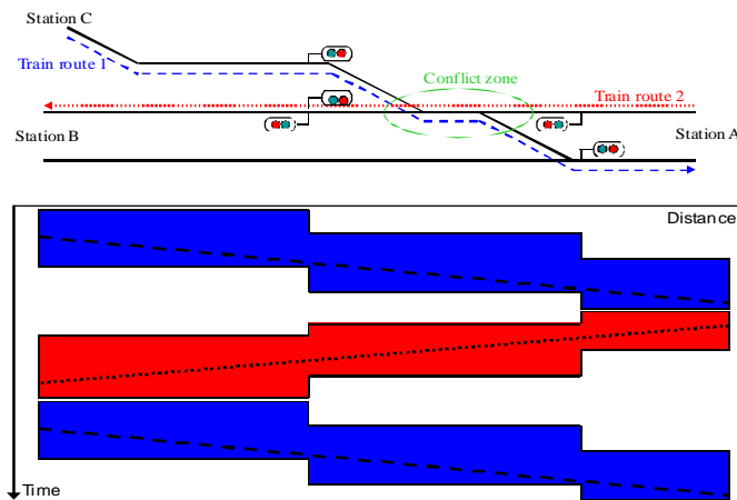
Figure 6: Capacity reduced for two trains running immediately after each other at a junction (only signals in use included). Based on [8].
