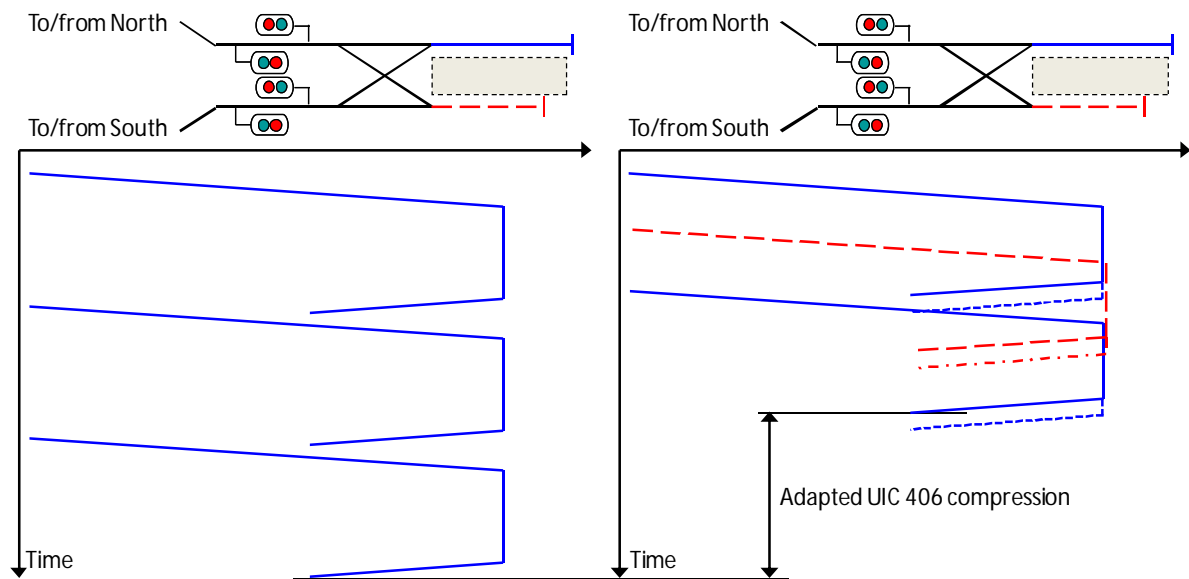
Figure 2: Adapted UIC 406 compression for stations.
