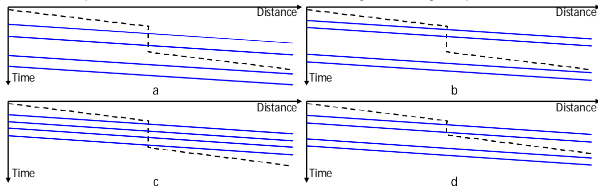
Figure 9: Timetable compression when overtaking. Based on[11].
