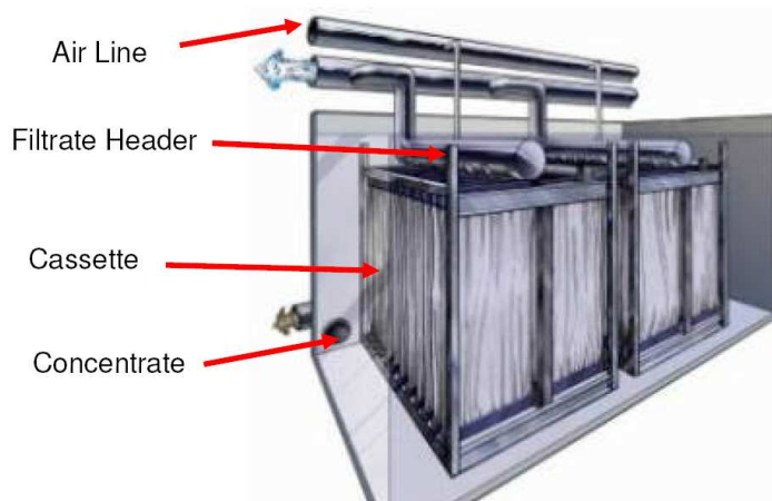
Figur 3.5. Ultrafiltreringskassetter. (Guan 2008)
