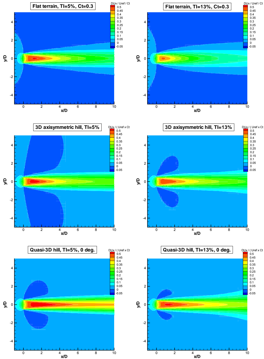
Figure 67: Comparison of wind speed deficit contours at hub height a. g. l. among flat terrain, 3D axisymmetric hill and quasi-3D hill. Tl_{in} is (a) 5% and (b) 13%.
