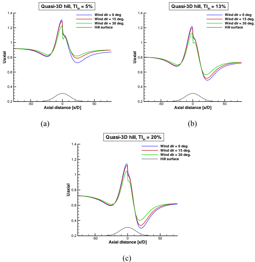
Figure 40: Variation of the streamwise wind speed at the hub height of the symmetry plane ( y = 0 ) for various wind directions and Tl_{in} values: (a) 5%, (b) 13% and (c) 20%.
