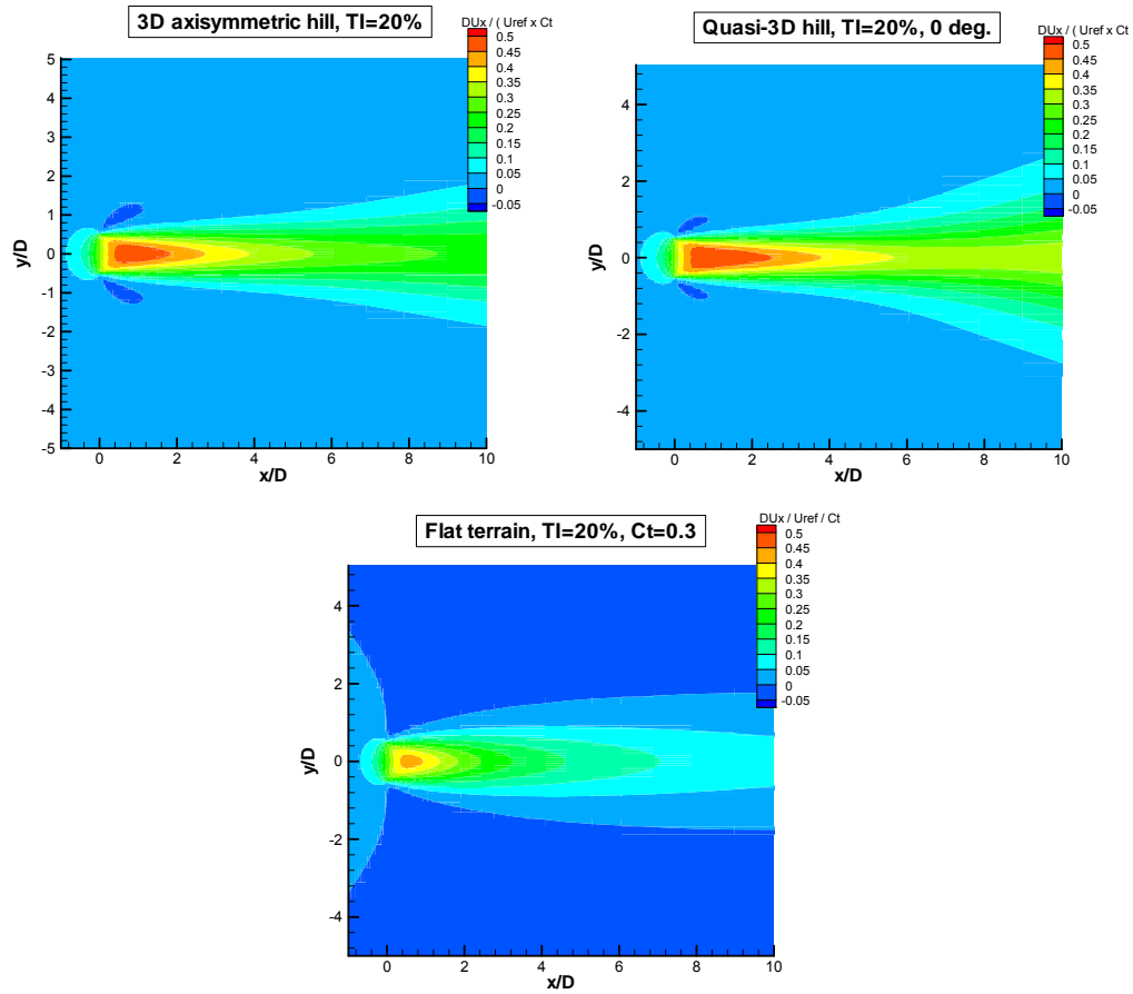
Figure 68: Comparison of wind speed deficit contours at hub height a. g. l. among flat terrain, 3D axisymmetric hill and quasi-3D hill for Tl_m = 20\% .
