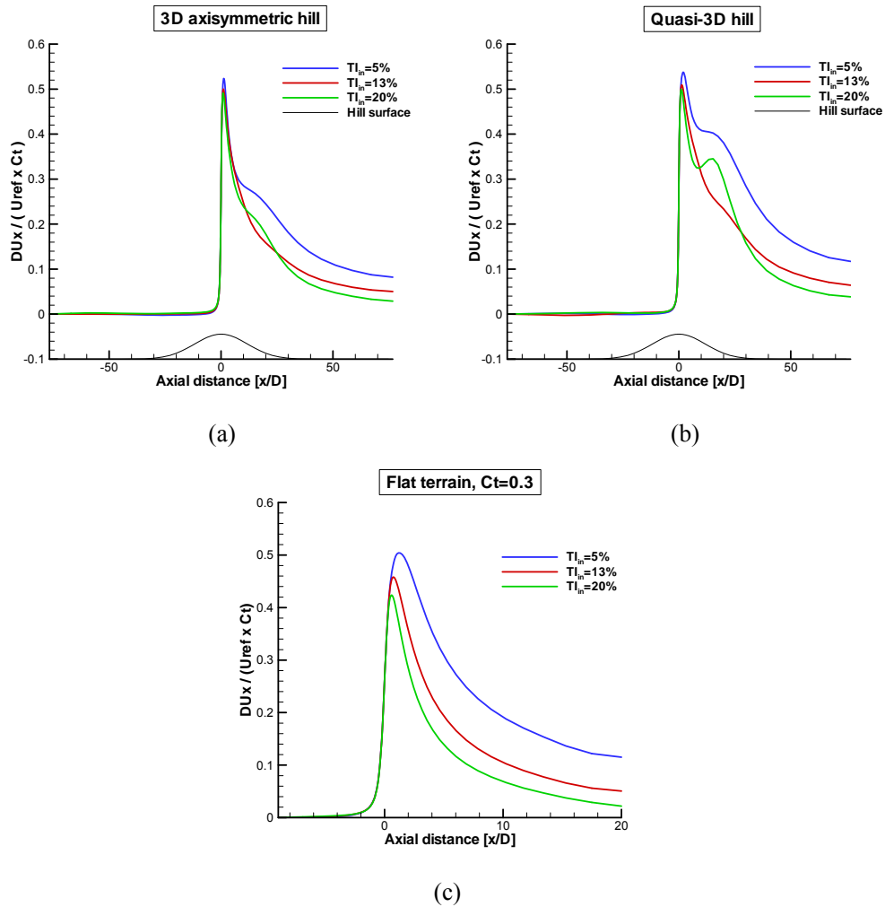
Figure 54: Wind speed deficit along y = 0 line at hub height a. g. l. for various values of Tl_{in} . (a) axisymmetric hill, (b) quasi-3D and (c) flat terrain. Wind direction is 0^\circ .
