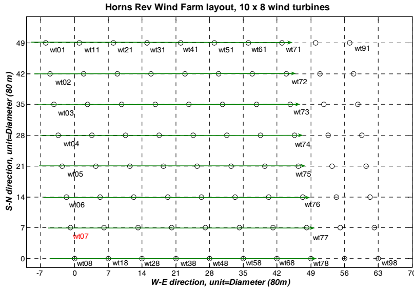
Figure 129: Horns Rev offshore wind farm, with an indication of 270° flow direction along the rows of wind turbines. The reference turbine for this flow analysis is wt07.
