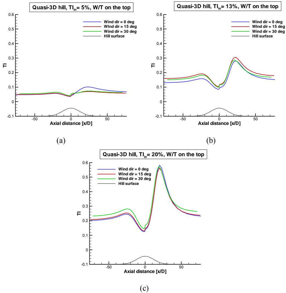
Figure 42: Variation of the turbulence intensity at the hub height of the symmetry plane ( y = 0 ) for various wind directions and Tl_{in} values: (a) 5%, (b) 13% and (c) 20%.
