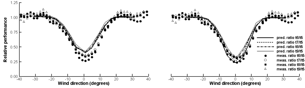
(a) (b) Figure 8. Predicted relative performances for the ECN test farm with 5 W/Ts in a row. (a) Baseline calculations (b) Calculations including Masson's correction with C=3 . 0^\circ correspond to the direction of the W/T's row. Measurements are taken from Machielse et al (2007)
