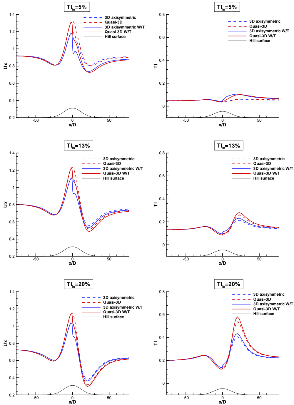
Figure 43: Comparison of the streamwise wind speed and turbulence intensity variation at the hub height of the symmetry plane ( y = 0 ) for the axi-symmetric and quasi-3D hills with and without W/T. Upper: Tl_{in} = 5\% . Middle: Tl_{in} = 13\% . Lower: Tl_{in} = 20\% .
