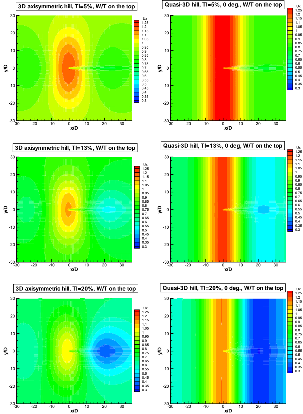
Figure 51: Streamwise wind speed contours for the axisymmetric and quasi-3D hill at hub height a. g. l. Upper: T_{in} = 5\% . Middle: T_{in} = 13\% . Lower: T_{in} = 20\% .
