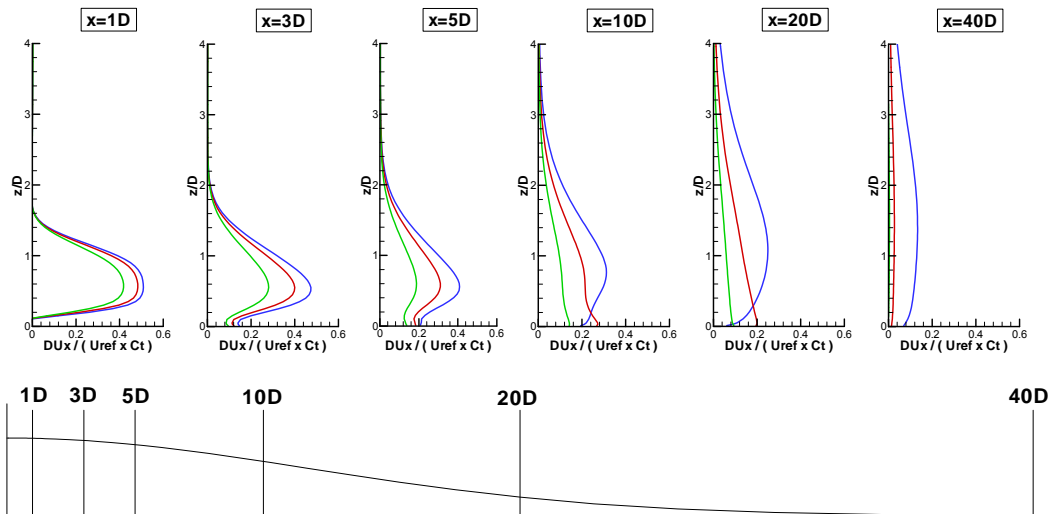
Figure 61: Quasi-3D hill – Vertical profiles of wind speed deficit downstream the hill top in the presence of W/T for various wind directions: — 0^\circ , — 15^\circ , — 30^\circ . T_{in} = 13\% .
