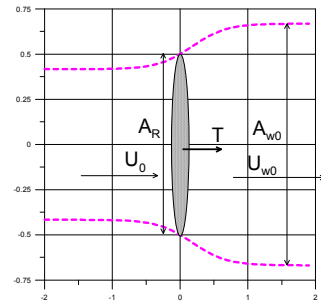
Figure 84. Near range flow around the rotor.
