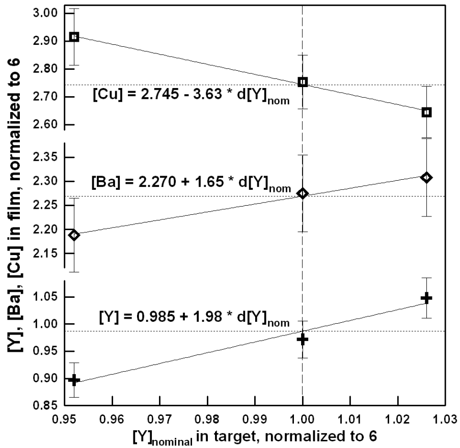
Fig. 1. Contents of cations in the YBCO film measured with ICP technique for varying yttrium contents in target.
