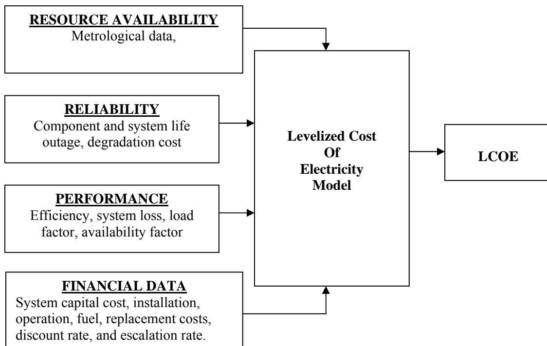
Figure 1: LCOE Model
