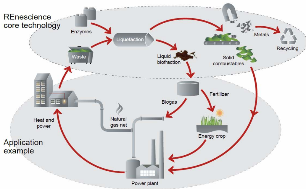
Figure 5: Concept for a sustainable household waste cycle - as demonstrated at the REnescience plant at Amagerforbrændingen waste plant in Copenhagen
