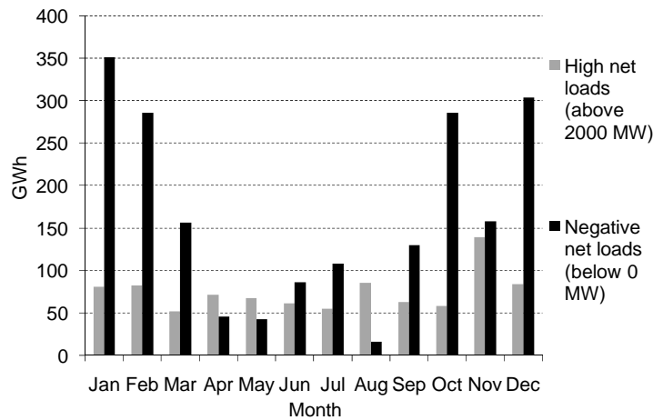
Fig. 10. Monthly distribution of negative net loads and high net loads (above 2500 MW) for West Denmark in 2025.
