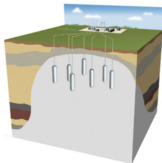
Figure 1: Figure 1: The 7 gas caverns in Ll. Torup (Energinet)
