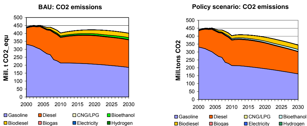
Figure 11a. CO 2 emissions in BAU-Scenario
