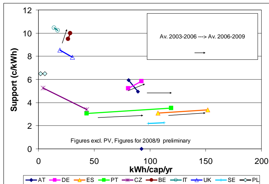
Figure 10. Effectiveness vs costs of promotion programmes for electricity from RES in selected countries 2003-2009 without PV and large hydro power (Source: own investigations)
