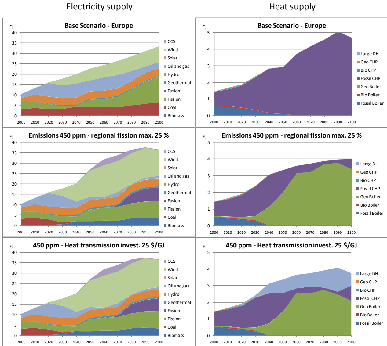
Figure 4. EFDA-TIMES results for electricity and heat supply in Europe 2000-2100. Base Scenario and two scenarios with emission constraints.
