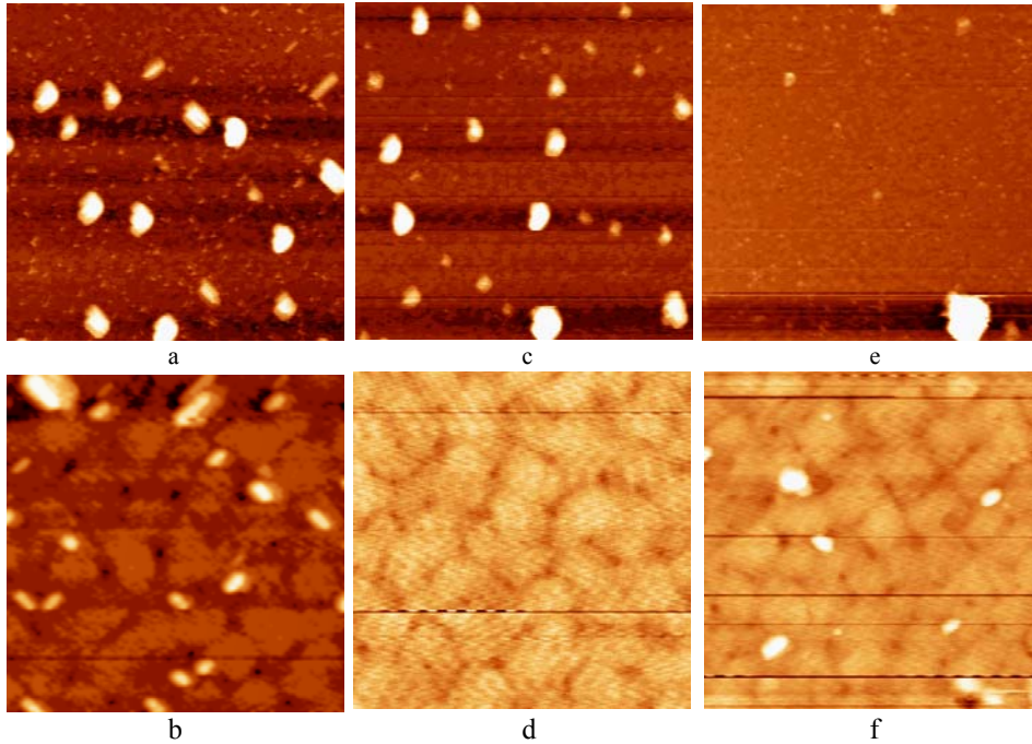
Fig. 7. AFM micrographs of YBCO films from stoichiometric target on different yttria layers. a, b - uniform yttria seeding layer; c, d - template yttria layer of nanoparticles; e, f - bare LSAT substrate. Scan size: a, c, e - 10 \times 10 \mu\text{m}^2 , b, d, f - 2 \times 2 \mu\text{m}^2 . Vertical scale 100 nm.
