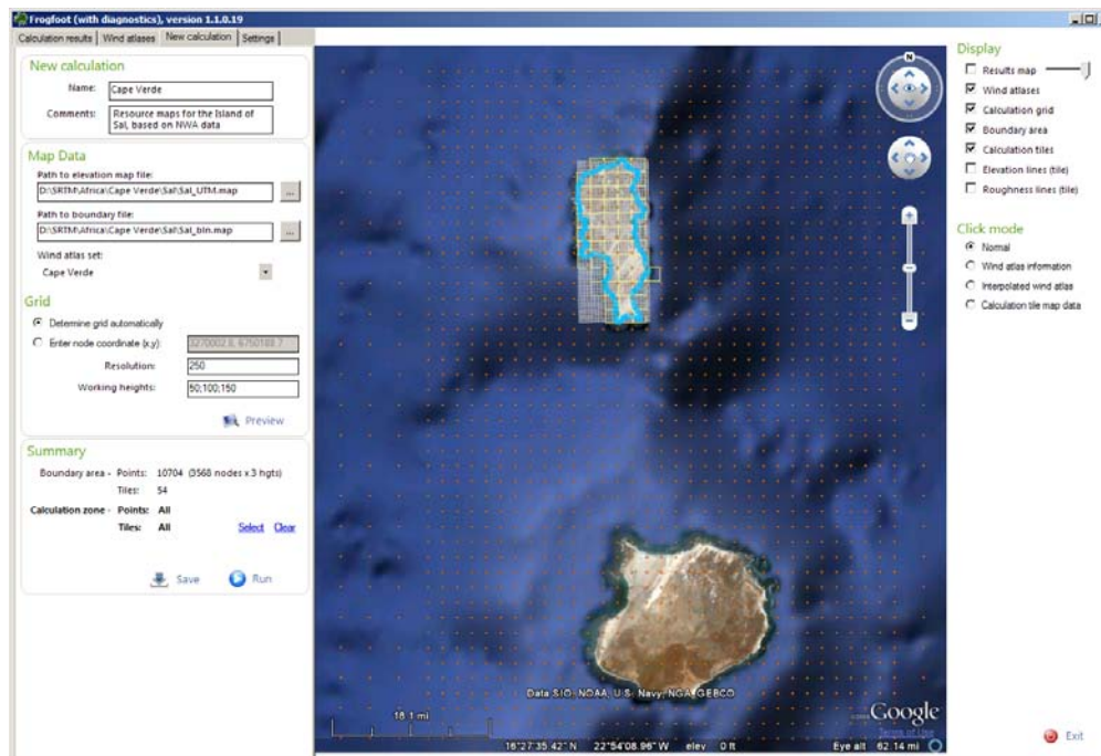
Figure 1: Cape Verde numerical wind atlas (NWA) in FROGFOOT. Each orange dot represents a data point with details sectorwise generalized wind climates statistics. FROGFOOT allows wind resources at high resolution to be calculated in WAsP using the coarser grid of generalized wind climate data points. Only part of Cape Verde is show here
