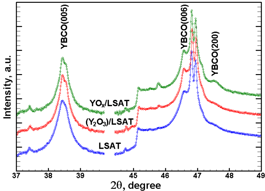
Fig. 8. Fragments of XRD \theta/2\theta -scans of the YBCO films on LSAT (100) substrates with different yttria decoration.
