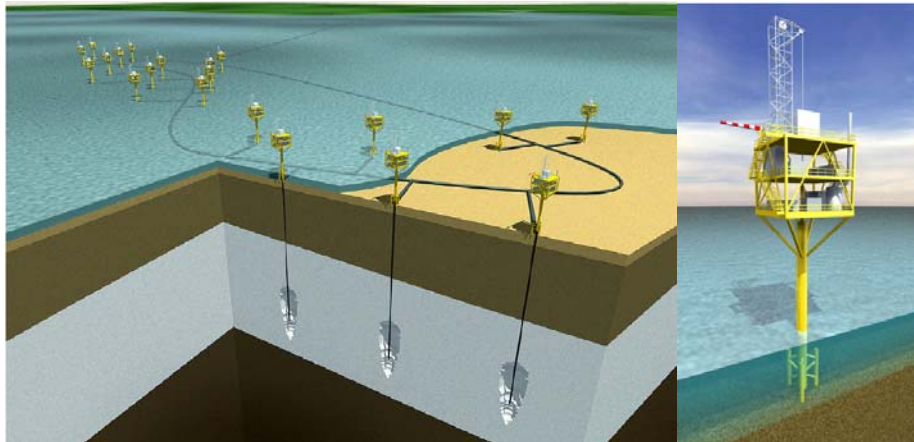
Figure 2: Planned offshore gas caverns in the Irish Sea (left), monopod for an offshore gas cavern (right). Stacey, 2008.
