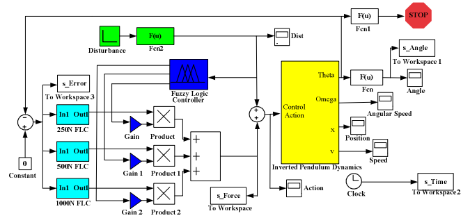
Figure 12: SIMULINK Model of a Double-Level FLC
