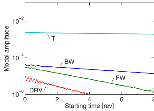
Fig. 17 Modal amplitudes from MWA for signal u_r
