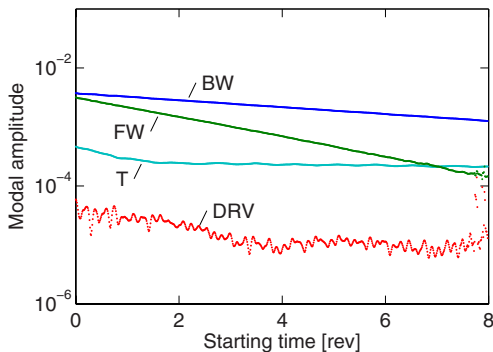
Fig. 16 Modal amplitudes from MWA for signal u_{a1}
