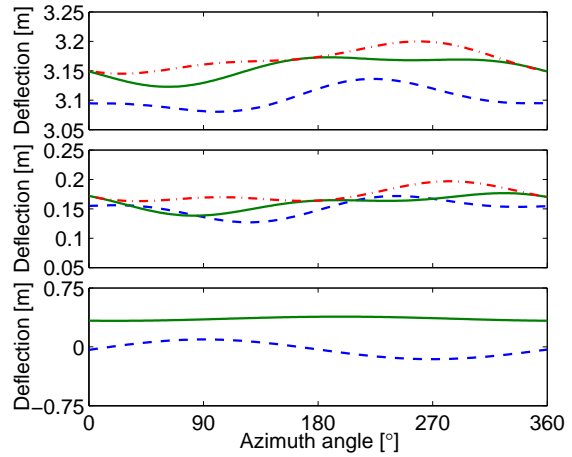
Figure 6: Steady state over one rotor period for the anisotropic rotor at 16 rpm. Blade tips flapwise (top) - - 1, — 2 and - · - 3 and edgewise (middle) - - 1, — 2 and - · - 3, and blade tips, tower top (bottom) — longitudinal and - - lateral.
