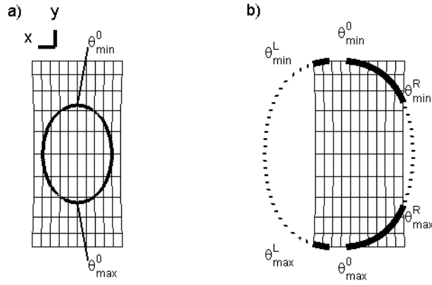
FIG. 4. Figure showing a sphere's crossing with a transducer (solid) and virtual crossings (dotted). View seen from the transducer back side in direction of the z-axis. a) The sphere has not yet crossed the side edges. The point is centered at x_p = 0 , which gives symmetry. b) The sphere has crossed the edges. Dotted lines indicate the virtual arc crossings. The point is offset to the left, which makes the left virtual arc significant bigger than the right virtual arc. See an illustration of the angles being created by the crossing in the video: "AngleVideo" found on the attached CD.
