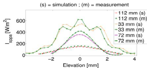
Fig.4 Comparison between measured and simulated spatial peak pulse average intensity
