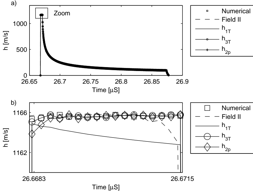
FIG. 10. Results of simulating a convex non-elevation focused array.
