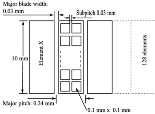
Fig.1 A frontal view of the transducer elements.
