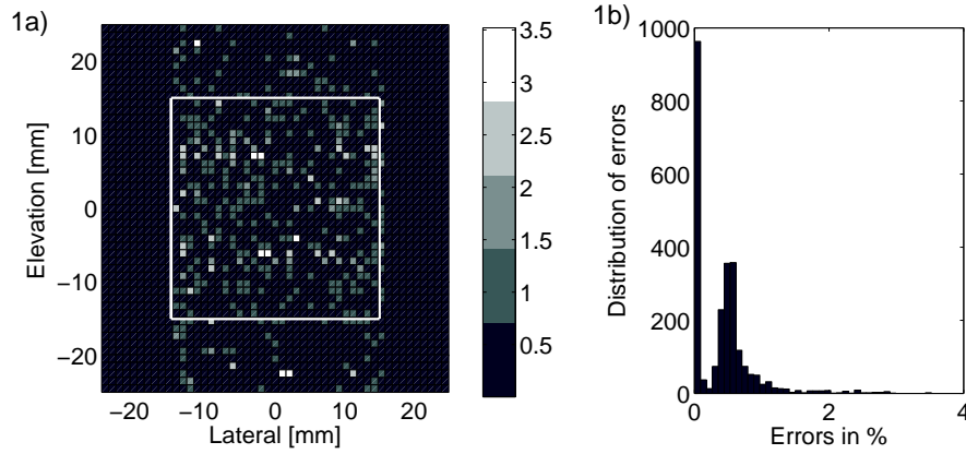
Figure 2.10: 1a) The RMS error for 2500 points, projected down onto the xy -plane. The white square indicates the outer boundary of the transducer. 1b) Distribution of the errors. Figure taken from Paper I.
