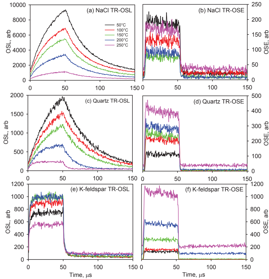
Figure 5.4: Time-resolved OSL and OSE from NaCl (a, b), quartz (c, d), and K-feldspar (e,f) for stimulation temperatures of 50, 100, 150, 200 and 250°C following doses of 200, 200, and 500 Gy respectively and a preheat to 280°C using pulsed LED stimulation (on-time: 50 μs, off-time: 100 μs). Doses and preheat similar to those of Fig. 5.3.
