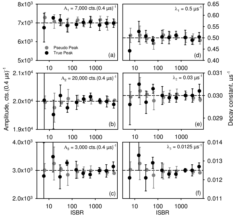
Figure 3.8: Results from fitting pseudo LM-OSL data (grey filled circles) and ‘true’ LM-OSL data (filled black circles) using the NLS method. In each plot the dashed line indicates the known parameter value, and each point is the average over five parameter values for the same ISBR. The left column shows the results for the amplitudes (a) A_1 = 7000 cts/( 0.4 \mu\text{s} ) ^{-1} , (b) A_2 = 20000 cts/( 0.4 \mu\text{s} ) ^{-1} , and (c) A_3 = 3000 cts/( 0.4 \mu\text{s} ) ^{-1} . The right column shows the results for the decay parameters (d) \lambda_1 = 0.5 \mu\text{s}^{-1} , (e) \lambda_2 = 0.03 \mu\text{s}^{-1} , and (f) \lambda_3 = 0.0125 \mu\text{s}^{-1} .
