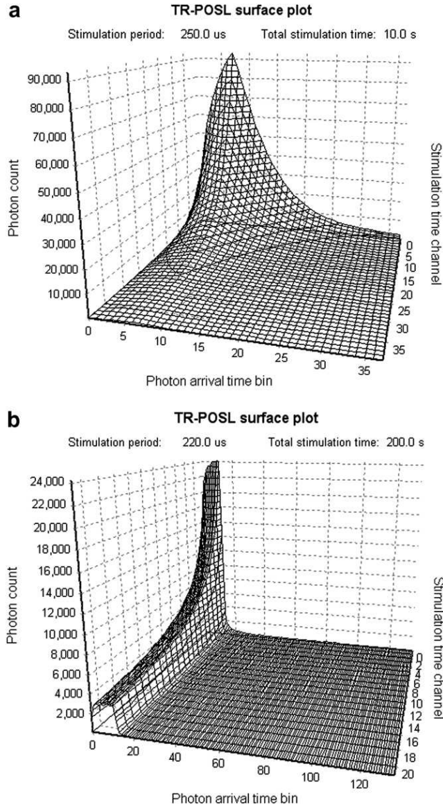
Figure 2.3: (a) PTanalyse TR-POSL surface plot of a quartz sample with on-/off-time of 50/200 \mu s. Bin width: 0.1 \text{ ns} \times 2^{16} = 6.55 \mu s, channel width: 1000 pulse periods = 250 ms, irradiation: 10 Gy, preheat at 260°C, blue LED stimulation at 125 °C. (b) PTanalyse TR-POSL surface plot of an orthoclase feldspar sample with on-/off-time of 20/200 \mu s. Bin width: 0.1 \text{ ns} \times 2^{14} = 1.64 \mu s, channel width: 40,000 pulse periods = 8.80 s, irradiation: 500 Gy, preheat at 250°C, blue LED stimulation at 50°C.
