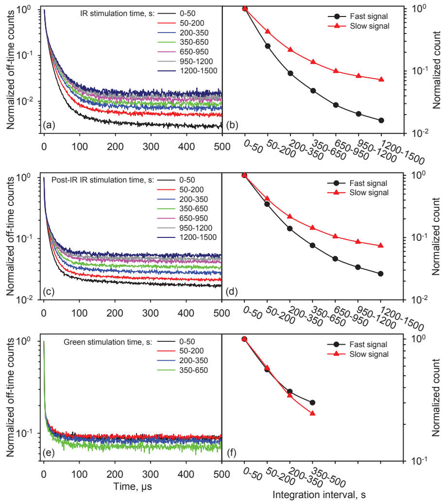
Figure 9.8: Stimulation time dependence of the TR-IRSL, post-IR TR-IRSL, and TR-GLSL off-time decay curves from orthoclase feldspar normalized to the last point in the on-time. The sample was preheated to 250°C for 60 s following a dose of 45 Gy (IR signals) or 100 Gy (green signal). The TR-IRSL signal was measured at 50°C for 1500 s, the post IR (at 50°C for 100 s) TR-IRSL signal was measured at 225°C for 1500 s, and the TR-GLSL was measured at 50°C for 500 s. The stimulation pulses produced during the stimulation time intervals given in the figures were added up to produce the normalized off-time curves shown on the left hand side; the legends show the stimulation time intervals during which the TR-OSL signals were added to produce these curves. The summary curves on the right hand side show the normalized behaviour of the fast (circles) and slow (triangles) signals of the time-resolved curves. Each point in the summary was normalized to the duration of the stimulation time interval, as these are of unequal length, so as to be able to compare the data. The data were then further normalised to the first point on the plots. All open symbols denote recycling points. (a) TR-IRSL off-time curves, (b) summary of the TR-IRSL curves, (c) post-IR TR-IRSL off-time curves, (d) summary of the post-IR TR-IRSL curves, (e) TR-GLSL off-time curves, and (f) summary of the TR-GLSL curves. Note that the integration intervals for the green stimulation are not identical to those of the IR stimulations.
