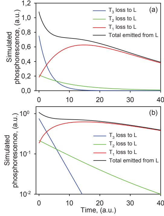
Figure 6.10: (a) Curves showing the loss from T_3 , T_2 , and T_1 together with the phosphorescence emitted at L when solving the rate-equations (6.1)-(6.4) using the parameters: n_{10} = 50 \text{ cm}^{-3} , \lambda_1 = 0.04 \text{ s}^{-1} , n_{20} = 300 \text{ cm}^{-3} , \lambda_2 = 0.09 \text{ s}^{-1} , n_{30} = 25 \text{ cm}^{-3} , \lambda_3 = 0.3 \text{ s}^{-1} , f_3 = 0.1 , and f_2 = 0.92 . (b) The same curves from (a) shown on a semi-log scale.
