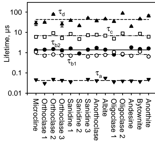
Figure 7.2: Lifetimes calculated for signals obtained with pulsed 532 nm laser stimulation ( \tau_a and \tau_{b_1} ) and pulsed (on-time 10 \mu\text{s} , off-time 200 \mu\text{s} ) 470 nm LED stimulation ( \tau_{b_2} , \tau_c , \tau_d ) for each of the 14 samples. The horizontal lines represent the average component lifetimes. The given doses were between 5 Gy and 1000 Gy depending on individual sample sensitivity. Heating conditions were identical to those in Fig. 7.1.
