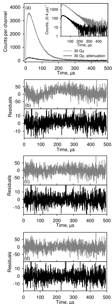
Figure 3.9: TR-OSL data measured from a colluvium quartz sample from Tanzania. The sample was given a dose of 30 Gy and was heated to 260^\circ\text{C} for 10 s prior to blue LED stimulation at 125^\circ\text{C} for 22 s. The on-time was 50 \mu\text{s} and the off-time was 500 \mu\text{s} . Prior to fitting, the data was transformed into a peak shape using Eqn. (3.7) (grey curve). The experiment was then repeated, but with a neutral density filter inserted beneath the PMT to attenuate the incoming light from the sample (black curve) by a factor of 16. The inset shows the curves on log-scale. (b) Residual curves for a one-component fit of the 30 Gy data (grey curve) and the attenuated 30 Gy data (black curve) using the NLS method, (c) residual curves for a two-component fit of the two data sets, and (d) residual curves for a three-component fit of the curves for the same notation as in (b).
