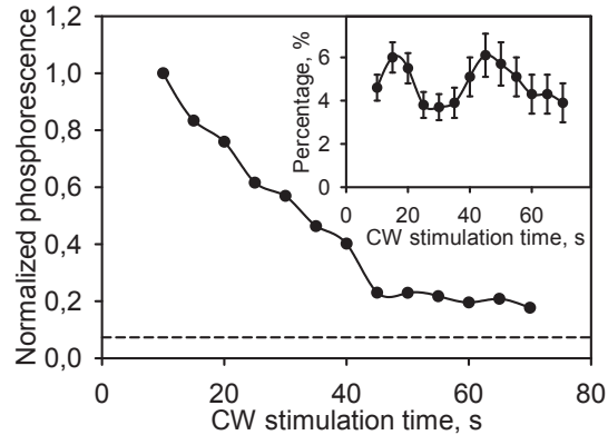
Figure 6.12: Normalized cumulative phosphorescence (integrated over 10 s) following different lengths of CW stimulations in the range of 10 s to 70 s. The sample was dosed with 25 Gy, preheated to 260°C for 10 s and stimulated at 125°C. The dashed line indicates the dark count level also integrated over 10 s. Inset: The percentage ratio between the end point of the OSL curve and the first point in the phosphorescence signal given for different CW stimulation times.
