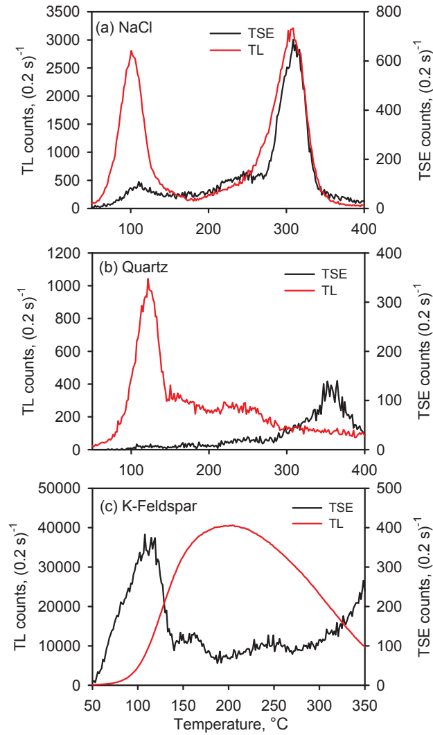
Figure 5.2: TL and TSE curves from (a) NaCl, (b) quartz and (c) K-feldspar, using doses of 100, 1000, and 1000 Gy respectively.
