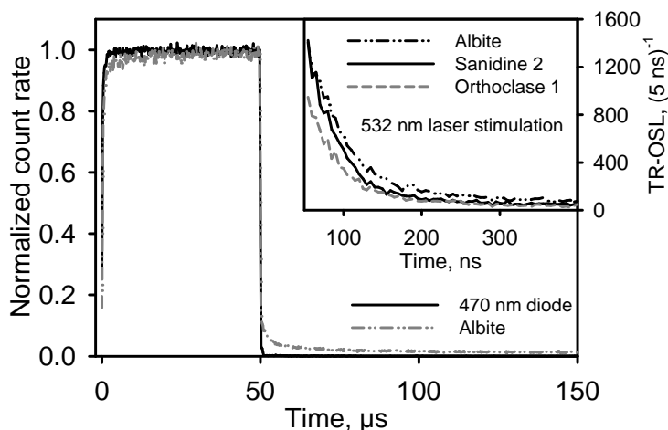
Figure 7.1: The stimulation pulse shape from the 470 nm LEDs plotted together with the OSL signal from Albite, both normalized to the 50 \mu\text{s} point. The Albite was given a dose of 5 Gy, preheated to 250°C for 60 s and stimulated at 50°C. Inset: Albite, Sanidine 2 and Orthoclase 1 TR-OSL signals obtained just after the 15 ns stimulation pulse width from the pulsed 532 nm laser. Note that the initial 55 ns have been removed from the data. Doses were 5, 500, and 5 Gy respectively, and the samples were preheated to 250°C for 60 s and stimulated at room temperature.
