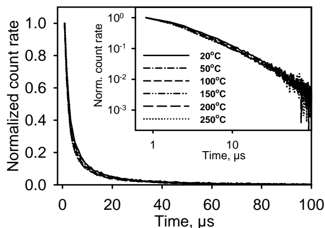
Figure 7.3: Initial-intensity-normalized TR-OSL signals measured (after stimulation) at temperatures of 20°C, and 50°C to 250°C in steps of 50°C for Sanidine 2 using on-time 20 μs and off-time 200 μs. The signal backgrounds were subtracted prior to normalization. The inset shows the curves on log-log scale. The sample was given a dose of 500 Gy prior to a preheat of 250°C for 60 s.
