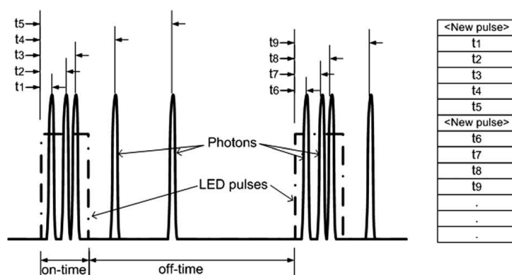
Figure 2.1: Diagram showing the principle of Photon Timer data recording. The list to the right illustrates the sequential listing of events.
