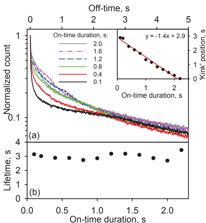
Figure 8.8: (a) Post-IR IRSP curves for different stimulation pulse durations. An aliquot of orthoclase was dosed with 200 Gy, preheated to 300°C for 60 s, IR bleached at 50°C for 100 s and then IR stimulated again at 240°C with a single pulse of length varying between 0.1 s and 2.2 s. The curves have been normalized to the intensity of the initial off-time data, and only the first 5 s of the off-time data is shown. Inset: changes in the position of the kink (sudden change in the decay rate) as a function of stimulation pulse duration. The data have been fitted to a straight line. (b) Lifetimes found from exponential fitting of the portion of the off-time curve after the 'kink' after subtraction of the average constant background estimated using the last 20 points in the off-time.
