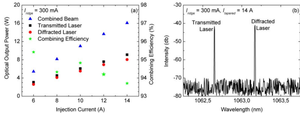
Fig. 4. (a) Output power of the individual lasers and the combined beam at 300 mA to the ridge section and different injection currents to the tapered section. The angles of incidence and the laser temperatures are adjusted for maximum diffraction and transmission at each current value. Star symbols indicate the corresponding combining efficiency achieved at each current. (b) Optical spectrum of the combined output beam at 14 A to the tapered section.
