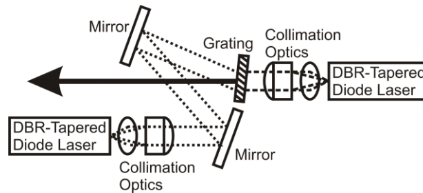
Fig. 1. Sketch of the spectral beam combining setup based on two DBR-tapered diode lasers and a reflecting volume Bragg grating. The beam transmitting the grating is indicated by dashes, the diffracted beam by dots. The arrow signifies the propagation of the combined beam.
