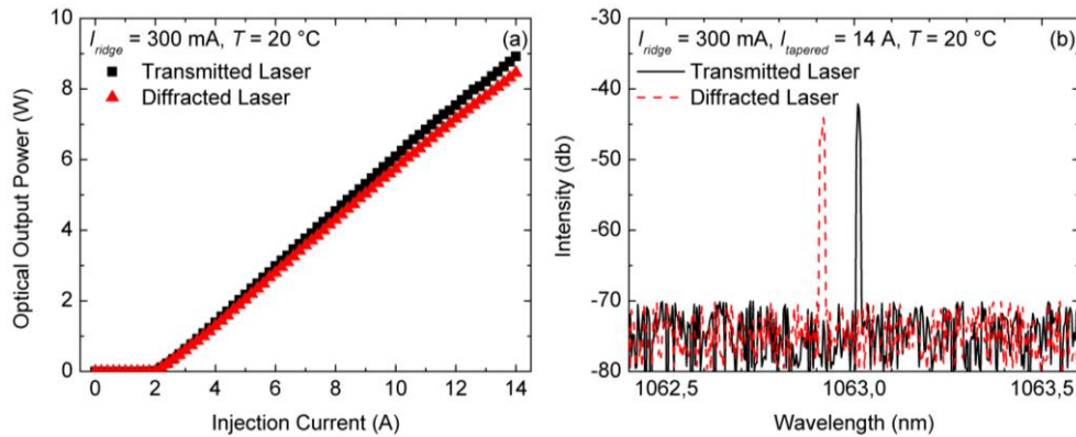
Fig. 2. (a) Power current characteristics of DBR-tapered diode lasers at 300 mA to the ridge section and operating temperatures of 20 °C. (b) Optical spectra of the lasers at 14 A to the tapered section.
