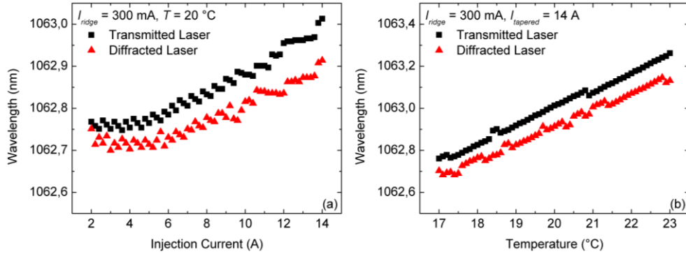
Fig. 3. (a) Wavelength versus injection current of DBR-tapered diode lasers at 300 mA to the ridge section and operating temperatures of 20 °C. (b) Wavelength versus temperature of the lasers at 14 A to the tapered section.
