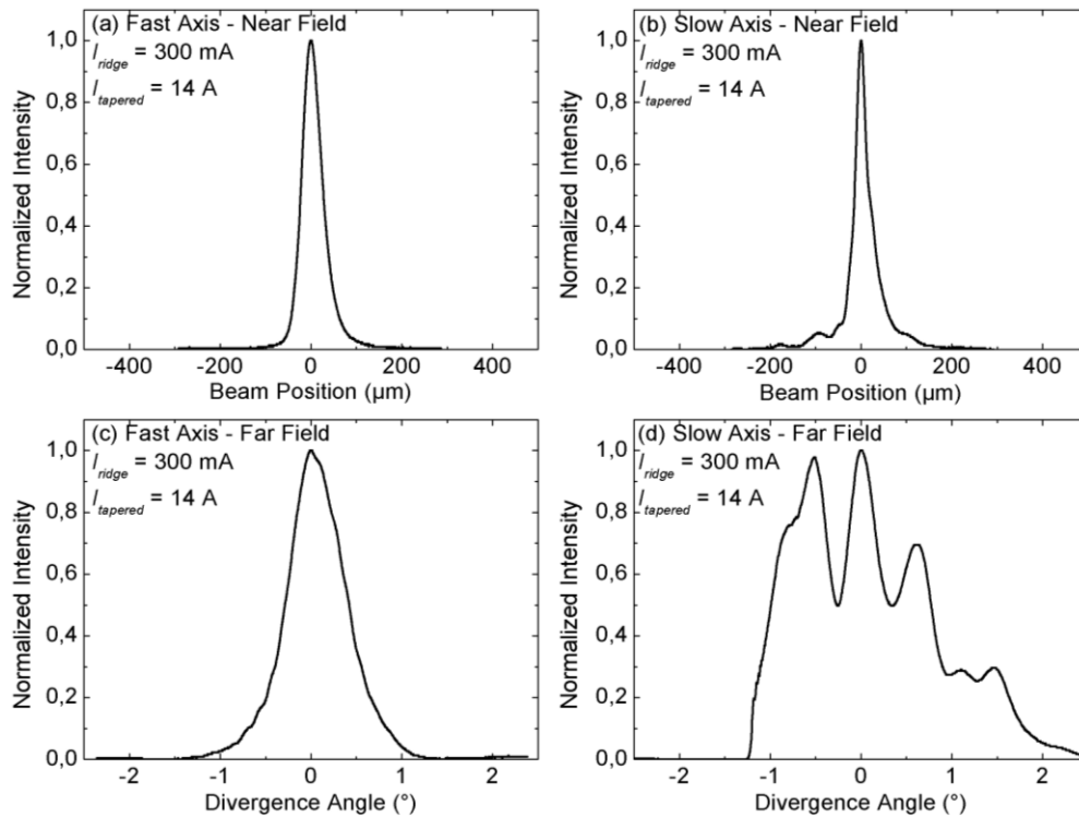
Fig. 6. Beam profiles of the combined beam at 300 mA to the ridge section and 14 A to the tapered section. (a) Near field profile in the fast axis. (b) Near field profile in the slow axis. (c) Far field profile in the fast axis (d) Far field profile in the slow axis.
