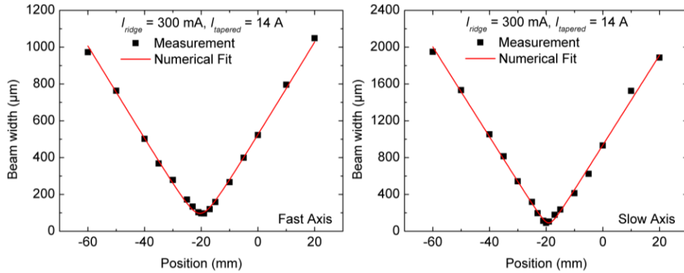
Fig. 5. Beam caustics of the combined beam at 300 mA to the ridge section and 14 A to the tapered section.
