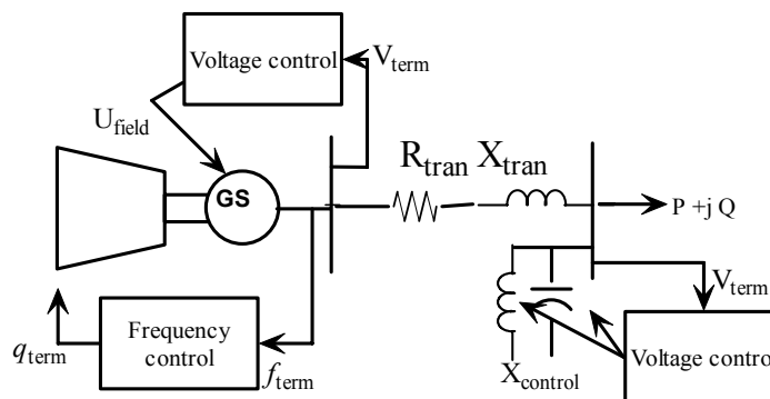
Figure 2.6 Single line equivalent of a Power System.
