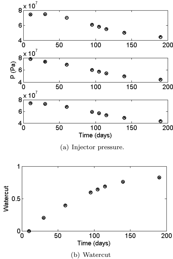
Figure 7.3: Match of injector pressures and watercut in a quarter-nine spot setup with the Levenberg-Marquardt method using Tikhonov regularization. The prior field is heterogeneous and comes from the same random process which was used to generate the reference field. \times : Reference, o : Match.
