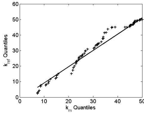
(c) qq-plot.
