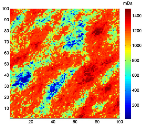
Figure 5.5: 100 \times 100 reference field generated by sequential Gaussian simulation. A trend in the North-East direction is induced by a non-isotropic variogram.
