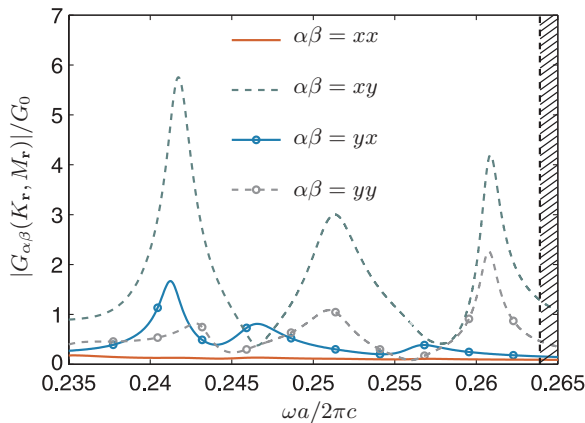
FIG. 6. (Color online) Absolute values, in units of G_0 , of elements in the propagator between the points K_r and M_r in a crystallite with side length L = 6a . Hatching indicates the in-plane band gap of the infinite crystal.
