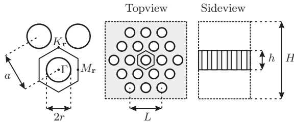
FIG. 3. Sketch of the crystallites. Of special importance are the high-symmetry points in the center and along the edge of the central Wigner-Seitz cell (hexagonal area). In this work we focus on the points \Gamma = (0,0,0) , K_r = (0, a/\sqrt{3}, 0) , and M_r = (a/2, 0, 0) .
