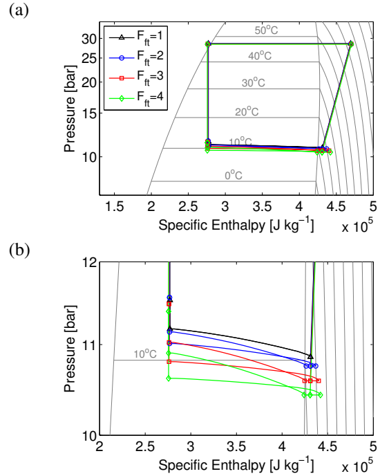
Figure 8: \log(p)h cycles at different feeder tube bending parameter
