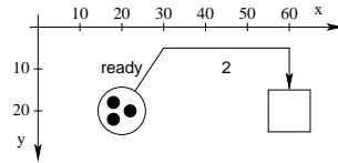
Figure 2.3: A simple P/T-System
