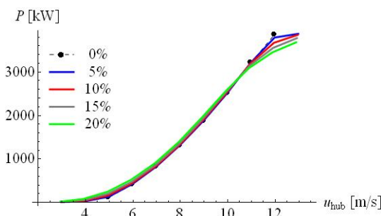
Figure 1 Mean power curves for various turbulence intensities
