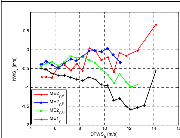
Figure 10: NWS_y (Latitude wind speed) measured at different positions versus DFWS_h (Derived free wind speed).
