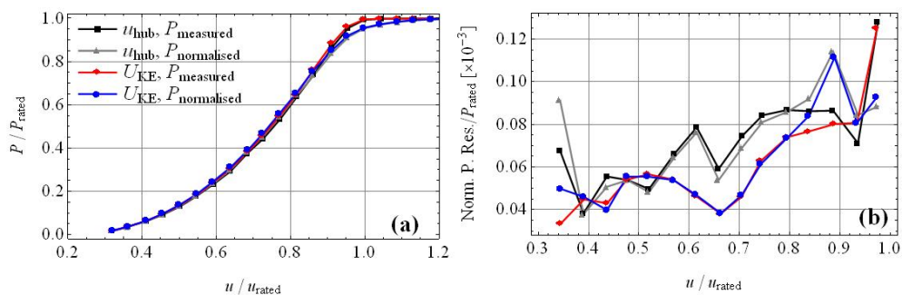
Figure 3 Mean power curve and scatter in the power curve obtained with wind speed measurements at hub height and equivalent wind speed, both with and without turbulence normalisation using Albers' method
