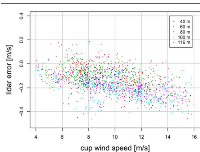
Figure 4 Lidar error versus wind speed for a Windcube WLS7 [3]
