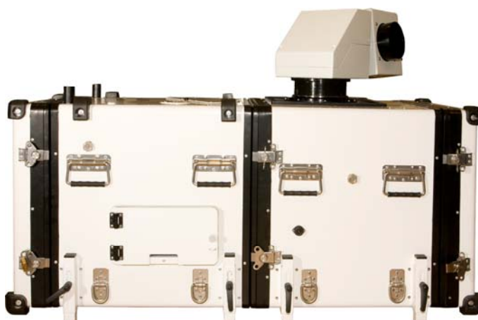
Figure 3: Long-Range WindScanner 2010
