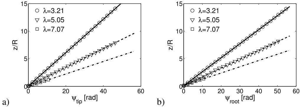
Figure 5.2: Angular positions of tip (a) and root (b) vortex cores as a function of their downstream location determined from contour plots of vorticity
