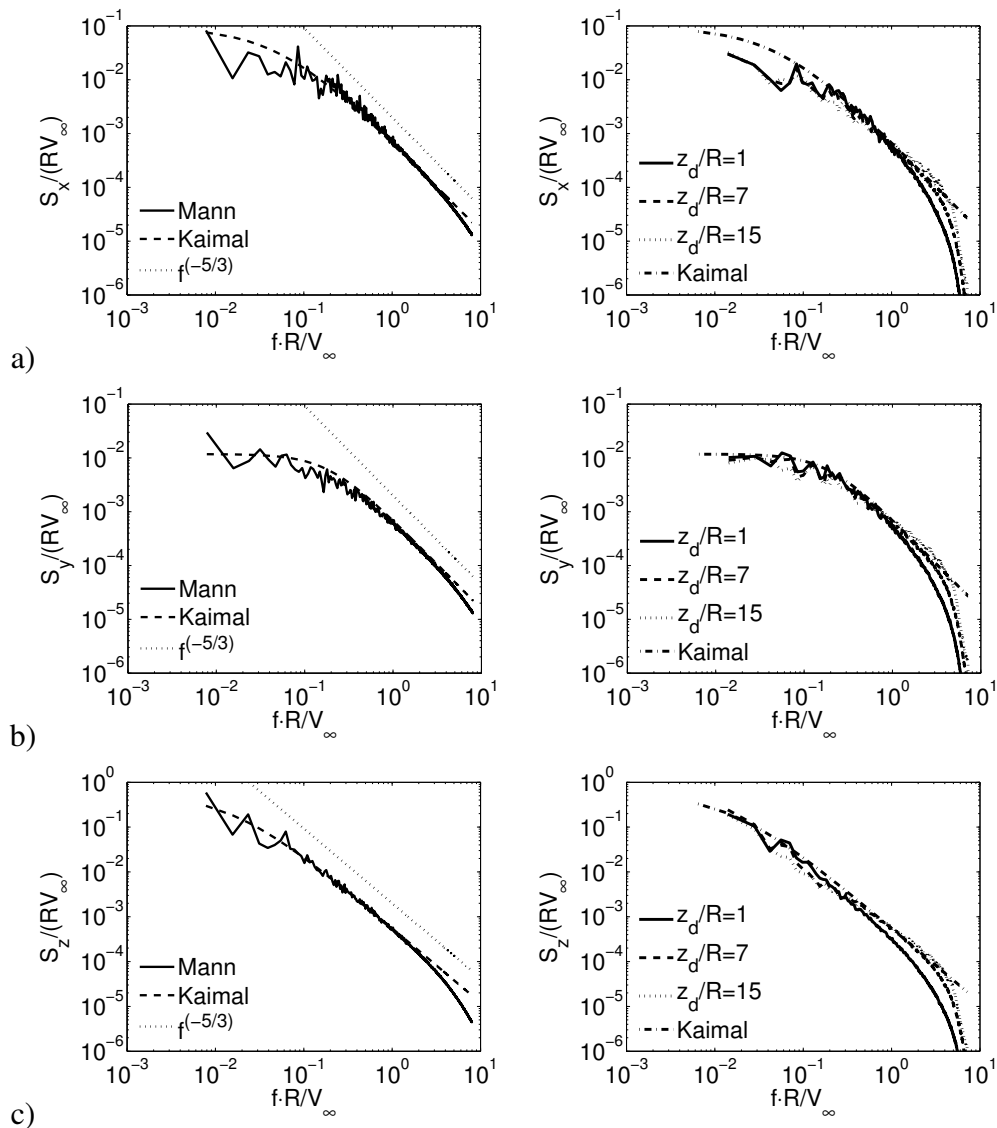
Figure 8.1: Comparison of the analytical Kaimal spectrum with the spectrum of the introduced turbulence field. Left: Initial spectra. Right: Downstream development of one dimensional spectra. a) x -velocity; b) y -velocity; c) z -velocity.
