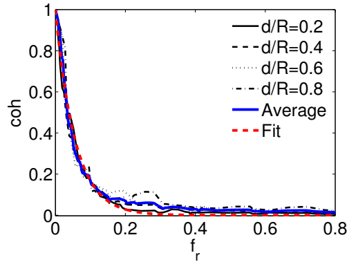
Figure A.5: Comparison of coherence functions computed for various displacements in the wake of the Tjæreborg turbine at V_\infty = 10 \text{ m/s} , r_m = 0.6 , \phi_m = 0 and z/R = 14 (see chapter 9). Also shown is the average of all curves as well as the fitted curve using equation A.17 with optimal choice of C
