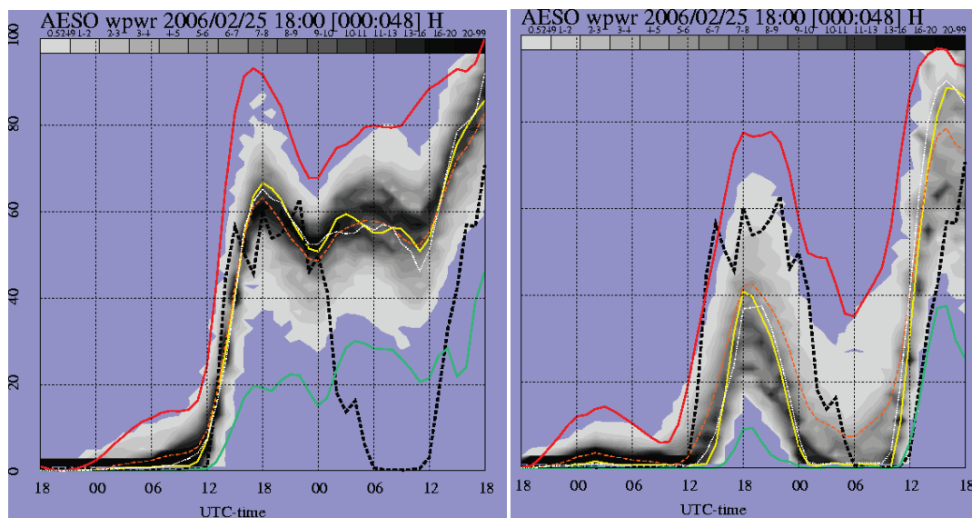
Figure 25: Measurements and calculated quantiles for 6 wind farms in Alberta, Canada. Picture from WEPROG. The measurements are the dark blue dotted line which is identical in both plots. The forecasts to the left show the large-scale model, the forecasts to the right the smaller scale model.
