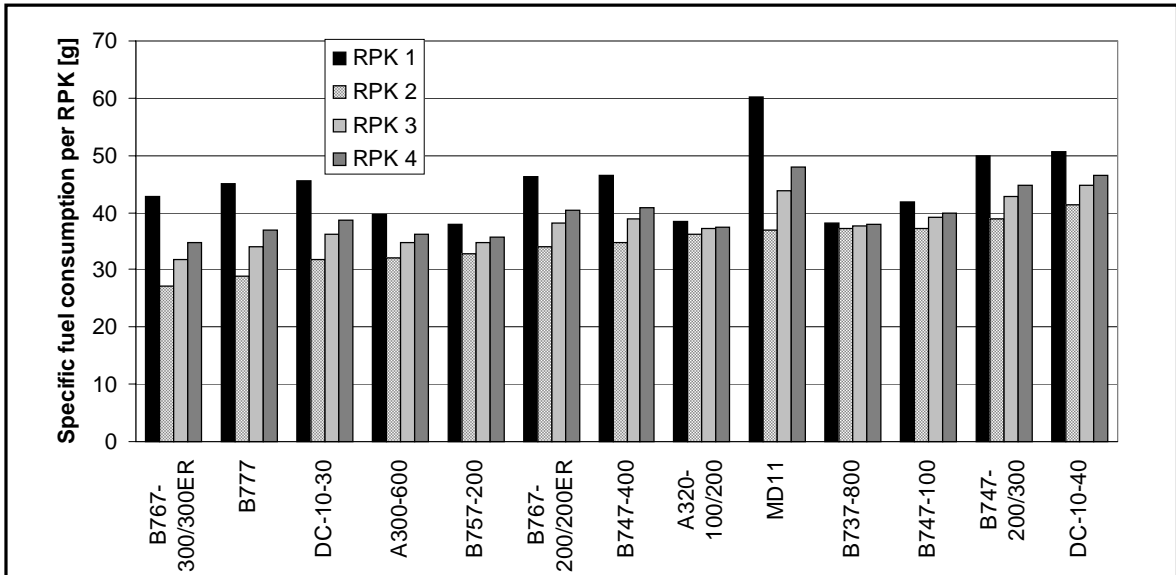
Figure 3.11: The variation in the specific fuel consumption per RPK when using four different methodologies for attributing fuel to freight
