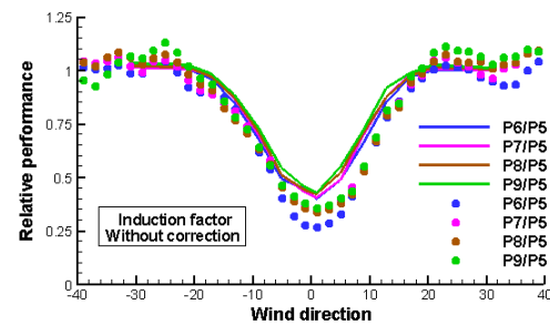
Figure 4: Relative power performances for the ECN test farm ( U=6-8\text{m/s} ). The reference velocity is defined using the induction factor concept. Lines correspond to predictions, symbols to measurements.
