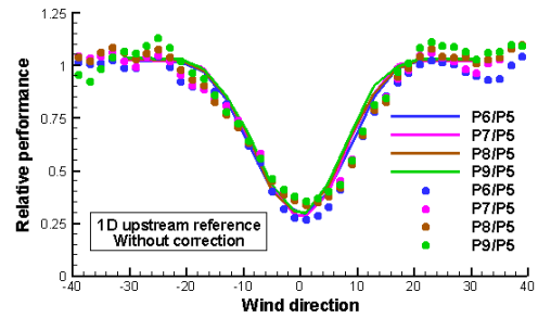
Figure 3: Relative power performances for the ECN test farm ( U=6-8\text{m/s} ). The reference wind speed is defined 1 D upstream of the rotor. Lines correspond to predictions, symbols to measurements.
