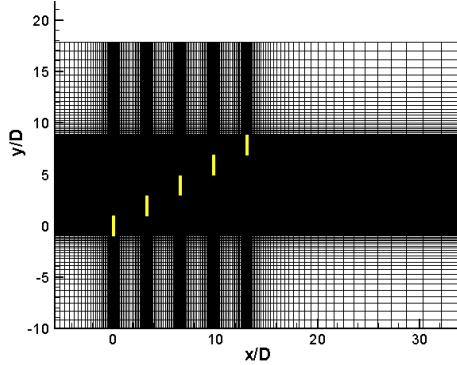
Figure 2: Two-dimensional layout of the generated grid for the simulation of the ECN test farm for 30^\circ wind direction.
