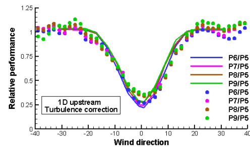
Figure 5: Relative power performances for the ECN test farm ( U=6-8\text{m/s} ). The reference wind speed is defined 1 D upstream of the rotor. Correction of the turbulence model is applied.
