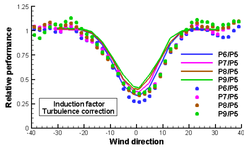
Figure 6: Relative power performances for the ECN test farm ( U=6\text{--}8\text{m/s} ). The reference wind speed is defined using the induction factor concept. Correction of the turbulence model is applied.
