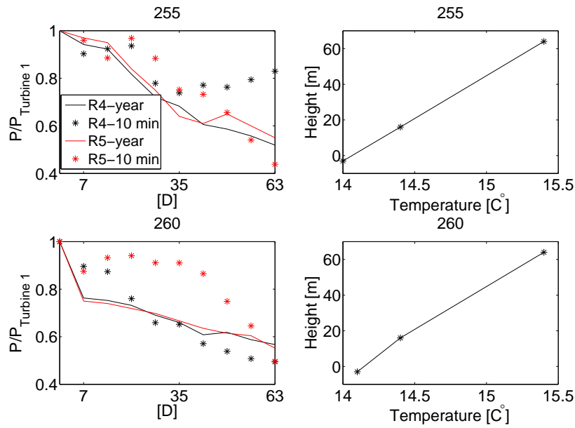
Figure 6: Experimental data from Horns Rev.
