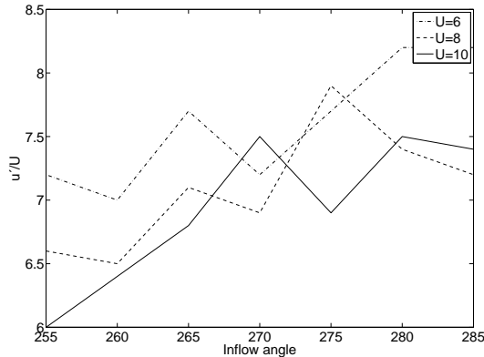
Figure 3: Measured turbulence intensity at Horns Rev wind farm at 62 m height. May 1999 to November 2002.
