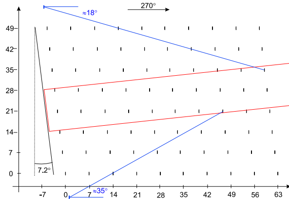
Figure 1: Layout of Horns Rev Wind Farm.
