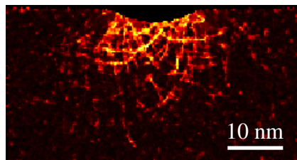
Figure 10. The shear bands are much more pronounced in a 2D simulation (using the LJ potential). The simulation shown is with an indentation rate of 7 \text{ m s}^{-1} and a cooling rate of 0.41 \text{ K ps}^{-1} . Changing the indentation rate to 0.7 \text{ m s}^{-1} does not change the pattern significantly (not shown).
