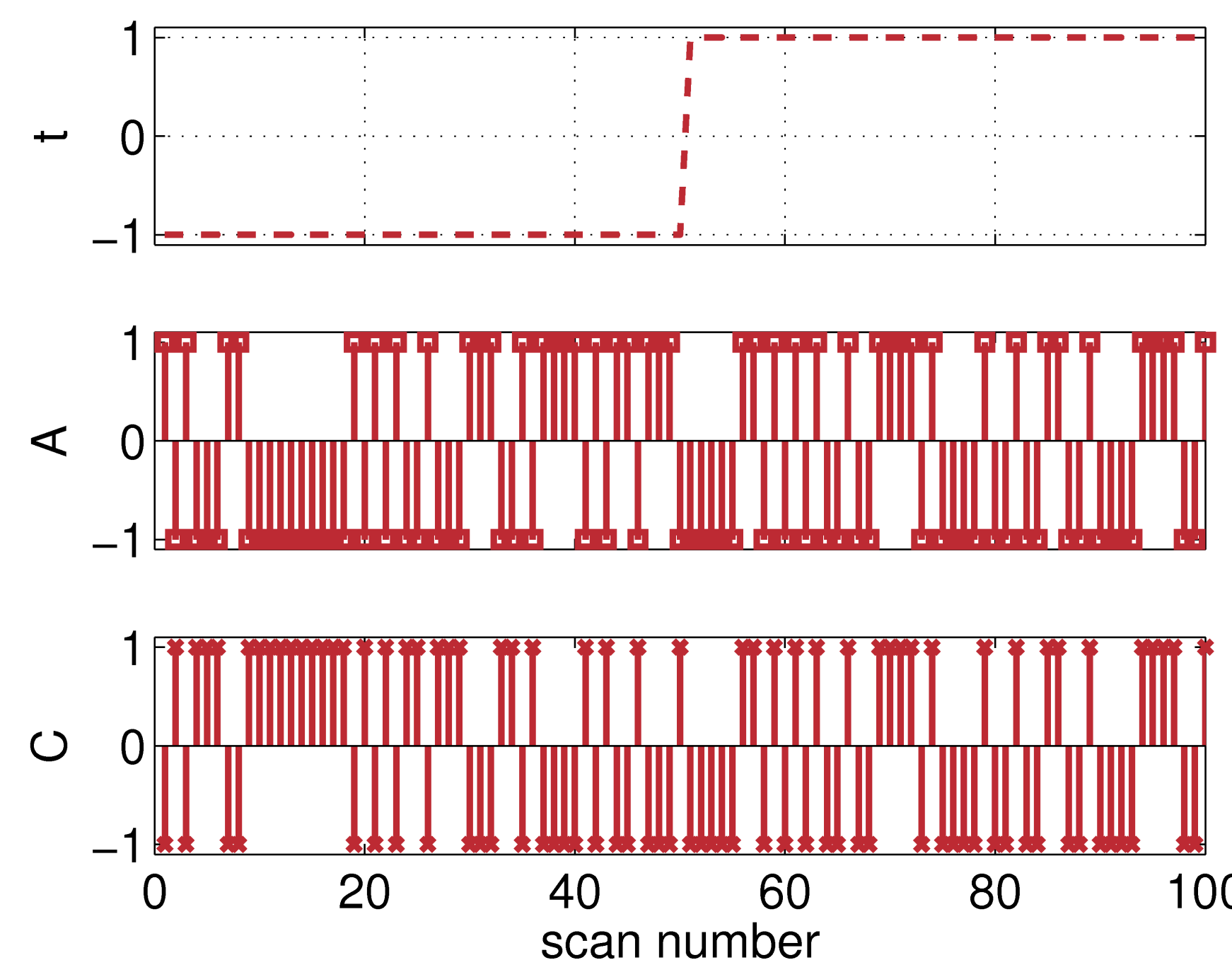
Figure 2: Simulation of regions that interact through a nonlinear relationship. The interrelation between the two regions is important to the classification task. This configuration is aimed at modeling a set of brain regions in which the interaction is modulated by the brain state. There are four spatially contiguous regions that can activate denoted by (A,B,C,D). Initially we let regions (A,B,D) be activated by random sequence taking values \pm 1 . The target signal, coding for an initial baseline taking values t_n = -1 , and for an active state t = 1 . The region (C) is activated with an XOR-sequence relative to region (A) and t_n , so that C_n = A_n t_n . The two regions (B,D) are unrelated to the stimulus reference function t_n but are included to ensure that the brain state can not be decoded based on regional measures, such as variance or non-Gaussianity. Additionally, Gaussian noise was added to the images to obtain a signal to noise ratio of 0.2. Classification accuracy with an SVM was 90% while the corresponding model with a linear kernel achieved 50% accuracy (corresponding to random guessing). Top panel left to right: simulation setup, example of input image, sensitivity map, "true map".
