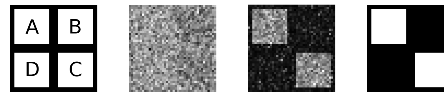
Figure 2: Simulation of regions that interact through a nonlinear relationship. The interrelation between the two regions is important to the classification task. This configuration is aimed at modeling a set of brain regions in which the interaction is modulated by the brain state. There are four spatially contiguous regions that can activate denoted by (A,B,C,D). Initially we let regions (A,B,D) be activated by random sequence taking values \pm 1 . The target signal, coding for an initial baseline taking values t_n = -1 , and for an active state t = 1 . The region (C) is activated with an XOR-sequence relative to region (A) and t_n , so that C_n = A_n t_n . The two regions (B,D) are unrelated to the stimulus reference function t_n but are included to ensure that the brain state can not be decoded based on regional measures, such as variance or non-Gaussianity. Additionally, Gaussian noise was added to the images to obtain a signal to noise ratio of 0.2. Classification accuracy with an SVM was 90% while the corresponding model with a linear kernel achieved 50% accuracy (corresponding to random guessing). Top panel left to right: simulation setup, example of input image, sensitivity map, "true map".
