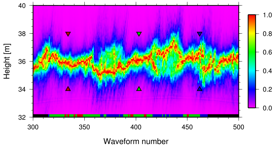
Figure 12: Distribution of the three typical waveform types. The bottom line is color coded after the classification; Gaussian (red), skewed (green), tail (blue), and rejected (black). The three waveforms marked with triangles are selected for further analysis.
