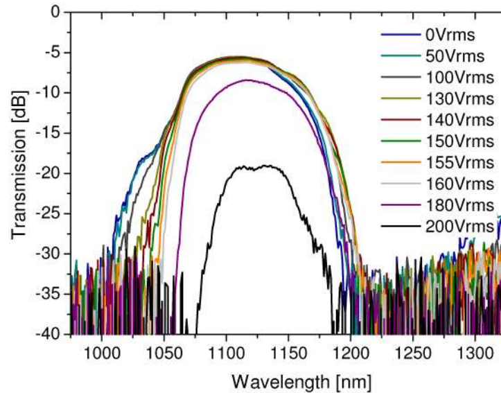
Fig. 5. Transmission spectrum of the all-spliced fiber assembly. The short wavelength bandgap edge is shifted towards longer wavelengths when a voltage is applied. Above 160 V_{rms} the losses in the bandgap become high.
