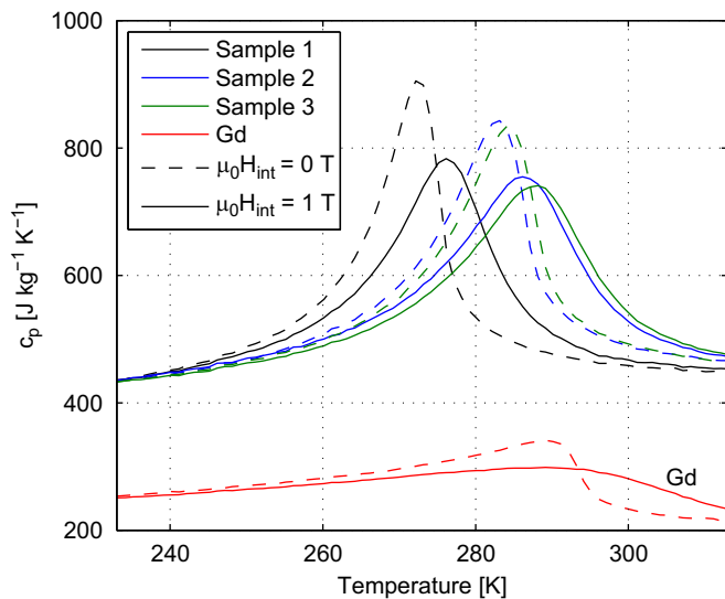
Fig. 5. The values of c_p interpolated at \mu_0 H_{int} = 0 and 1 T as a function of temperature for Gd and the three different samples of LaFeCoSi. The peak temperature increases with increasing sample number for the LaFeCoSi samples.
