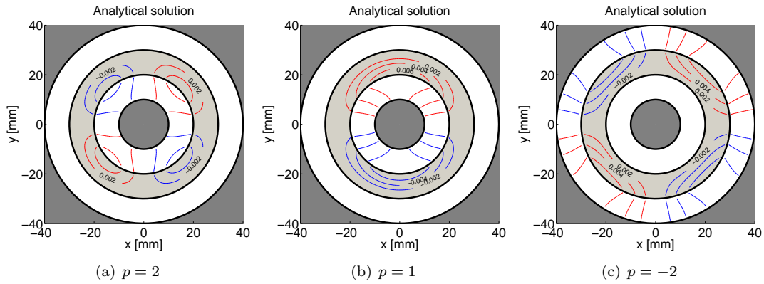
Fig. 5.3: The analytical solution as given by Eqs. (5.12), (5.17) and (5.18). Shown are contours of A_z = \pm[0.002, 0.004, 0.006] \text{V s m}^{-1} for an enclosed Halbach cylinder with dimensions as given in the text and a value of p as given above. The shaded areas in the figures correspond to the similar shaded areas in Fig. 5.2.
