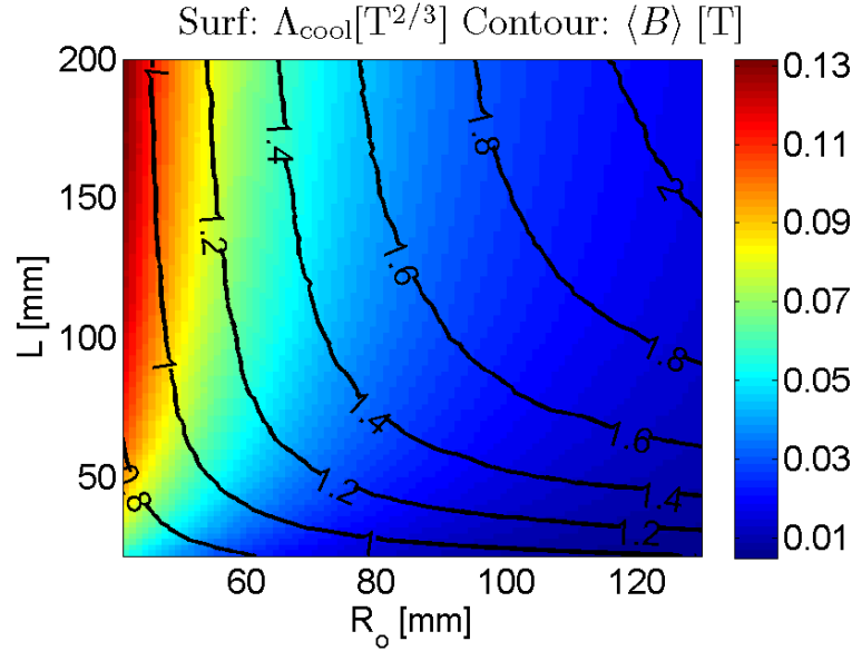
Fig. 5.19: A surface plot showing the magnetic cooling parameter, \Lambda_{cool} , for the Halbach cylinders without additional blocks and with R_i = 20 mm. Also \langle B \rangle is shown as contours.
