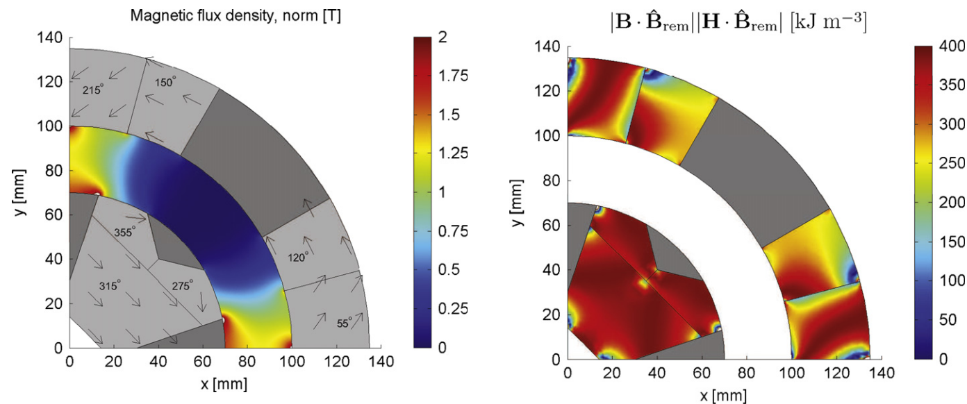
Fig. 4. The segmentation of the final design. The direction of magnetization has been found by maximizing \langle B_{\text{high}}^{0.7} \rangle - \langle B_{\text{low}}^{0.7} \rangle . The direction of magnetization is indicated on each segment. The small white areas in the air gap have a flux density higher than the maximum value on the color bar. (For interpretation of the references to colour in this figure legend, the reader is referred to the web version of this article.)
