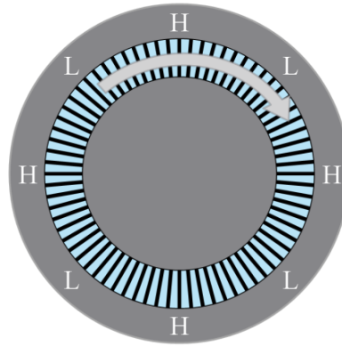
Figure 1: Sketch showing the alternating high and low field regions, as well as the rotating regenerator.
