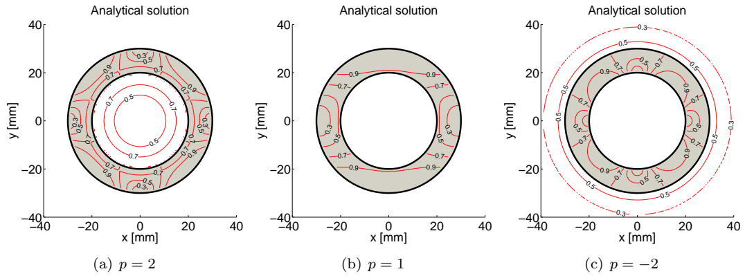
Fig. 5.7: The analytical solution as given by Eqs. 5.26) and (5.27). Shown are contours of \|\mathbf{B}\| = [0.3, 0.5, 0.7, 0.9] T for a Halbach cylinder in air with \mu_r = 1 and with dimensions as given in the text and a value of p as given above. The shaded areas in the figures correspond to the similar shaded areas in Fig. 5.2.
