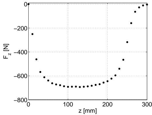
Fig. 7.13: The force on the whole 500 plate regenerator as a function of distance the regenerator is moved out of the air gap. The force is directed into the magnet.
