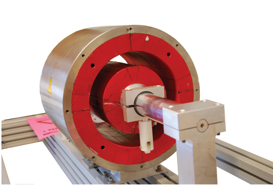
Fig. 7.1: A photo of the actual constructed magnet (in red) including stand and an outer stainless steel casing. The individual segments can be discerned. A small placeholder for a rod to fixate a Hall probe can also be seen.
