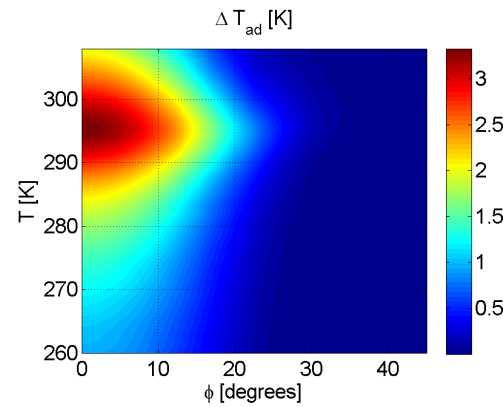
Fig. 7.18: The adiabatic temperature change in a plate at starting temperature, T , located at an angle, \phi . The temperature change for the remaining angles can be obtained by mirror symmetry.
