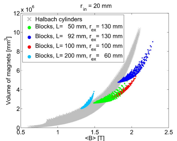
FIG. 10. (Color online) Placing additional blocks on a specific Halbach cylinder improves the mean flux density in the cylinder bore but the improvement depends on L and r_{\text{ex}} of the Halbach cylinder. The legend shows which Halbach cylinder the additional block was placed on. Without the additional blocks the figure is identical to Fig. 7.
