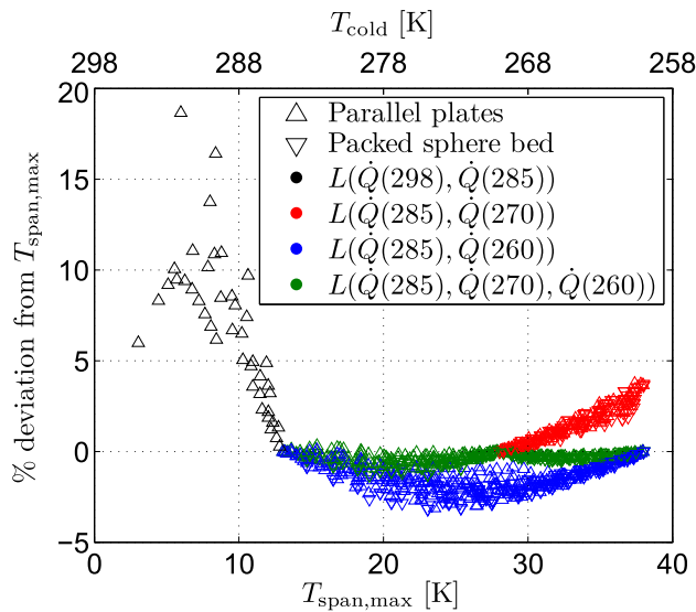
Fig. 4 – The deviation of the estimated T_{\text{span,max}} , based on different linear fits, from the true T_{\text{span,max}} . From T_{\text{cold}} = 285 \text{ K} to 270 \text{ K} the two linear functions L(\dot{Q}(285), \dot{Q}(270)) and L(\dot{Q}(285), \dot{Q}(270), \dot{Q}(260)) are identical, and thus only L(\dot{Q}(285), \dot{Q}(270), \dot{Q}(260)) is shown.
