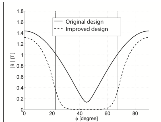
Figure 4: The magnetic flux B = \mu_0 H in the centre of the gap between the magnets as a function of the rotation angle. Adapted from Bjørk et al. (2010b).
