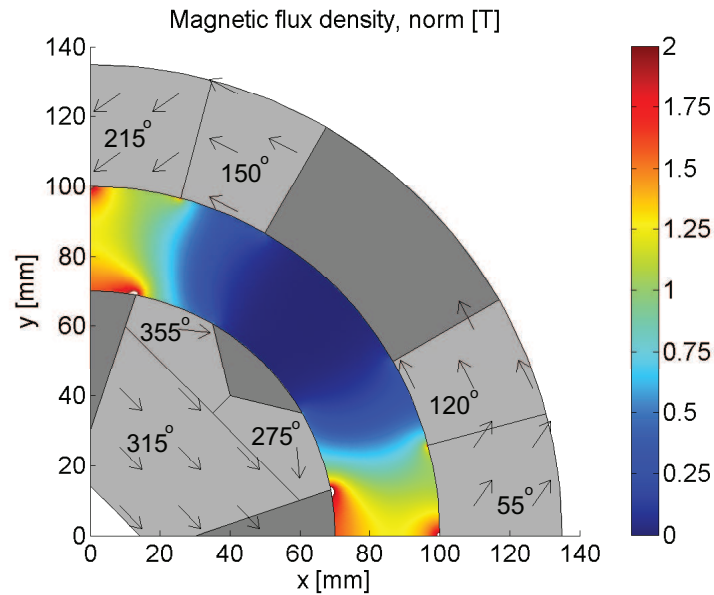
Fig. 6.23: The segmentation of the final design. The direction of magnetization has been found by maximizing \langle B_{\text{high}}^{2/3} \rangle - \langle B_{\text{low}}^{2/3} \rangle and is indicated on each segment. Note that the flux density scale on this figure is larger than on the previous figures in this chapter.
