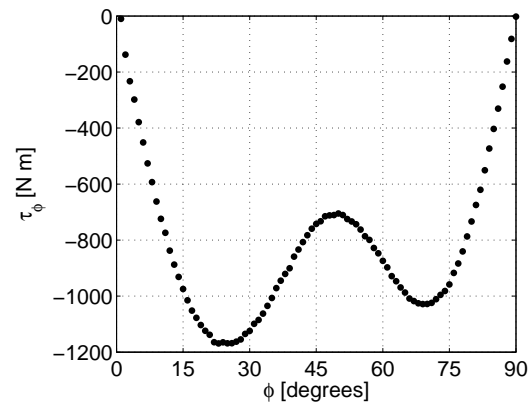
Fig. 7.9: The torque between the inner and outer magnet as a function of the angle the inner magnet has been rotated.
