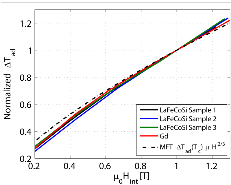
Fig. 2.5: The scaling of the adiabatic temperature change of Gd and three different LaFeCoSi samples as a function of magnetic field at the peak temperature.
