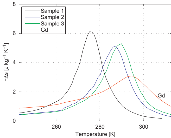
Fig. 4. The values of \Delta s interpolated at \mu_0 H_{int} = 1 T as a function of temperature for Gd and the three different samples of LaFeCoSi. The peak temperature increases with increasing sample number for the LaFeCoSi samples.
