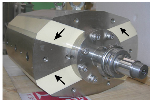
Fig. 12 – The inner magnetic structure in the design by Okamura et al. (2007). From Okamura (2009). The outer magnetic structure consists of a cylinder of soft magnetic material (not shown). The arrows indicate the direction of magnetization of the magnets, which are white in color.
