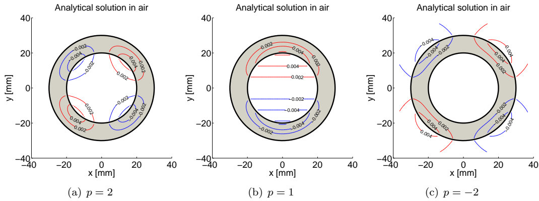
Fig. 5.5: The analytical solution as given by Eqs. (5.12), (5.20) and (5.21). Shown are contours of A_z = \pm[0.002, 0.004, 0.006] \text{V s m}^{-1} for a Halbach cylinder in air with dimensions as given in the text and a value of p as given above. The shaded areas in the figures correspond to the similar shaded areas in Fig. 5.2.
