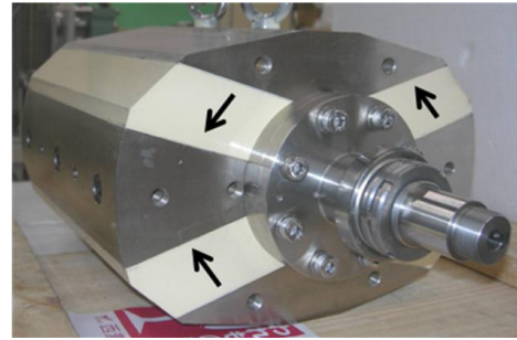
Fig 4: The magnet design by Okamura (2009). The arrows show the direction of magnetization of the magnets (white). The outer yoke is not shown.
