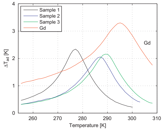
Fig. 6. The values of \Delta T_{ad} interpolated at \mu_0 H_{int} = 1 T as a function of temperature for Gd and the three different samples of LaFeCoSi. The peak temperature increases with increasing sample number for the LaFeCoSi samples.
