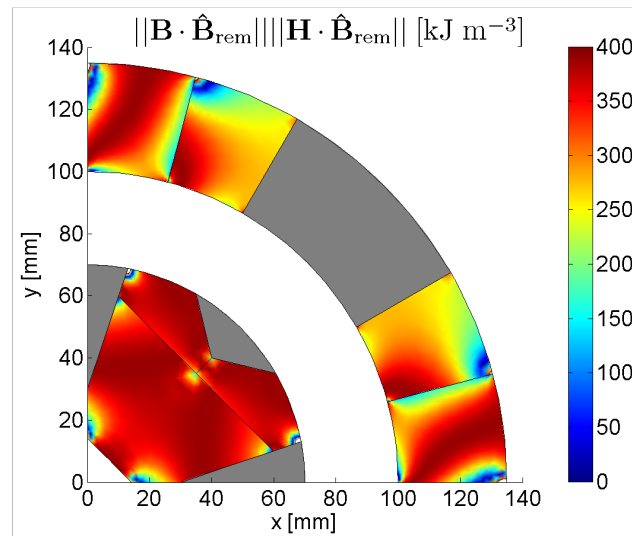
Fig. 6.24: The working point, \|\mathbf{B} \cdot \hat{\mathbf{B}}_{\text{rem}}\| \|\mathbf{H} \cdot \hat{\mathbf{B}}_{\text{rem}}\| , of the magnets. The maximum working point for a 1.44 T remanence magnet, as is used here, is 400 \text{ kJ m}^{-3} .
