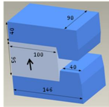
Fig 1: The magnet design by Zheng et al. (2007). From Zheng (2009). The blue material is soft magnetic material. All dimensions are in mm. The arrow indicates the direction of magnetization.
