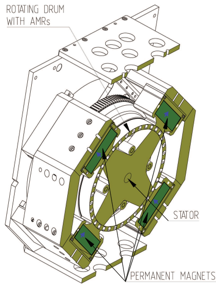
Fig. 4.11: The design by Tušek et al. (2009). The green structures consist of soft magnetic material while the dark green structures are magnets. The small blue arrows indicated the direction of magnetization. From Tušek et al. (2009).
