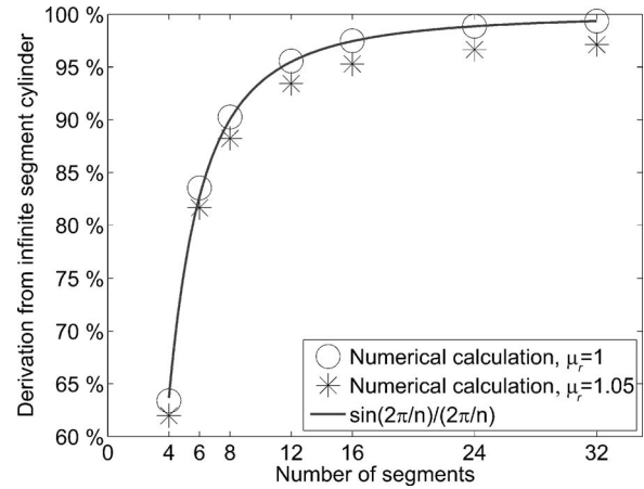
FIG. 2. Dividing a Halbach cylinder into n segments makes the flux density differ from that of a perfect Halbach cylinder. The deviation is given by Eq. (4) for “perfect magnets,” \mu_r=1 , while magnets with \mu_r=1.05 deviate more from the ideal Halbach cylinder.
