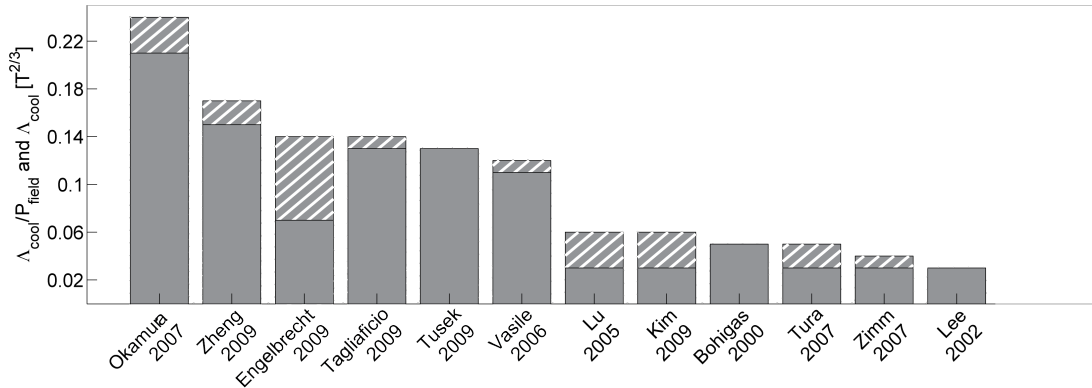
Fig. 4.20: The parameters \Lambda_{\text{cool}}/P_{\text{field}} (hatched) and \Lambda_{\text{cool}} (full). The \Lambda_{\text{cool}}/P_{\text{field}} parameter only takes the magnet design into account and not the fraction of time the magnet is used. As P_{\text{field}} \leq 1 the \Lambda_{\text{cool}} parameter is always less than or equal \Lambda_{\text{cool}}/P_{\text{field}} . Completely filled bars have P_{\text{field}} = 1 . Note that the best design is five times as good as the design with the lowest value of \Lambda_{\text{cool}}/P_{\text{field}} .
