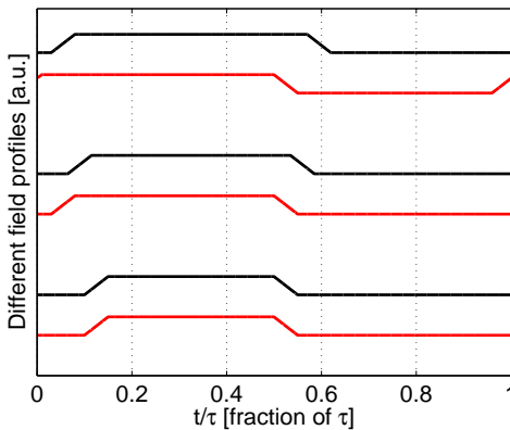
Fig. 3.11: Three of the different magnetic field profiles for the width experiment. The black curves are centered on the fluid flow profile (not shown), while the red curves are synced, i.e. the time at which the magnetic field is ramped down is fixed at t = \tau_1 + \tau_2 = 0.5 .
