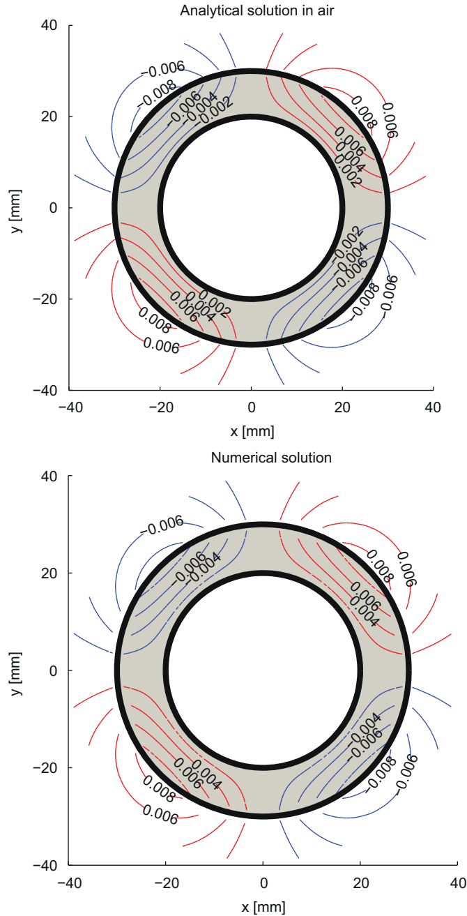
Fig. 4. (Color online) Comparing the analytical solution as given by Eqs. (8) and (18) with a numerical solution computed using Comsol. Shown are contours of A_z = \pm [0.002, 0.004, 0.006, 0.008] \text{ Vs m}^{-1} for an external field p = -2 Halbach cylinder in air with dimensions R_i = 20 \text{ mm} , R_o = 30 \text{ mm} and B_{\text{rem}} = 1.4 \text{ T} , \mu_r = 1.05 . The red contours are positive values of A_z while the blue are negative values. As with Fig. 3 the solutions are seen to be identical. (For interpretation of the references to color in this figure legend, the reader is referred to the web version of this article.)
