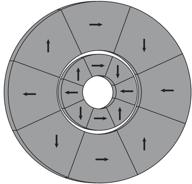
Fig. 10 – A sketch of the concentric Halbach magnet design by Tura and Rowe (2007), viewed from the front. The inner and outer radius of the inner cylinder is 12.5 mm and 27 mm, respectively while the corresponding figures for the outer cylinder is 30 mm and 60 mm, respectively. The rotational length of the actual concentric cylinder is 100 mm. The configuration shown here is the high flux density configuration.
