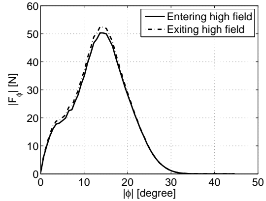
Fig. 7.20: The force on a plate with a linear temperature profile from 273 K to 303 K as it enters and exits the high field region. At the center of the high field region, \phi = 0^\circ , the generated heat is removed and the plate brought back to its original linear temperature profile. The exiting force is negative.
