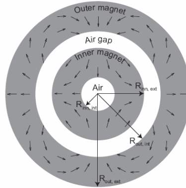
Figure 3: Two concentric quadropole Halbach type cylinders. The inner magnet directs the field outward, while the outer one directs the field inward.
