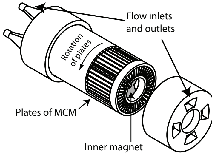
Fig. 6.1: A drawing of the design idea for the magnetic refrigeration device. The plates of MCM rotate, while the magnet and the fluid inlets and outlets are stationary. The outer magnetic structure is not shown in this drawing. The temperature gradient is along the plates. Adapted from Bahl et al. (2009).
