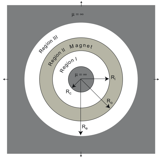
Fig. 2. A Halbach cylinder with inner radius R_i and outer radius R_o enclosing an infinitely permeable cylinder with radius R_c while itself being enclosed by another infinitely permeable cylinder with inner radius R_e and infinite outer radius. The regions marked I and III are air gaps.
