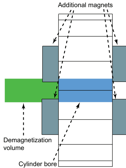
Fig. 5.18: A side view of the Halbach cylinder with additional blocks. The volume inside which \langle (\mu_0 H)_{\text{low}}^{2/3} \rangle is calculated is labeled “Demagnetization volume”. The volume is identical in shape to the cylinder bore and is located directly outside the end of the cylinder bore. Also shown are the additional blocks of magnets. The edges of the 16 segments that make up the Halbach cylinder can also be seen on the figure.
