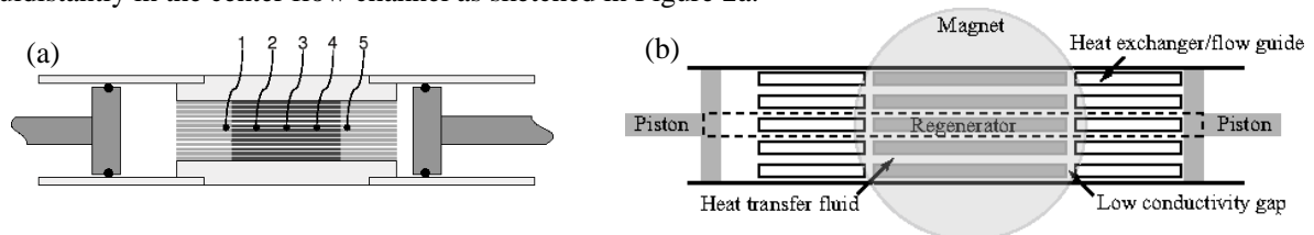
Figure 2: Drawing (a) is a schematic of the regenerator pictured in Figure 1a. The locations of the five thermo-couples are indicated with their appropriate numbers. Thermo-couples 1 and 5 are placed at the cold and hot ends respectively. Figure (b) shows how the numerical model represents the full geometry of the AMR. The model breaks the geometry down into a single replicating cell consisting of one half of a complete flow channel (indicated with a dashed line in the figure and magnified in Figure 3).
