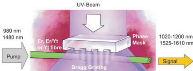
Figure 2.4: Distributed feedback fiber laser consisting of a Bragg grating UV written in actively doped fiber and pumped at 980 nm of 1480 nm. Courtesy of NKT Photonics A/S.
