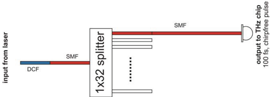
Figure 5.11: Schematic of the fiber link. The input laser pulse is stretched in a dispersion compensating fiber (DCF) module with single mode fiber (SMF) pigtailed. The DCF module is spliced onto a 1 \times 32 splitter and each of these channels is spliced onto a piece of single mode fiber for pulse compression.
