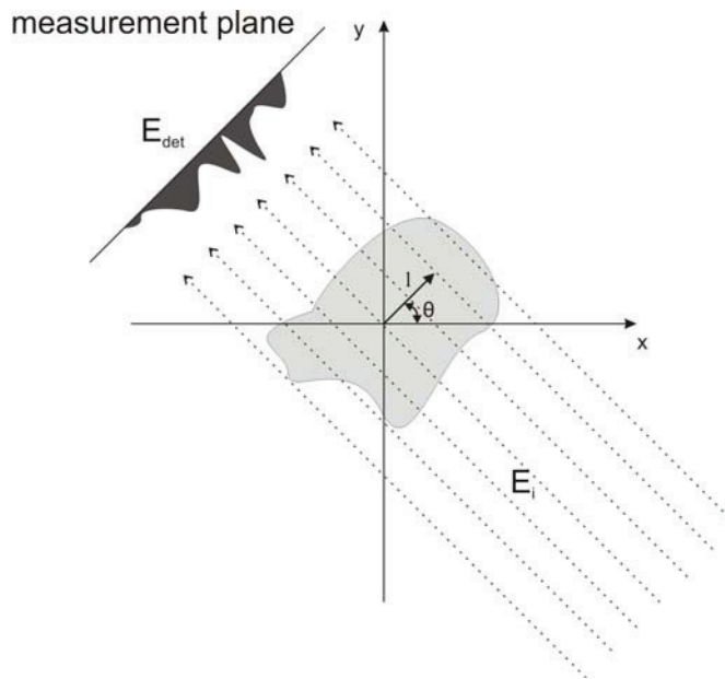
Figure 3.12: Schematic of computed tomography. The object is rotated around the z -axis ( z is out of the page). The incident THz beam E_i propagates through the object at an angle \theta and a offset l from the rotation axis. In the measurement plane both the amplitude and the phase of E_{det} is detected.
