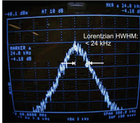
Figure 2.10: Self-heterodyne linewidth measurement, which shows a linewidth of the two-color laser of below 24 kHz.
