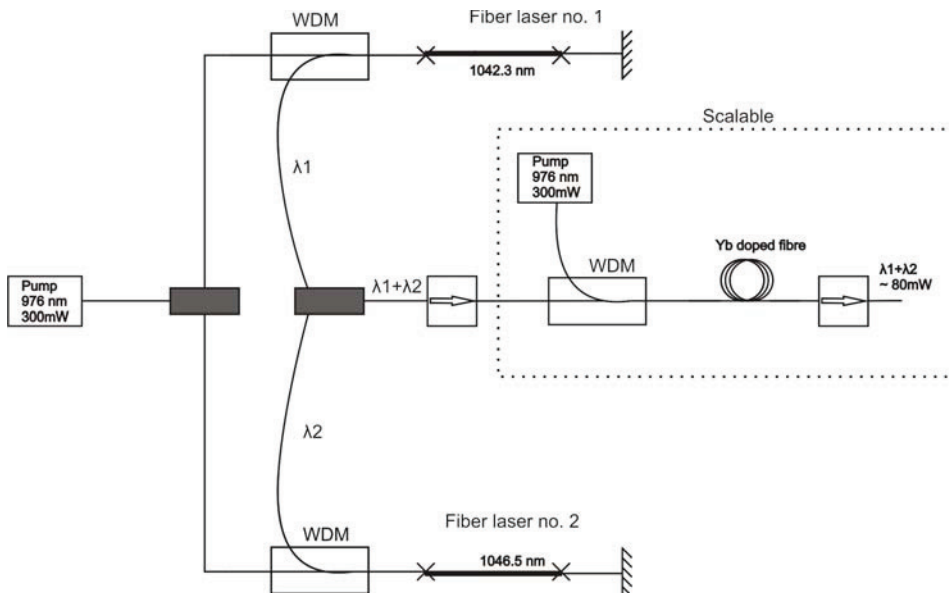
Figure 2.8: Sketch of the first principle of the two-color laser. The two oscillators are followed by an amplifier stage combining and amplifying the oscillator signal.
