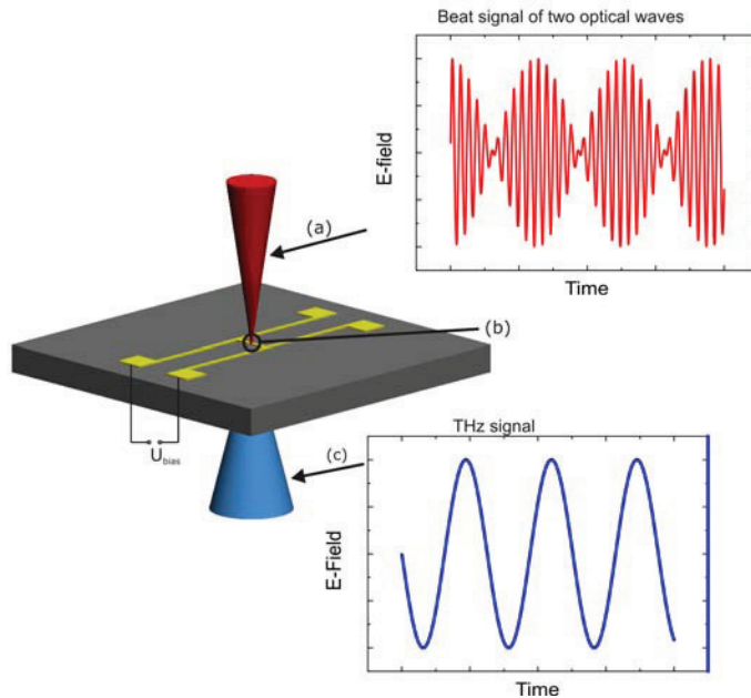
Figure 2.1: CW THz emitter with H-structure dipole metal structure on a semiconductor substrate. THz radiation is generated by photomixing of two slightly detuned laser beams. (a) Beat signal of \omega_1 and \omega_2 with difference frequency of \omega_{THz} . (b) The generated photocurrent is proportional to the optical input power, I_{ph} \propto P_{opt} \sin(\omega_{THz}t) . (c) The radiated THz power is proportional to the photocurrent squared, P_{THz} \propto I_{ph}^2 .
