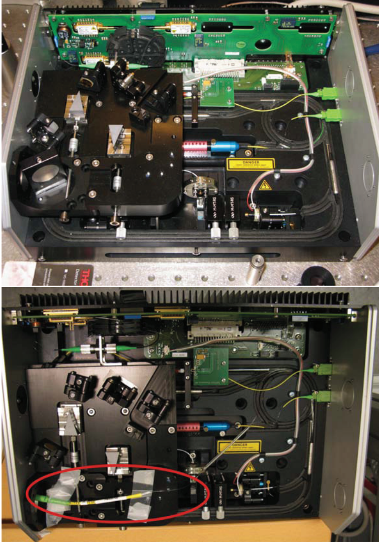
Figure 5.6: (top) FFS.SYS laser before rerouting of the prism-compressor. The output pulse length was measured to 110 fs. (bottom) The prism-compressor is now rerouted and the original free-space output coupler removed and replaced by an APC/FC-connector. The connector was fusion spliced onto the fiber laser output. The output pulse length directly out of the fiber connector is measured to 0.9 ps and the output power increased by approximately 25%.
