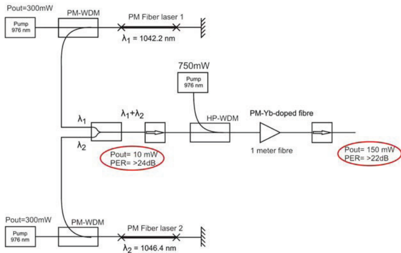
Figure 2.12: Sketch of a polarization maintaining two-color fiber laser setup with individual pumps for each oscillator followed by an Yb-doped fiber amplifier pumped with 750 mW.
