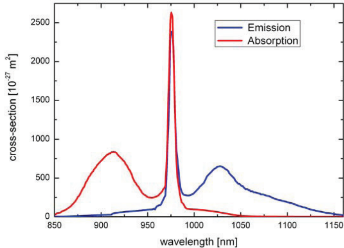
Figure 2.6: Absorption and emission cross section of Yb in germanosilicate glass. [49]
