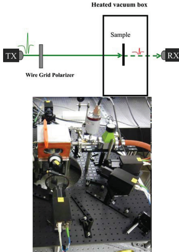
Figure 4.10: Measurements setup used with the CNT film. Measurement box characteristics: Pressure: min. 24 \text{ kN} \cdot \text{m}^{-2} , low absorption and low dispersion TOPAS windows, PID controlled temp. up to 250^\circ\text{C} .
