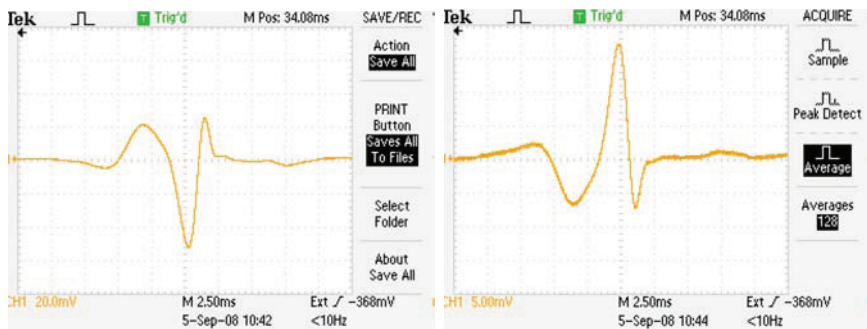
Figure 5.30: THz traces recorded at a scan rate of 8 Hz, using the newly developed current preamplifier (left) and a commercially available preamplifier (right). Our design shows a lower baseline noise and higher bandwidth than the commercial product.
