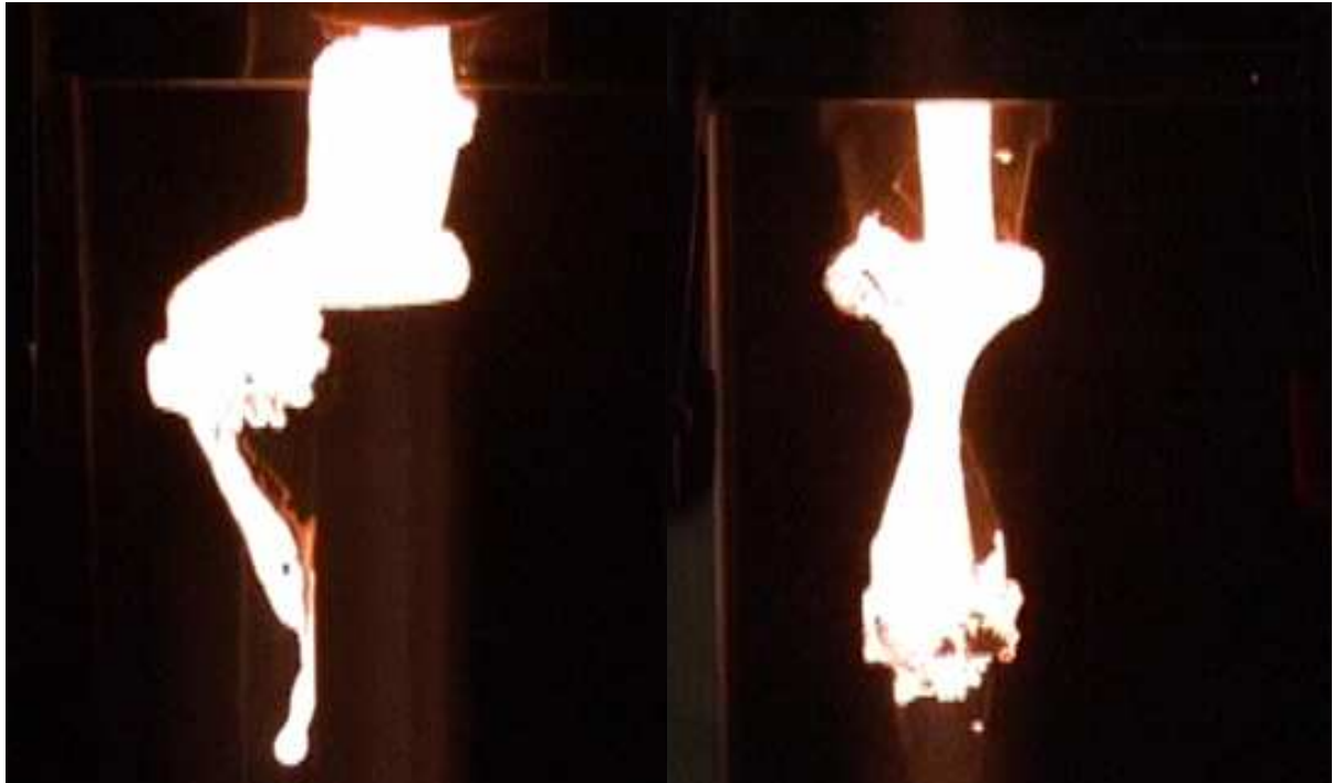
Figure 8-10 Frames from the glass plate experiments showing the initial melt passing through the foam filters. The frames show that the melt does not exit the filter in a coherent stream.
