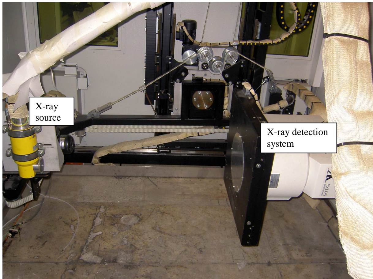
Figure 5-7 Inside of the x-ray chamber. To the left: the x-ray source. To the right: the x-ray detection system.
