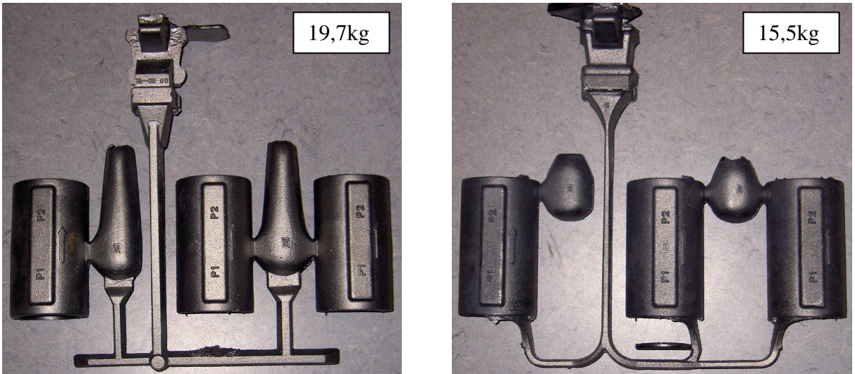
Figure 6-3 Picture to the left: castings with the traditional layout. Picture to the right: castings with the streamlined layout.
