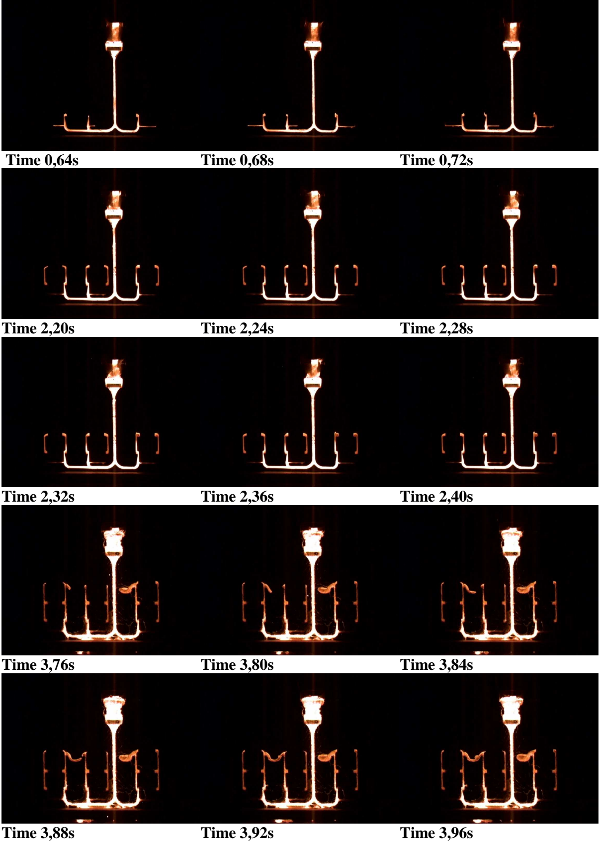
Figure 6-9 Streamlined gating system. A pressed filter is used.
