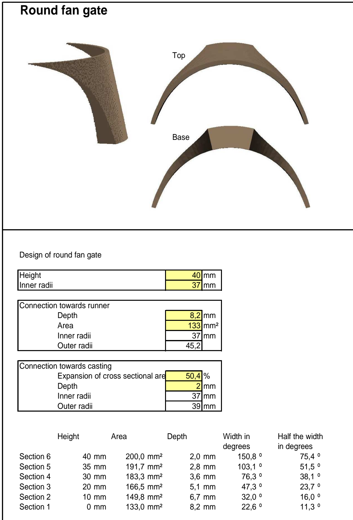
Figure 3-8 Sheet 3 – Fan gates. This part of the sheet is used for designing a round fan gate. This type of fan gate can be useful for filling of a cylinder shaped casting.
