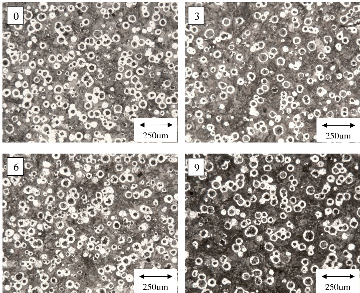
Figure 6-6 Microstructures in the centre flange from the streamlined layout
