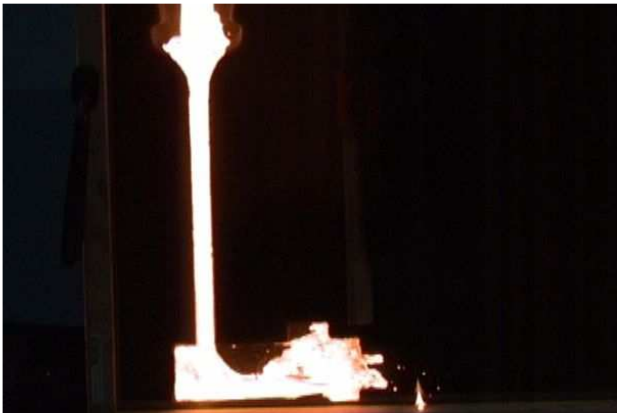
Figure 8-11 Frame from the glass plate experiments showing the initial melt passing through the foam filter. The frame shows that the melt does not exit the filter in a coherent stream.
