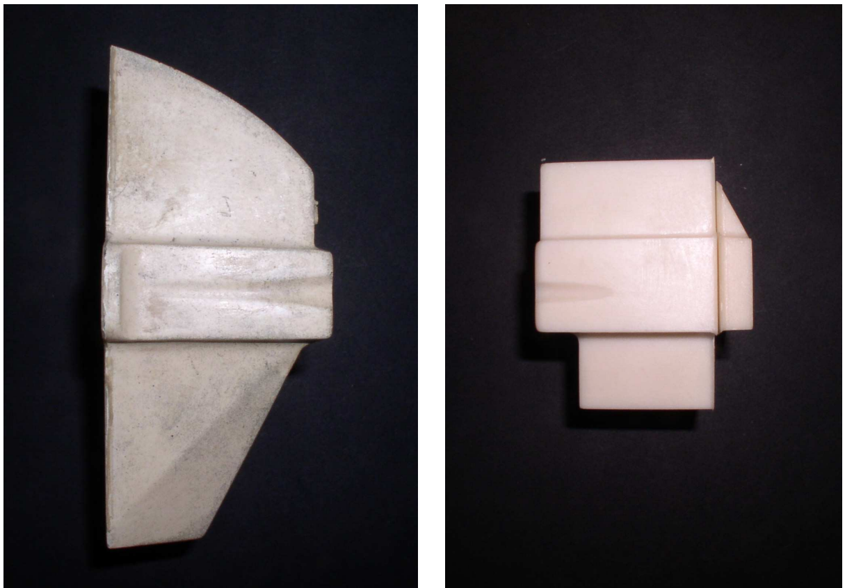
Figure 8-6 Filter prints for vertical moulding. To the left: Filter print as seen in the traditional layout presented in 'Theory in gating technology'. To the right: Replica of a filter print.
