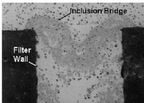
Figure 8-3 [Ref. 8-3] Micrograph of an inclusion bridge
