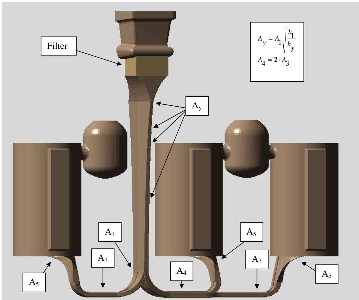
Figure 2-5 The streamlined gating system
