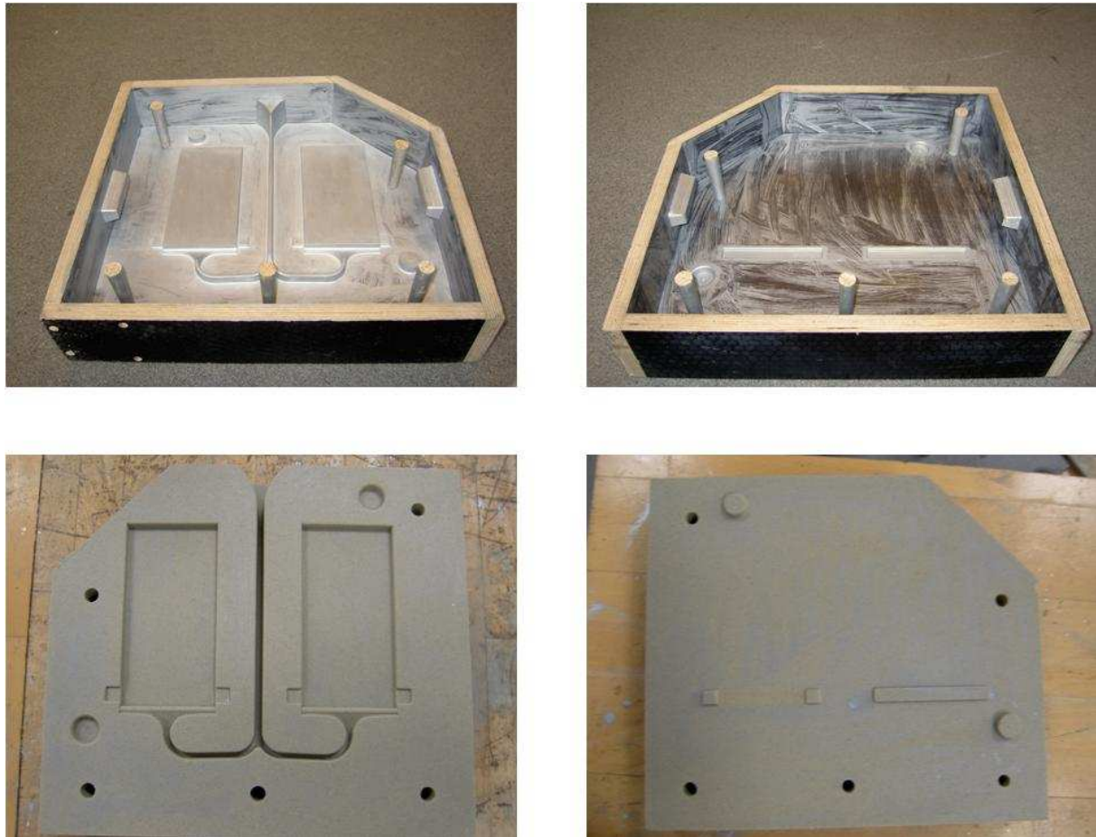
Figure 9-2 Top left: Pattern plate with the castings. Top right: Pattern plate with the ‘cores’. Bottom left: Sand mould with the castings. Bottom right: Sand mould with the core to the left removed and the core to the right intact.
