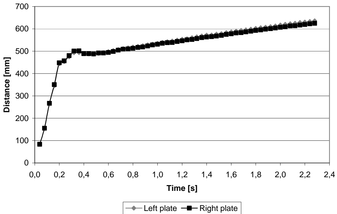
Graph 9-7 The distance which the front of the melt has moved plotted against the time for the experiment with glass plate fronted mould.
