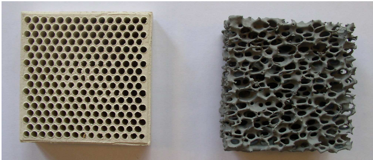
Figure 8-1 Ceramic filters. To the left: a pressed filter, size: 50mm x 50mm, diameter of the holes: 2,4mm. To the right: a foam filter, size: 50mm x 50mm, porosity: 10ppi (pores per inch)
