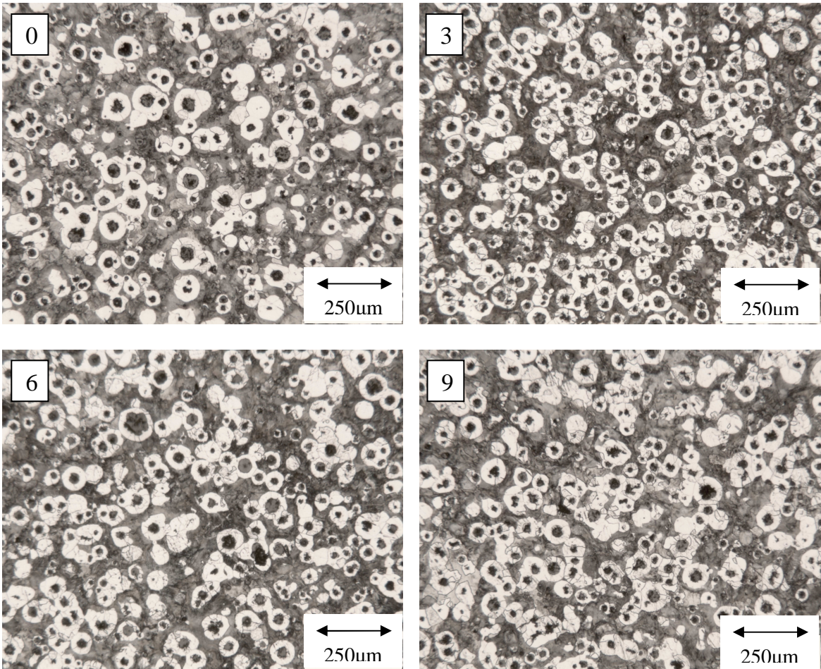
Figure 6-5 Microstructures in the centre flange from the traditional layout
