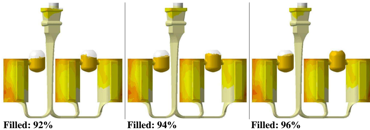
Figure 4-9 Simulation results – The streamlined layout
