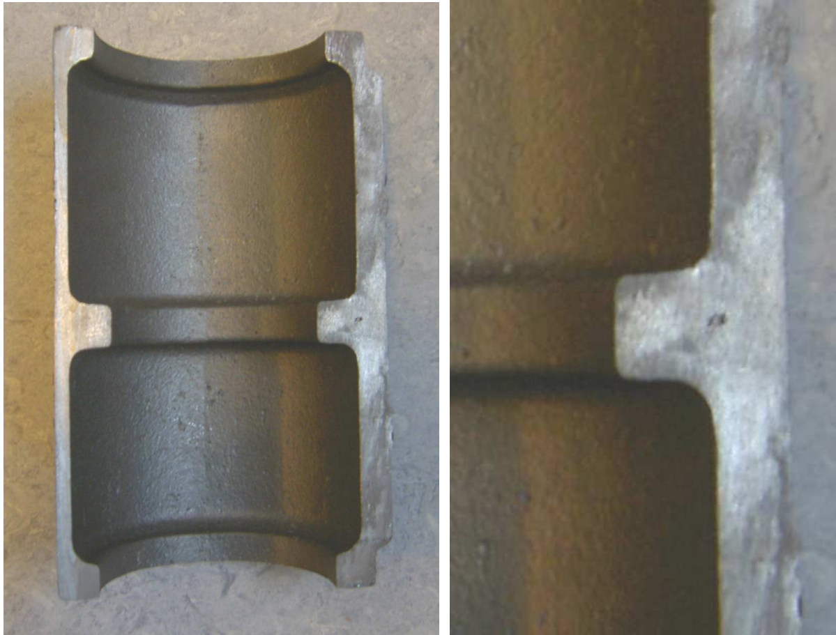
Figure 6-7 To the left: Casting from the streamlined gating system that has been cut through vertically. The right side of the casting is middle of the thick bar on the side of the casting. A small porosity is seen here. To the right: A close up of the small porosity.
