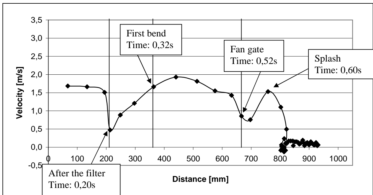
Graph 8-2 The graph shows the measured velocities through out the mould filling
