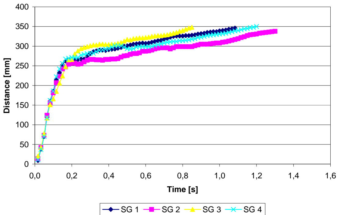
Graph 9-3 The distance which the front of the melt has moved plotted against the time for the experiments with ductile iron. Here 'Ductile iron 1' is called 'SG 1' for convenience.
