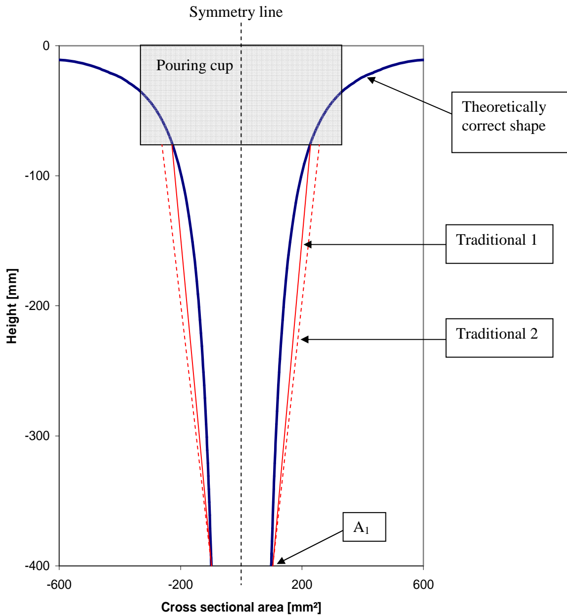
Figure 2-2 Graphical representation of height plotted against cross sectional area in the down runner. The curves ‘Traditional 1’ and ‘Traditional 2’ represent two designs of straight tapered down runners.
