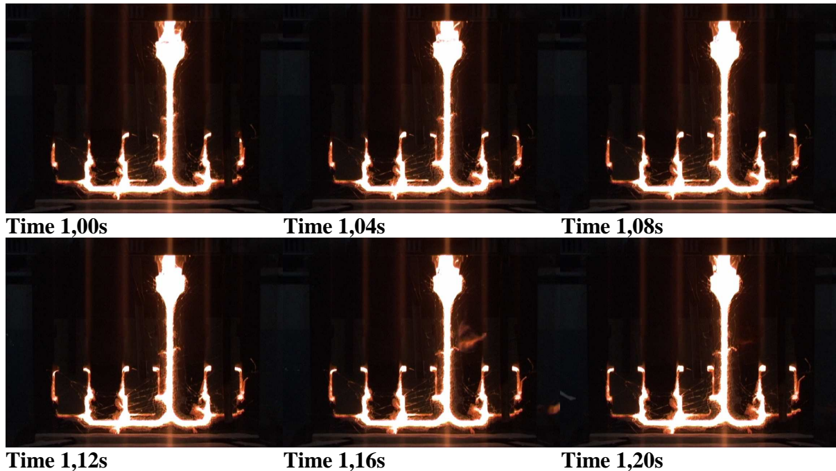
Figure 6-10 Streamlined gating system. No filter is used
