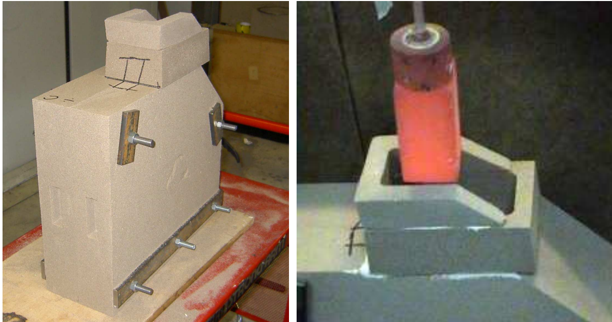
Figure 9-3 To the left: The fully assembled mould ready to be placed in the X-Ray chamber. To the right: Preheated stopper being placed in the pouring basin
