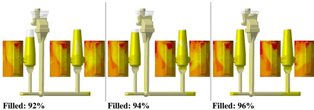
Figure 4-8 Simulation results – The traditional layout
