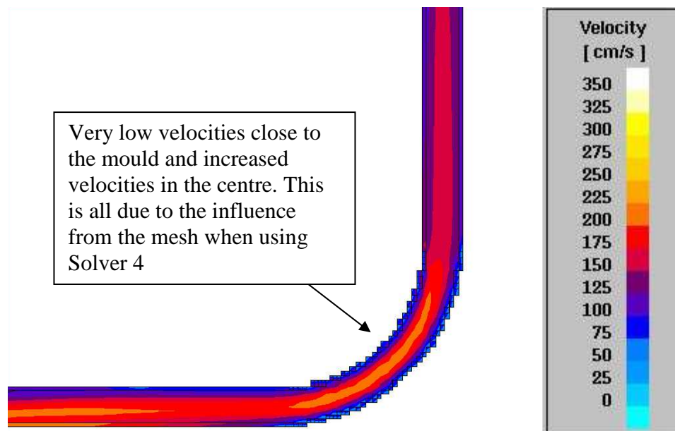
Figure 4-5 Velocities in a bend under a down runner using solver 4. The Influence of the mesh on the flow path in the bend is clearly seen.
