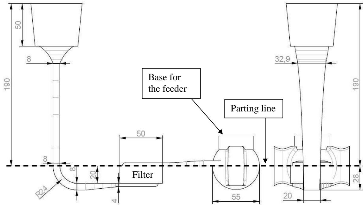
Figure 10-3 The figure shows drawings and dimensions of the streamlined gating system.
