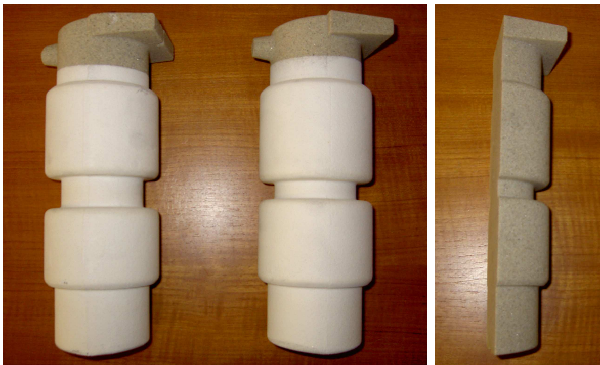
Figure 6-1 To the left: A core for the traditional layout. In the Middle: A core for the streamlined gating system. To the right: half a core used for experiments using glass plate fronted moulds.
