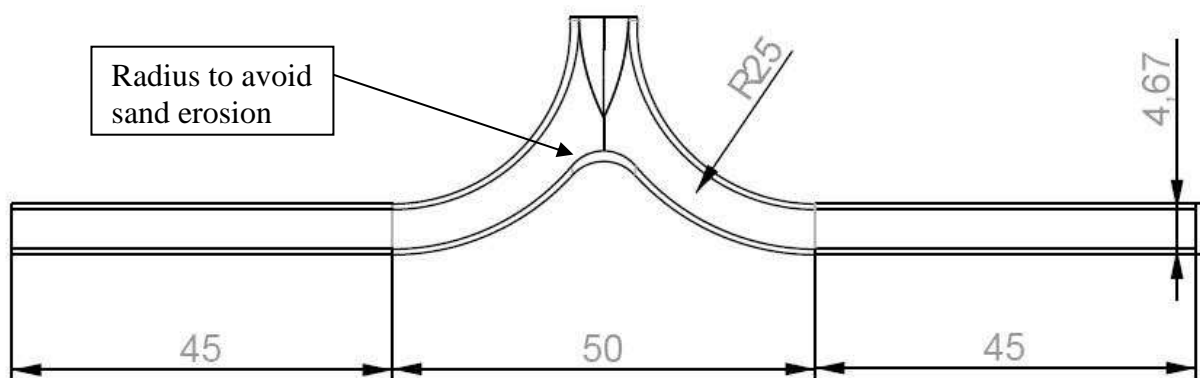
Figure 3-13 The figure shows an example of how the combination of to standard geometries for bends can be used for guiding the melt to either side under the down runner. Between the two bends a small radius is put to avoid sand erosion.
