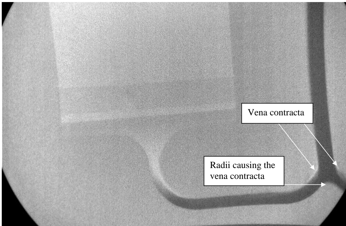
Figure 9-8 Frame showing the small vena contracta observed in the x-ray experiments. The reason for the vena contracta is the small radii between the two bends not compensated for.
