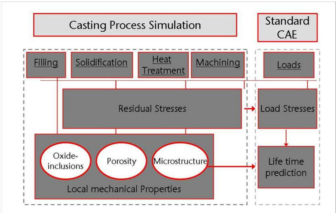
Figure 4-1 Schematic illustration of integrated modelling. [Ref. 4-1]
