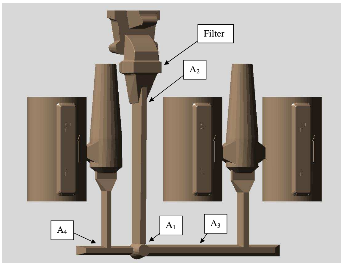
Figure 2-3 The traditional gating system.
