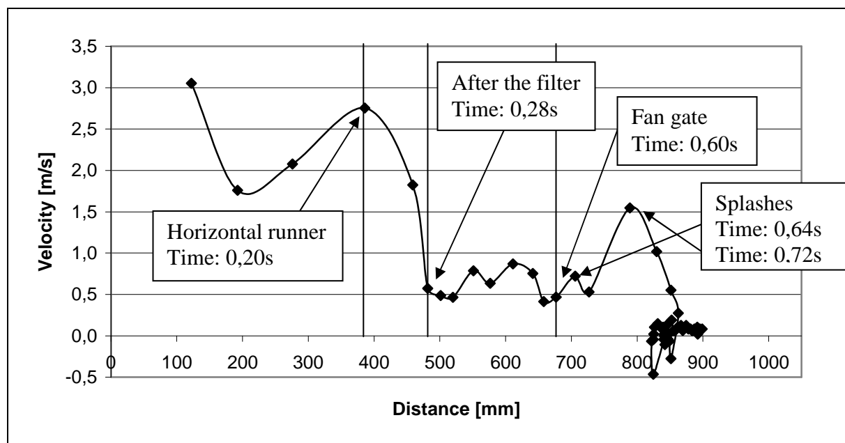
Graph 8-3 The graph shows the measured velocities through out the mould filling
