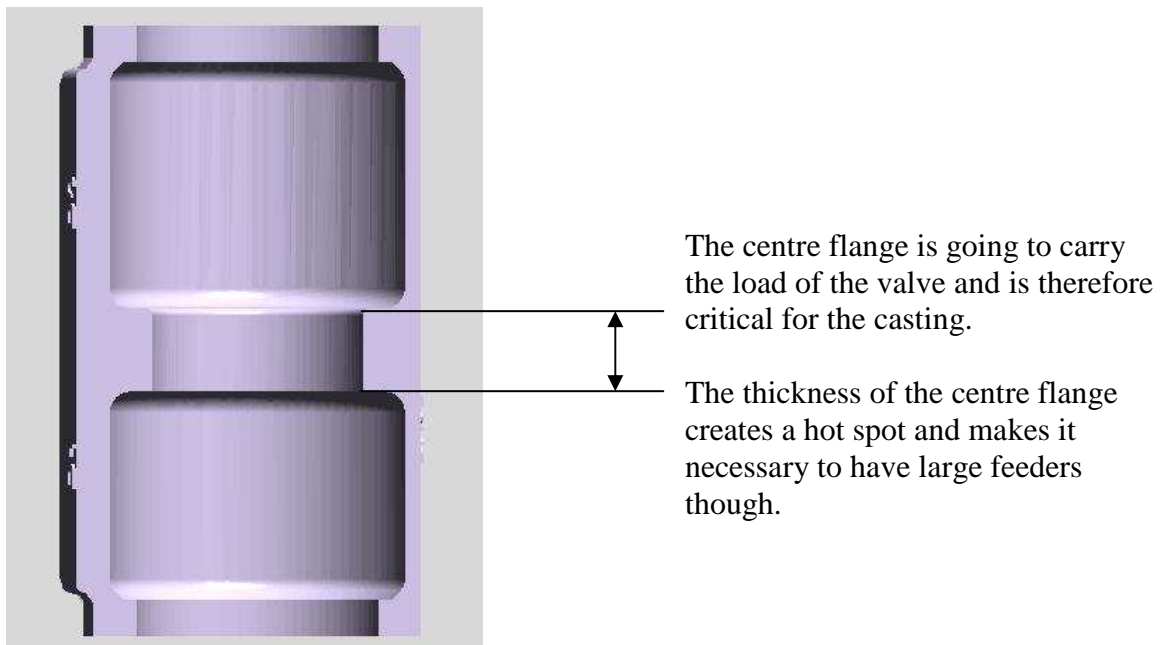
Figure 4-3 Three dimensional representation of the valve housing cut through. The possibility of reducing the thickness of the centre flange is considered.
