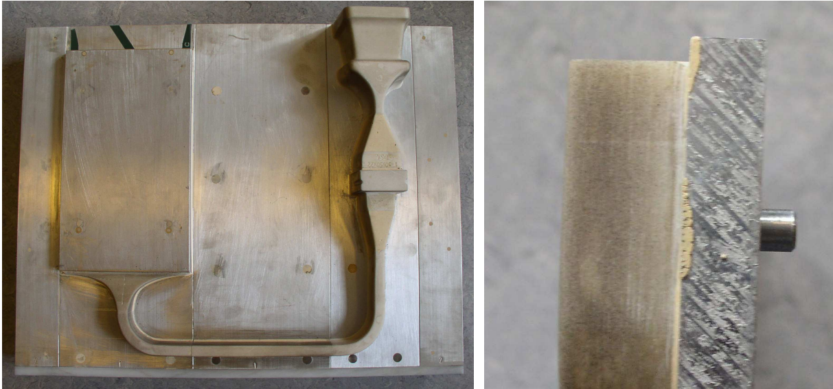
Figure 5-2 To the left: A layout consisting of three modules each going from the top to the bottom of the base plate. To the right: a close up of a module seen from the bottom. From left a part of the runner is seen. In the middle the 10mm module plate and to the right the lower part of the guide pin is seen.
