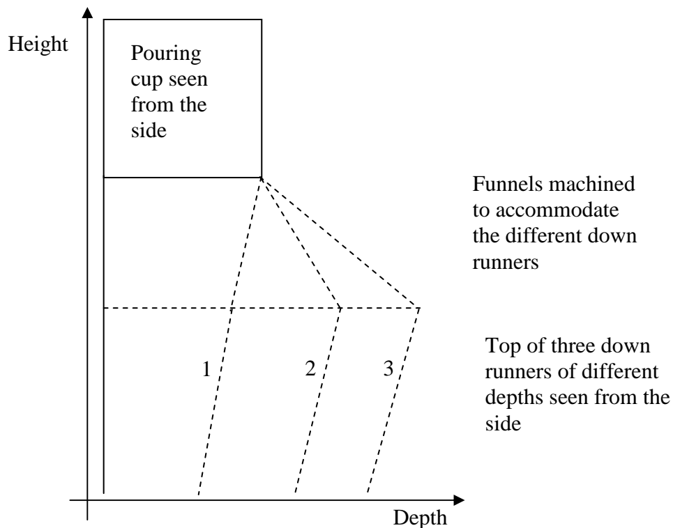
Figure 2-12 The figure shows schematically how the depth of the funnel is modified to accommodate down runners of different depth but always with the same pouring cup
