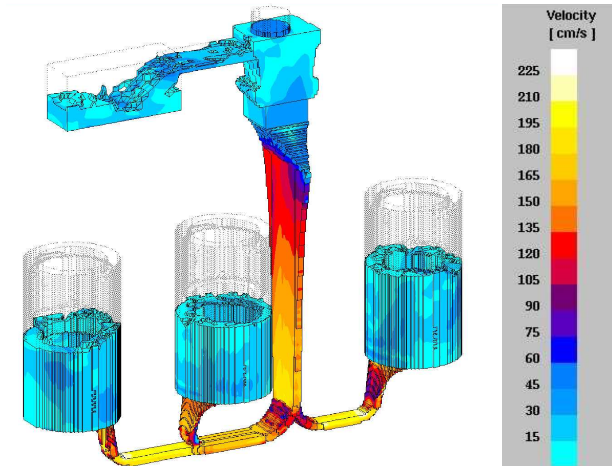
Figure 4-7 The picture shows the principle in having an over flow. The over flow prevents the pressure wave that occurs if the pouring cup is filled prematurely.
