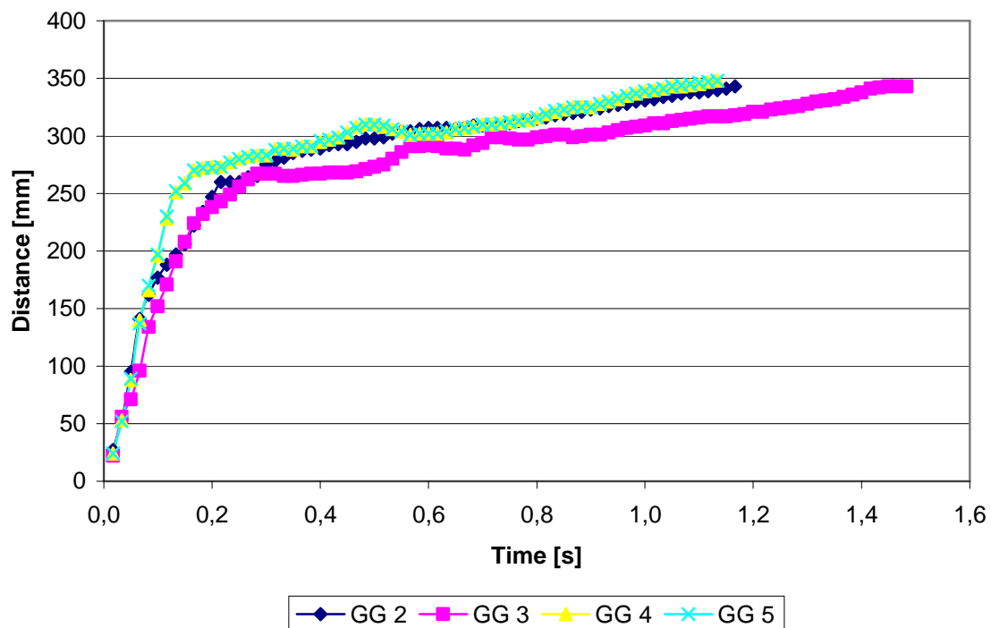
Graph 9-5 The distance which the front of the melt has moved plotted against the time for the experiments with gray iron. Here ‘Gray iron 2’ is called ‘GG 2’, ‘Gray iron 3’ is called ‘GG 3’, ‘Gray iron 4’ is called ‘GG 4’ and ‘Gray iron 5’ is called ‘GG 5’ for convenience.
