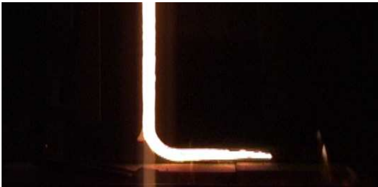
Figure 7-2 The frame shows the front of the melt in the horizontal runner. The time for the frame is 0,28s.
