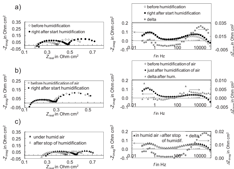
Figure 3. Impedance spectra (Nyquist and -Z_{\text{imag}} vs f plot) recorded under current load, just before the start of the 4% humidification of air and right after the start at (a) 750°C and 0.75 A/cm 2 (2test50), (b) 800°C and 0.5 A/cm 2 (5test34), and (c) recorded just before and after stopping humidification of air at 750°C and 0.75 A/cm 2 (12test33). Delta in the plots are the differences between the two shown spectra. For test conditions see also Table I.
