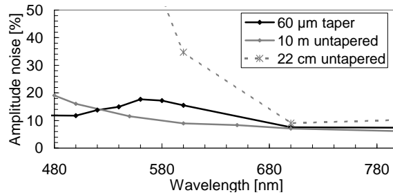
Figure 5.9: Noise curves for a taper with a 60 \mu\text{m} waist compared to a 10 m long untapered fiber (solid gray). This is compared to a 22 cm untapered fiber (dotted gray) which represents the spectrum entering the taper.
