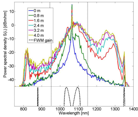
Figure 3.5: Development of the spectrum along the fiber according to numerical simulations. Vertical dotted black lines mark the ZDWs at 954 nm and 1152 nm. The FWM gain, shown in the lower part of the figure, is calculated for the pump power of 116 mW used in the simulation. The FWM gain peaks are at 877 nm, 1039 nm, 1091 nm, and 1354 nm.
