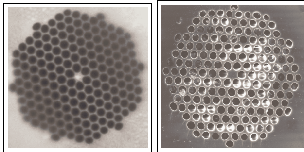
Figure 5.5: Left: Optical microscope photograph of the waist cross section of a fiber tapered to 60 \mu\text{m} waist width recorded with \times 100 magnification. Right: SEM picture of the waist cross section of a fiber tapered to 62.5 \mu\text{m} . The color differences across the fiber facet on the SEM picture are caused by surface damage from the imaging electron beam, contamination and astigmatism in the lens effect created by the electric field.
