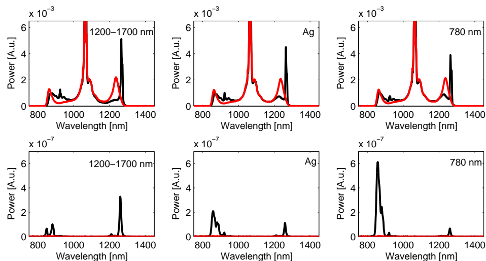
Figure 3.12: SC spectra generated using various feedback spectra. The three columns correspond to the spectra produced using a 1200-1700 nm mirror (left), an Ag mirror (center), and a broad spectrum mirror centered at 780 nm (right) as the SDC mirror. The top row shows the output spectrum from the PCF with (black) and without (red) feedback, while the bottom row shows the spectrum which is fed back through the system, measured at mirror 7 in the setup. Only the light being fed back with the SDC mirror is shown, because the reflection from the fiber facets alone is too small to be seen on a linear scale. Note that all these spectra are plotted on a linear scale.
