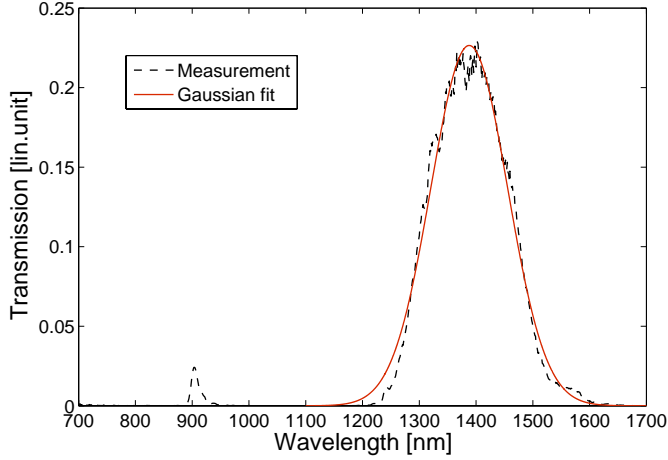
Figure 5.6: Measured transmission spectrum at room temperature of a tapered LMA-10 filled with E7. The amplitude of the Gaussian fit is 0.22, the mean value is 1388nm and the standard deviation is 67.42nm.
