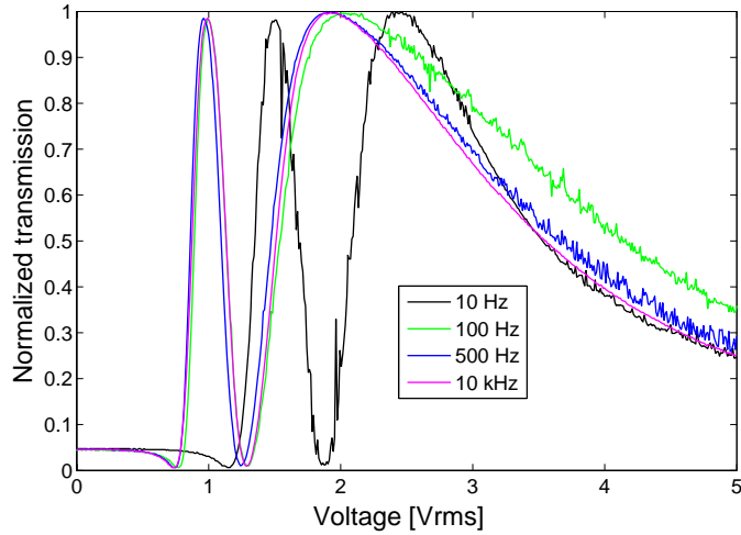
Figure 6.17: Voltage-dependent transmission of a homogeneous 8\mu\text{m} cell filled with \text{BaTiO}_3 nanoparticle-doped E7 for different frequencies of the external applied field.
