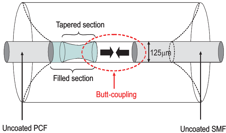
Figure 5.12: Illustration of the mechanical splice of the oil infiltrated PCF with the SMF. UV curable polymer is positioned on top and cured in order to give mechanical stability to the device.
