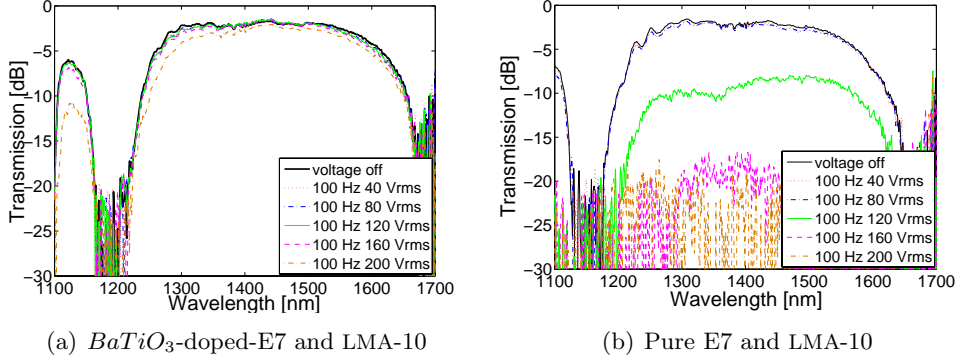
Figure 6.10: Transmission spectra for various amplitudes of the applied field at a frequency of 100Hz.
