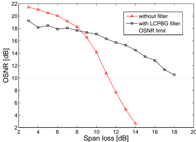
Figure 7.4: OSNR versus span-loss when no filter is inserted in the transmission spectrum and when the LCPBG filter is used. The number of transmitted spans was fixed at 10.
