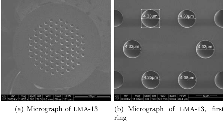
Figure 4.7: SEM of the end facet of LMA-13. The hole size d , inter-hole distance \Lambda and fiber outer diameter D are 4.3\mu\text{m} , 8.5\mu\text{m} and 125\mu\text{m} , respectively.
