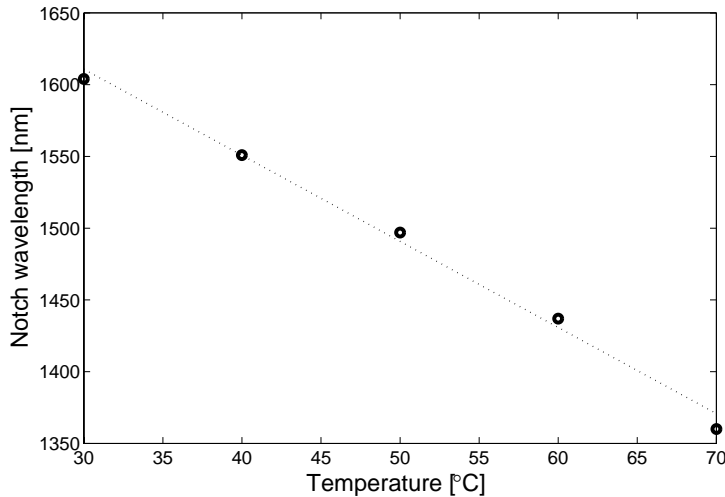
Figure 6.7: Thermal tunability of the PM LCPBG fiber device.
