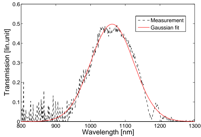
Figure 5.9: Measured transmission spectrum at 30°C of the tapered LMA-10 filled with MDA-00-1444. The amplitude of the Gaussian fit is 0.49, the mean value is 1062nm and the standard deviation is 62.25nm.
