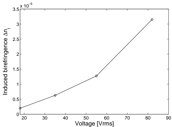
Figure 6.21: Induced birefringence as a function of voltage at \lambda = 1600\text{nm} and 25^\circ\text{C} .
