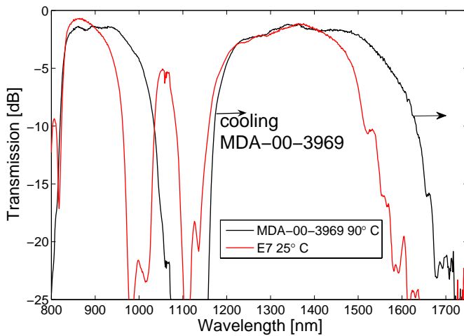
Figure 6.2: Transmission spectrum of LMA-10 filled with MDA-00-3969, 90^{\circ}\text{C} (black curve), together with the transmission spectrum of LMA-10 filled with E7, 25^{\circ}\text{C} (red curve). By decreasing the temperature of MDA-00-3969, the common transmission bands are narrowed.
