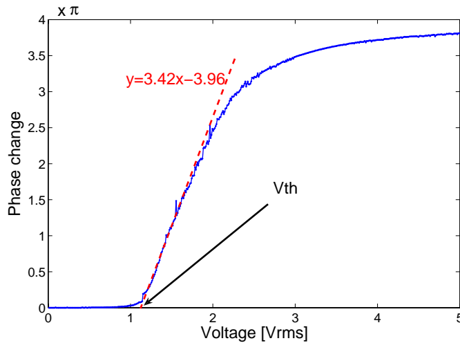
Figure 6.18: Voltage-dependent phase change of the \text{BaTiO}_3 nanoparticle-doped cell when a 10Hz square wave is applied to the cell.
