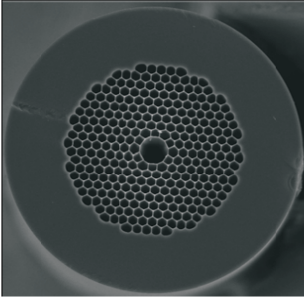
Figure 2.3: SEM of the end facet of a PBG fiber, HC-1550 (core diameter= 10.9\mu\text{m} , \Lambda = 3.8\mu\text{m} ). This fiber exhibits a bandgap around 1550nm. Picture appear courtesy of Crystal Fibre A/S.
