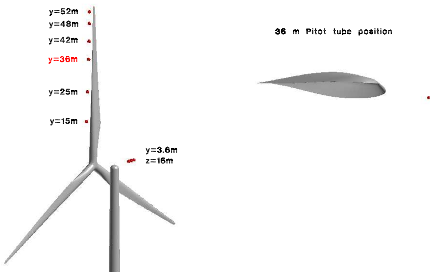
Figure 10. Positions of the velocity probes in the simulations.
