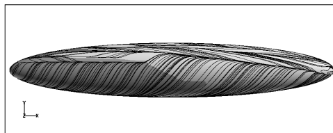
Figure 60. Intermittency and limiting streamlines on the surface of the spheroid at a Reynolds number of 7.2 \times 10^6 and 30 deg. incidence. The flow is from bottom left and the dark regions at the bottom left indicates laminar flow, while the light gray regions indicate turbulent flow.
