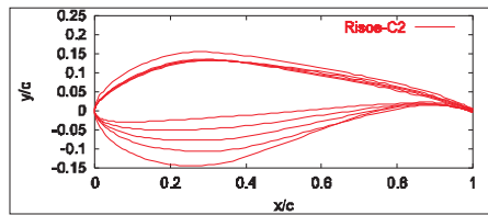
Figure 72. The Risø-C2 airfoil family.
