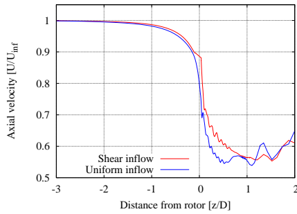
Figure 16. Normalised axial velocity along a line through the rotor plane at r/R=0.79 for the modern MW turbine.
