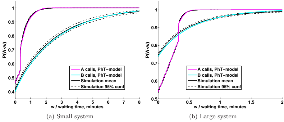
Figure 6: The Erlang approximation compared to simulations with 95% confidence intervals. The parameters used are k = 0.33\text{min}^{-1} , \lambda_a = 0.75\text{min}^{-1} , \lambda_b = 1.75\text{min}^{-1} , \mu_a = 0.33\text{min}^{-1} , \mu_b = 0.5\text{min}^{-1} , \gamma = 30\text{min}^{-1} , n_a = 2 , n_b = 5 , m = 10 , D_a = 50 and D_b = 300 for Figure 6a and k = 0.33\text{min}^{-1} , \lambda_a = 7\text{min}^{-1} , \lambda_b = 10\text{min}^{-1} , \mu_a = 0.33\text{min}^{-1} , \mu_b = 0.5\text{min}^{-1} , \gamma = 90\text{min}^{-1} , n_a = 20 , n_b = 27 , m = 30 , D_a = 40 and D_b = 200 for Figure 6b.
