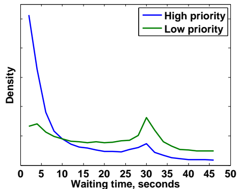
Figure 3.2: Waiting time distribution before abandonment. The peak at 30s coincides with a “please hold”-message.
