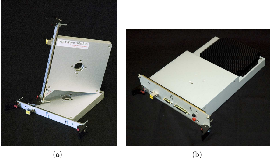
Figure 3.1.: (a) Rack-mountable DCF modules and (b) DCRA. The DCRA includes DCF module, pump unit, power supply and all required optical components. Courtesy of OFS Fitel Denmark ApS.
