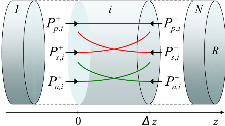
Figure 2.6.: The fiber amplifier is divided into N sections with reflectivity R at the fiber end connections. A single component of the forward and backward propagating pump, signal and ASE are seen to enter section i . In each section, the pump power due to pump p is assumed to be constant, thus providing a constant gain for the signal s and noise bin n across the section.
