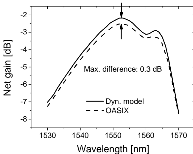
Figure A.1.: Comparison of calculated net gain vs. wavelength in 80 km TW-REACH. The fiber is backward-pumped with 300 mW pump at 1453 nm.
