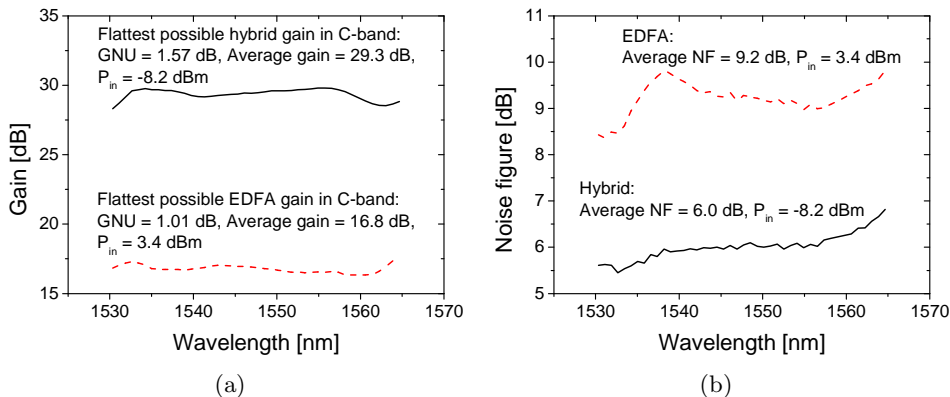
Figure 3.10.: (a) The flattest possible gain using the hybrid amplifier (solid) and the EDFA (dashed). (b) The noise figure of the hybrid amplifier (solid) and the EDFA (dashed). The input powers are -8.2 dBm and 3.4 dBm, respectively.
