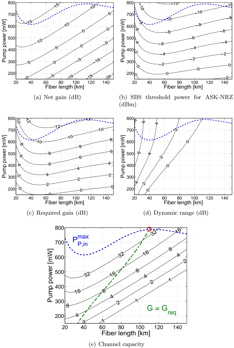
Figure 4.5.: Calculated results for a 50% bidirectionally pumped link.
