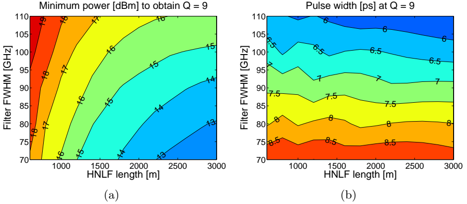
Figure 5.9.: Calculated: (a) Minimum power needed to obtain Q = 9.0 , or 3 dB improvement. (b) Output pulse width vs. filter width and HNLF length. HNLF dispersion is D = -0.5 ps/nm/km.
