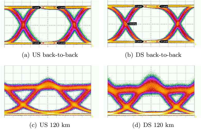
Figure 4.9.: Measured eye diagrams before and after transmission. Time scale is 16.3 ps/div – 17.0 ps/div.
