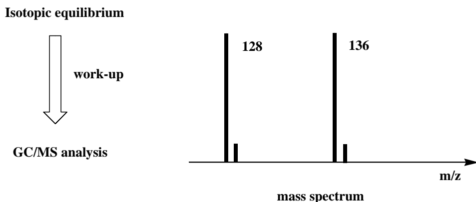
Figure 4.12 Work-up and stable isotope dilution illustrated by the analysis of naphthalene
