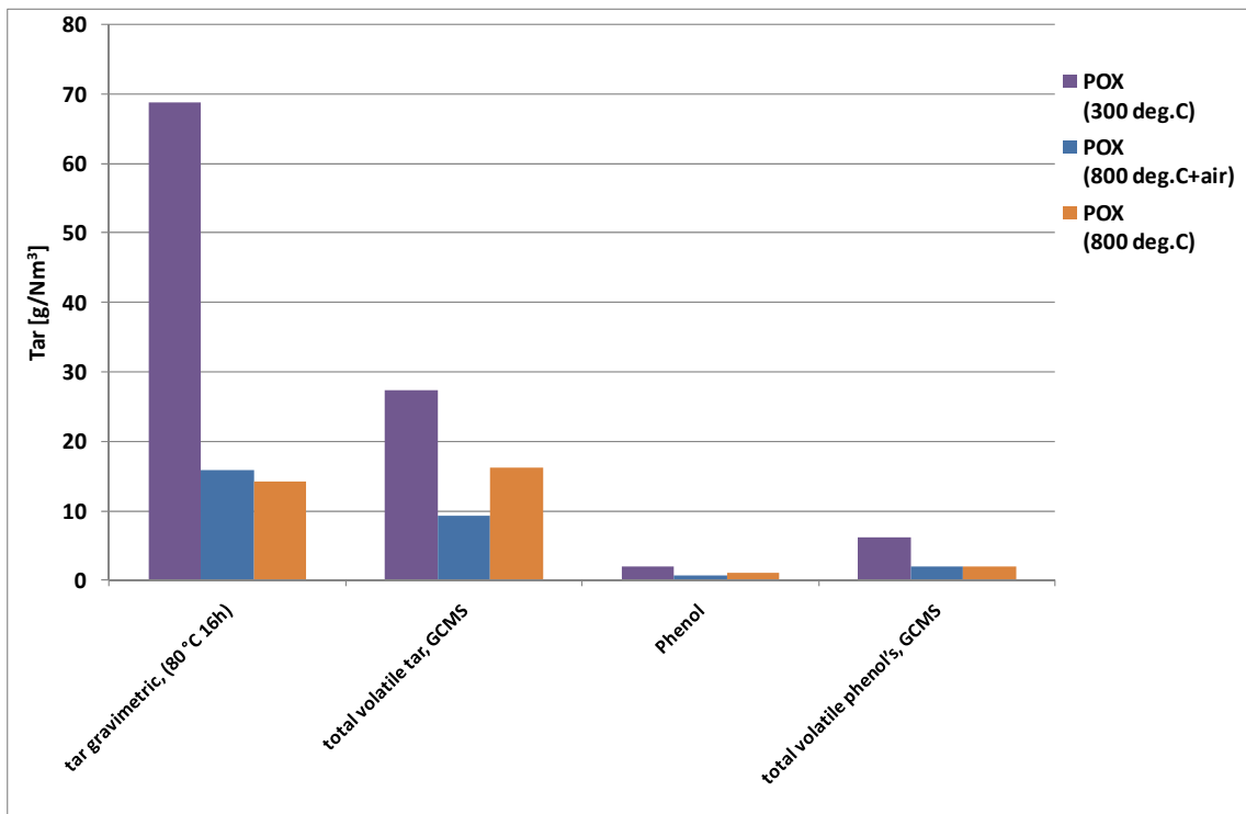
Figure 4.21 Overall tar content of producer gas leaving the POX reactor
