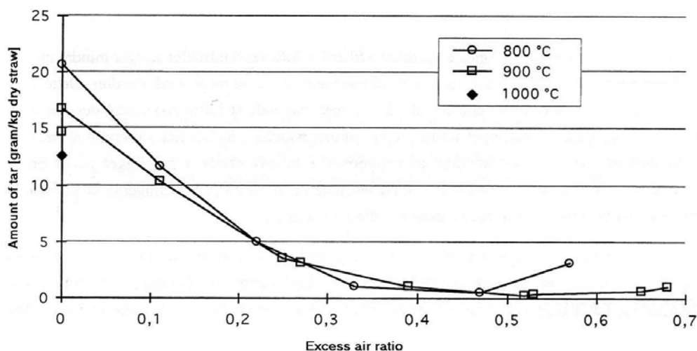
Figure 4.1 Results from partial oxidation experiments
