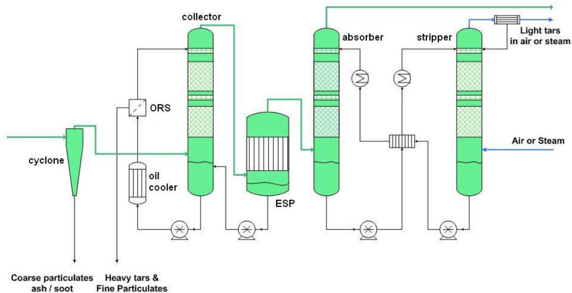
Figure 3.2 OLGA scheme
