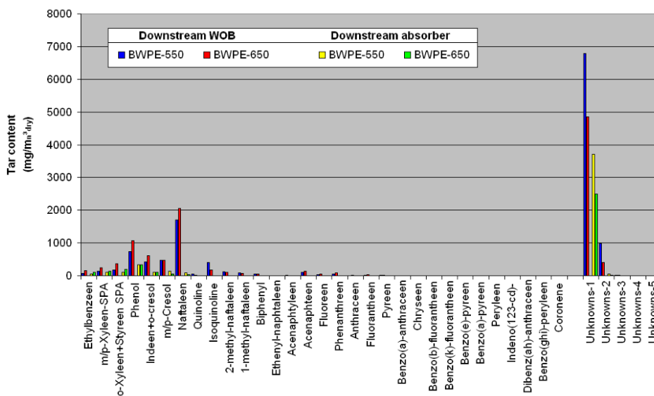
Figure 3.12 OLGA performance downstream beech wood / PE gasification at 550 & 650°C
