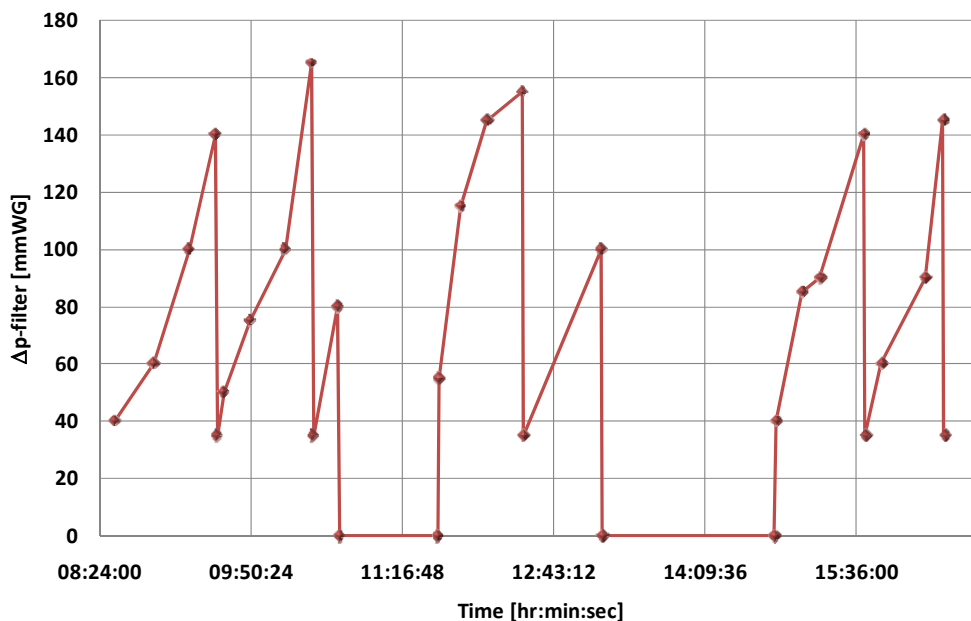
Figure 4.16 Measurement of pressure drop across back house filter on September 24 th 2009
