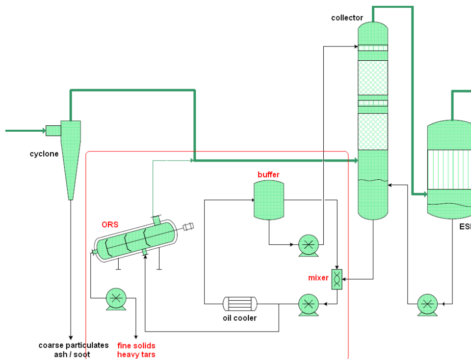
Figure 3.5 ORS scheme
