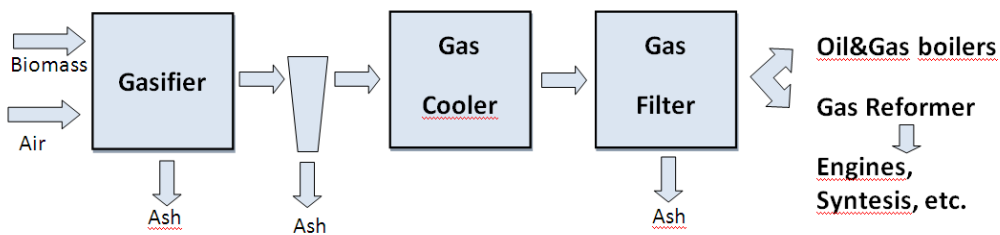
Figure 5.2 Principal diagram of Low Temperature gasifier with gas cooling and gas filter
