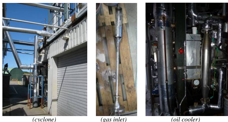
Figure 3.4 OLGA pilot scale modifications
