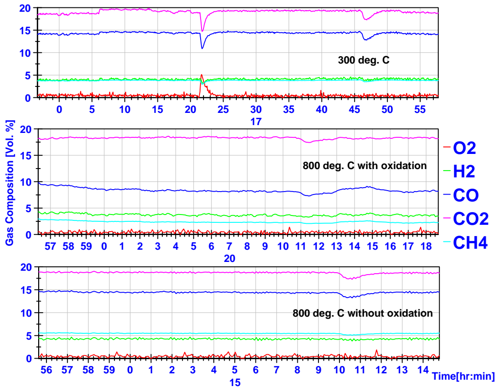
Figure 4.20 Gas composition of producer gas leaving the POX
