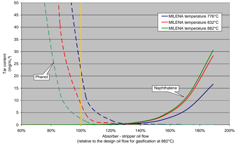
Figure 5.1 MILENA 10 MW th tar removal efficiency for different gasification temperatures
