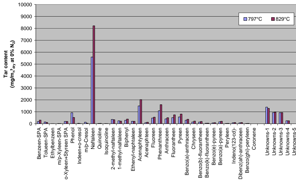
Figure 2.5 MILENA pilot scale tar composition for clean wood pellets & olivine (air on riser)
