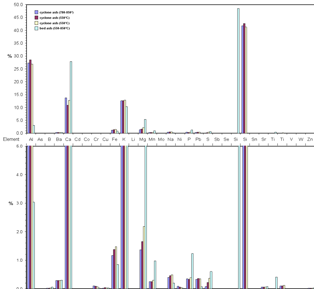
Figure 2.11 WOB lab scale elemental composition of ashes for beech wood / PE
