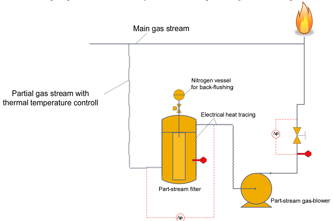
Figure 4.5 Diagram of the filtration set-up
