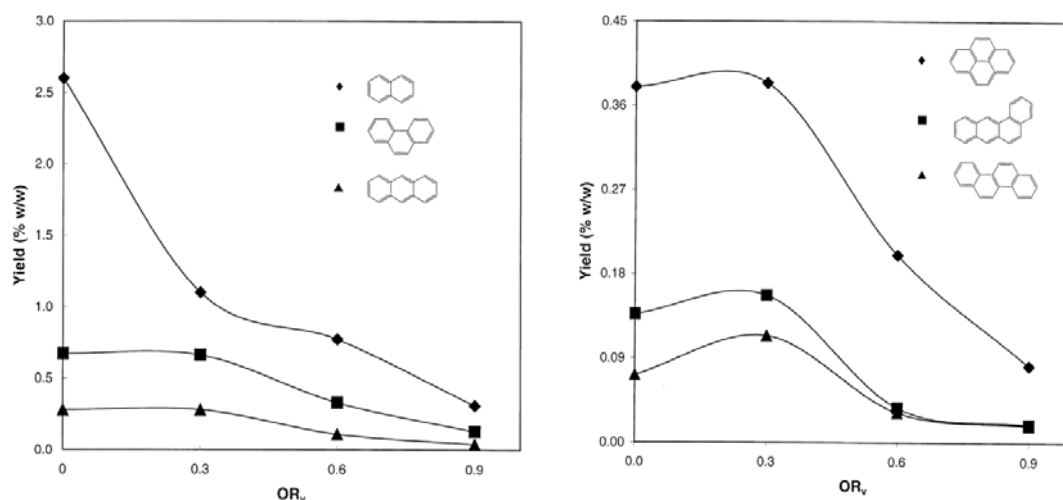
Figure 4.2 Yields of naphthalene, phenanthrene and anthracene (left) as well as pyrene, benzanthracene and chrysene (right) as function of the excess air ratio
