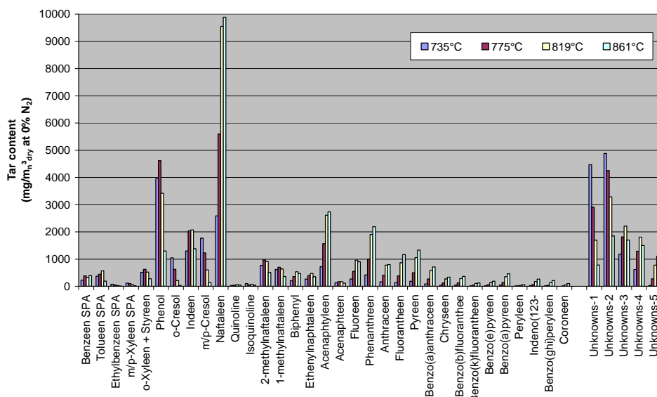
Figure 2.3 MILENA lab scale tar composition for beech wood & sand
