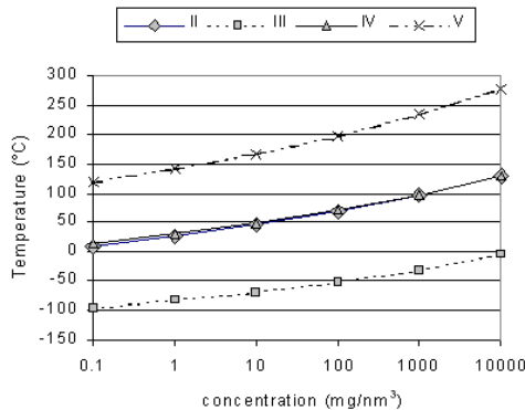
Figure 2.6 Relation between tar dew point and concentration
