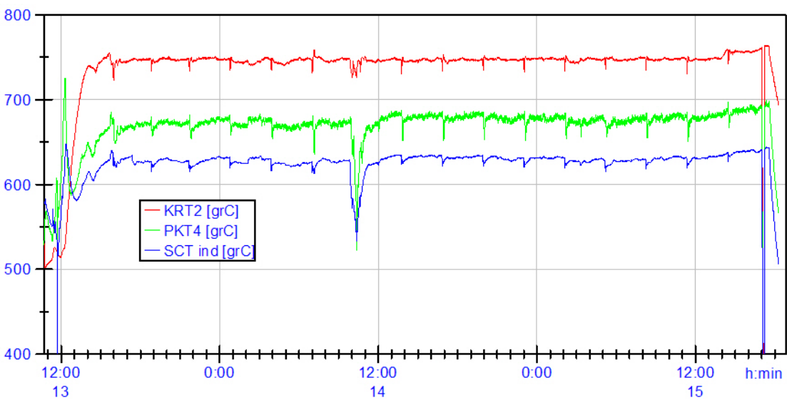
Figure 2.17 Important process temperatures from 100 kW th LT-CFB test no. 8
