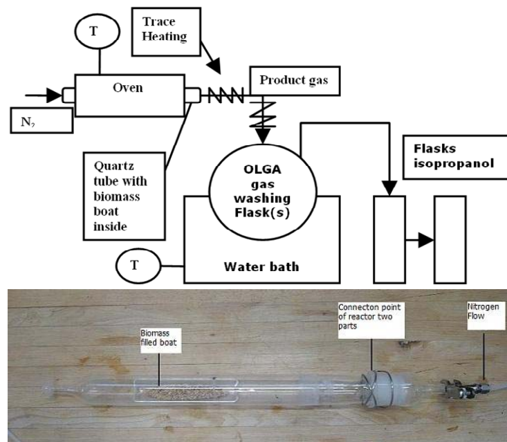
Figure 3.7 OLGA micro scale facility
