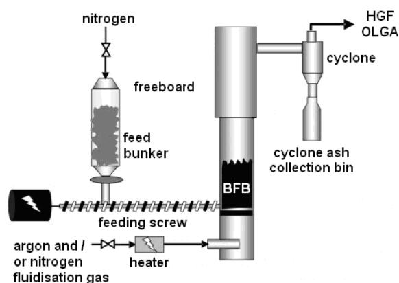
Figure 2.7 WOB scheme
