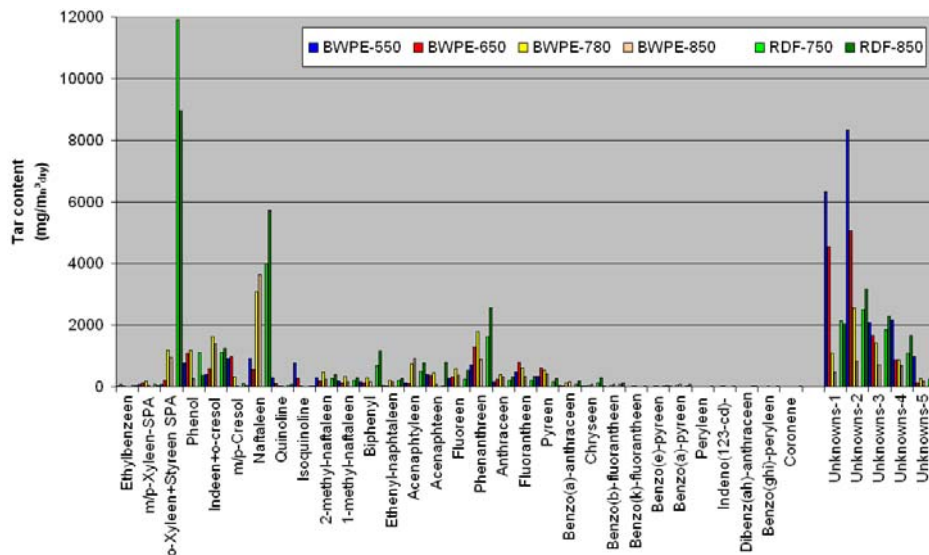
Figure 2.9 WOB lab scale tar composition for RDF and for beech wood / PE (bulk)
