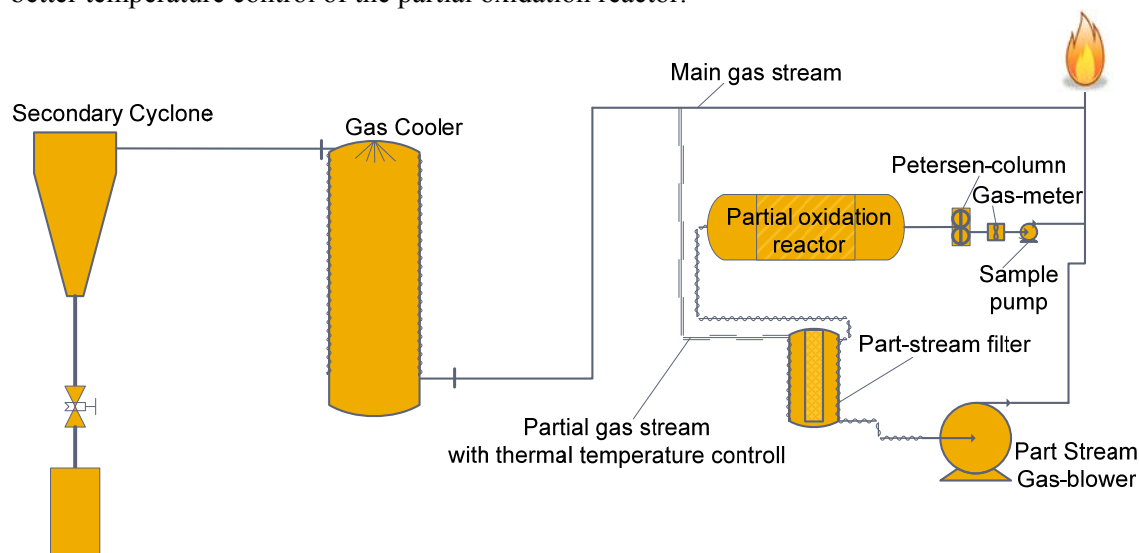
Figure 4.7 Diagram of the gas cleaning set-up
