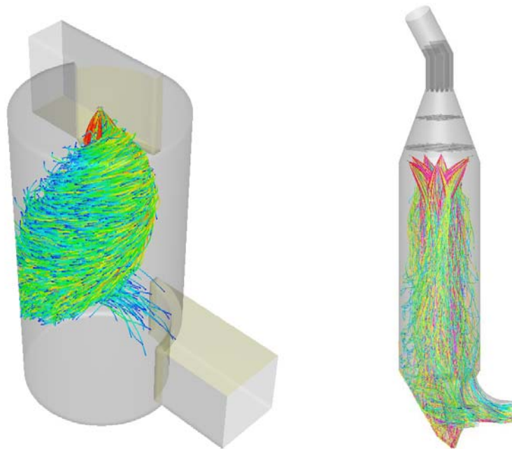
Figure 5.3 Compact cooler design for gas coolers below 10 MW th (left) and cooling tower design for gas coolers above 10 MW th (right)
