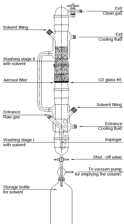
Figure 4.9 The Petersen Column setup
