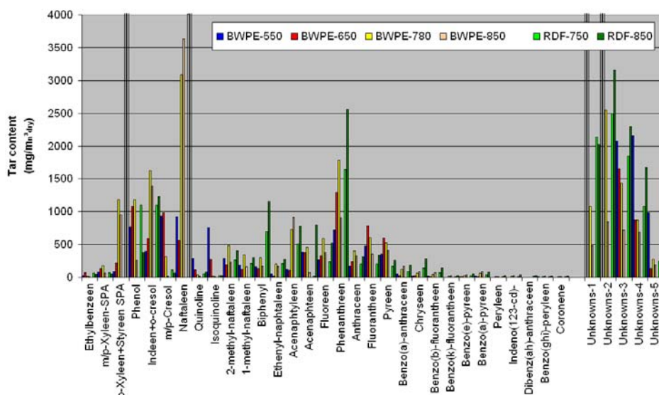
Figure 2.10 WOB lab scale tar composition for RDF and for beech wood / PE (detailed)
