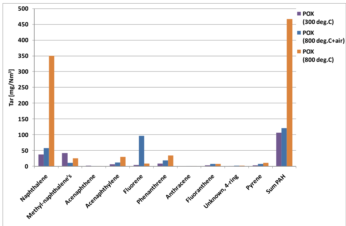
Figure 4.22 PAH-tar content of producer gas leaving the POX reactor
