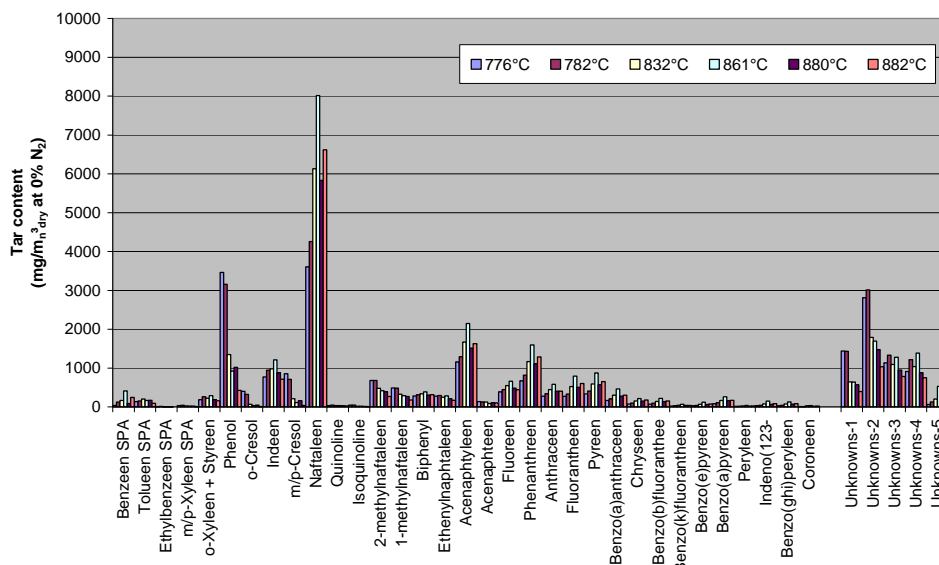
Figure 2.4 MILENA lab scale tar composition for beech wood & olivine
