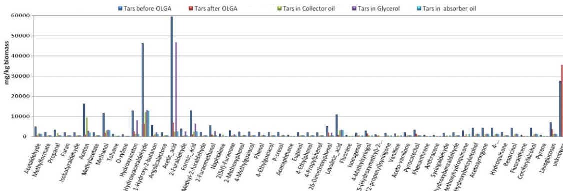
Figure 3.9 OLGA micro scale with biodiesel scrubber
