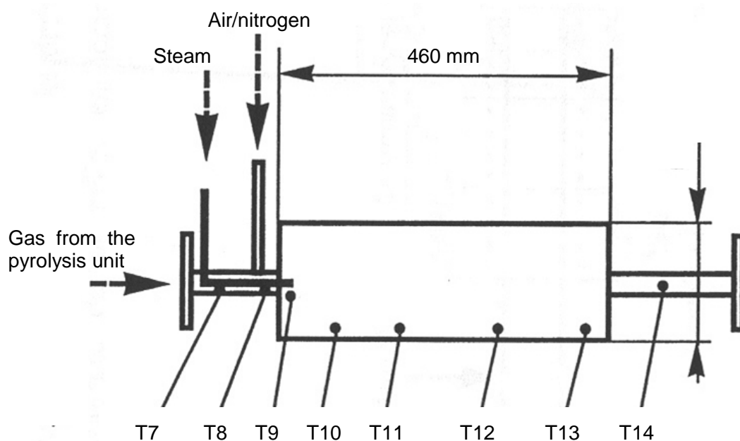
Figure 4.8 Schematic drawing of the partial oxidation reactor
