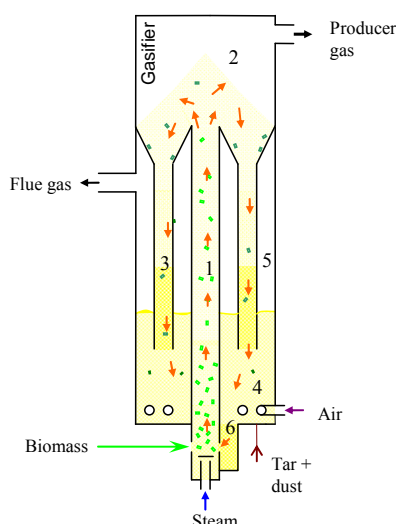
Figure 2.1 MILENA scheme
