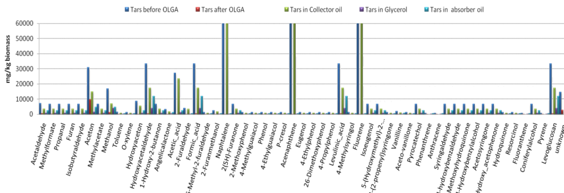
Figure 3.10 OLGA micro scale with glycerol scrubber
