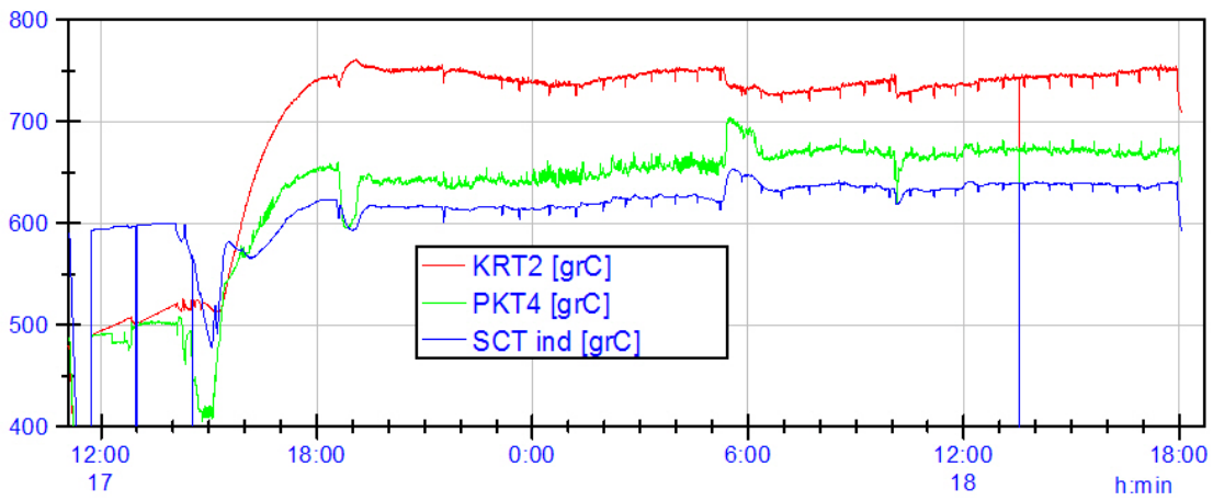
Figure 2.16 Important process temperatures from 100 kW th LT-CFB test no. 6
