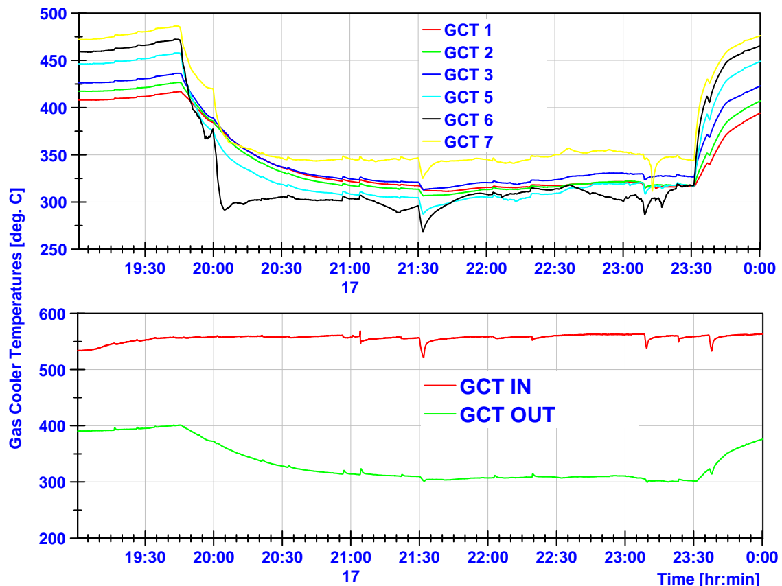
Figure 4.13 Gas cooler temperatures from tests during gasifier operation on pectin residues
