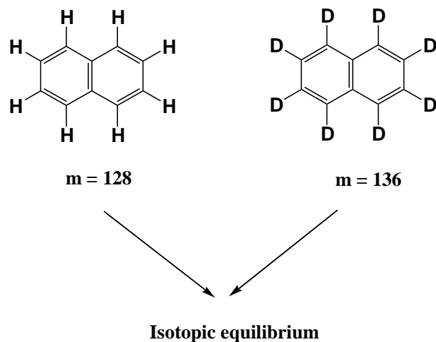
Figure 4.11 Stable isotope dilution illustrated by the analysis of naphthalene
