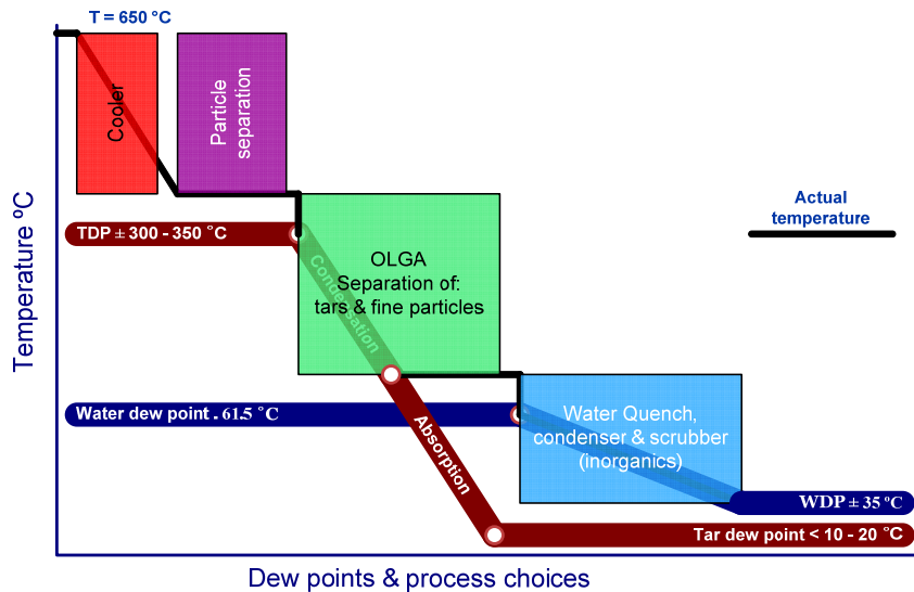
Figure 3.20 LT-CFB 100 kW th basic OLGA working principle
