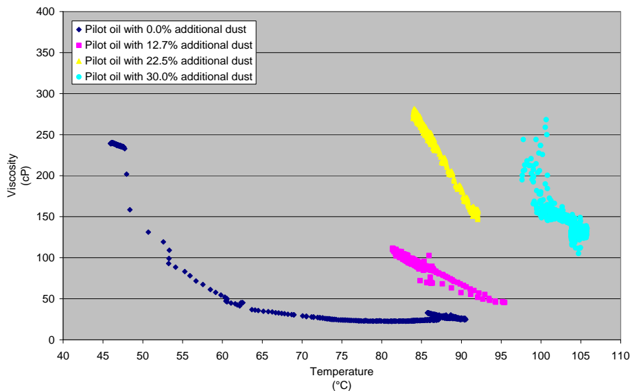
Figure 3.18 ORS pilot scale effect of dust/tar ratio on oil viscosity
