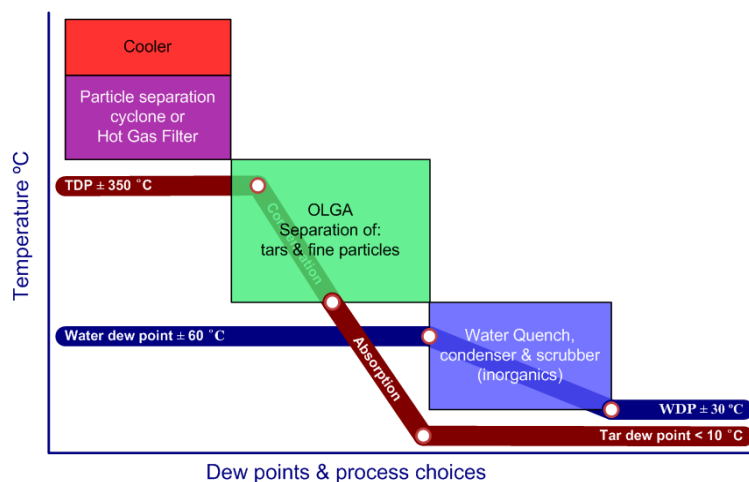
Figure 3.1 OLGA equipment selection based on dew points
