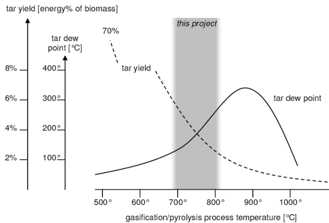
Figure 1.2 Effect of temperature on tar yield & dew point
