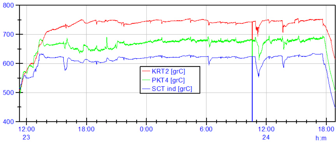
Figure 2.15 Important process temperatures from 100 kW th LT-CFB test no. 5
