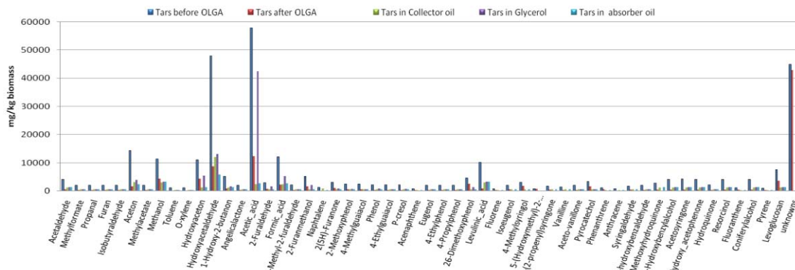
Figure 3.8 OLGA micro scale with RME scrubber
