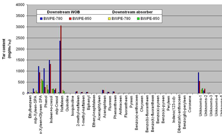
Figure 3.13 OLGA performance downstream beech wood / PE gasification at 780 & 850°C
