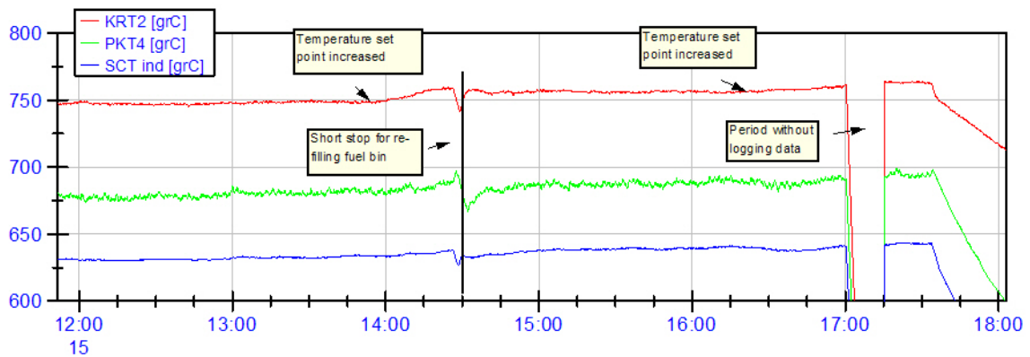
Figure 2.18 Important process temperatures from last 6 hours of 100 kW th LT-CFB test no. 8
