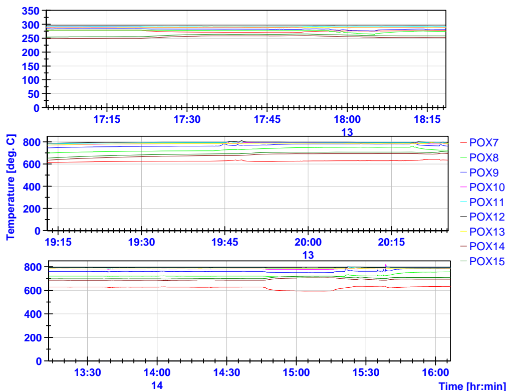
Figure 4.19 The POX temperatures during the experiments
