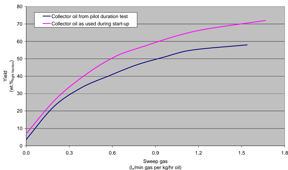
Figure 3.19 ORS pilot scale recovery yield of the light fraction at 320°C
