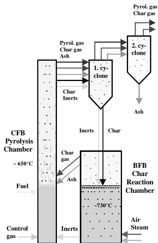
Figure 2.12 LT-CFB flow diagram (simple version with a hot 2 nd cyclone for gas cleaning)
