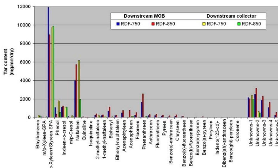
Figure 3.11 OLGA performance downstream RDF gasification at 750 & 850°C
