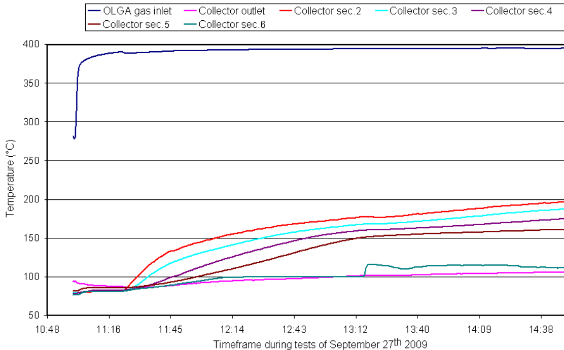
Figure 3.14 OLGA pilot scale temperature profile
