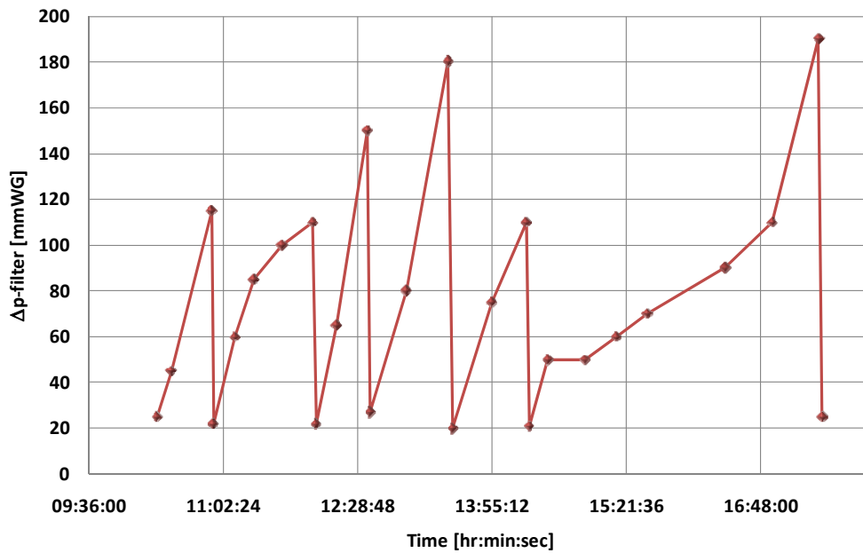
Figure 4.17 Measurement of pressure drop across back house filter on November 18 th 2009
