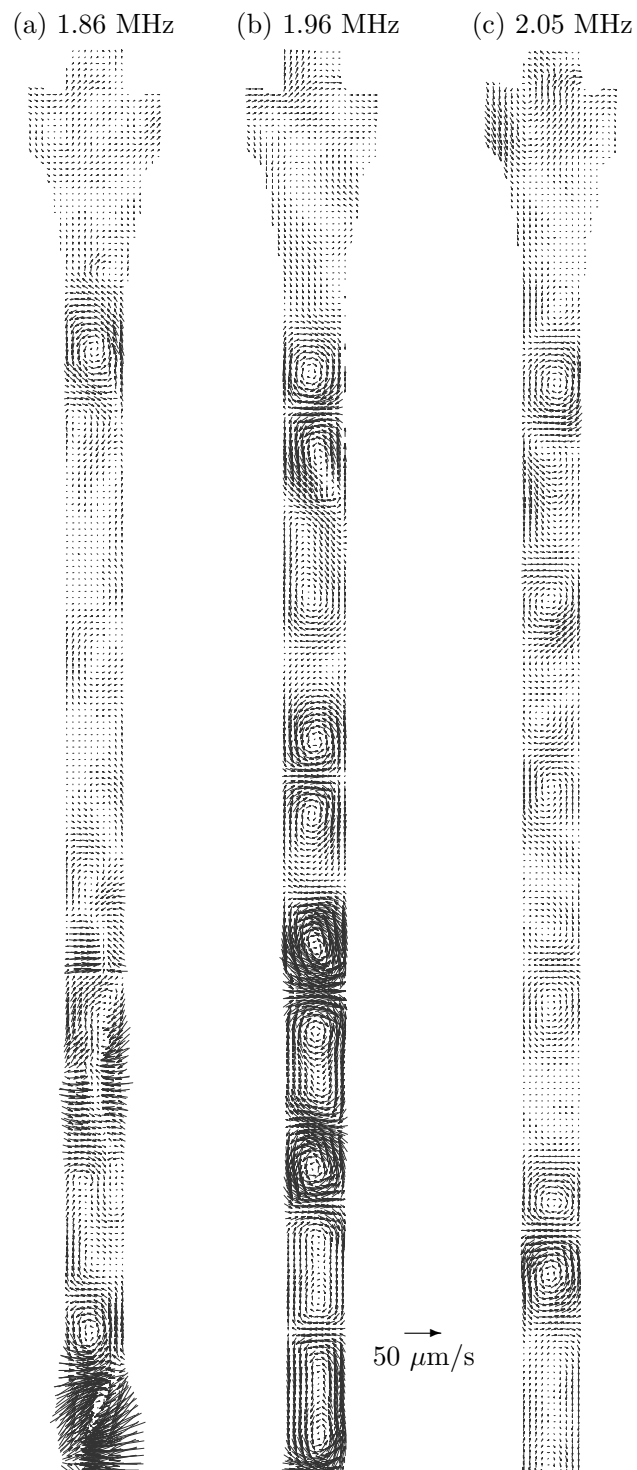
Figure 5.7: Velocity vectors of fluid motion caused by acoustic streaming. 1 \mu\text{m} tracer particles were used for recordings at (a) 1.86 MHz (b) 1.96 MHz and (c) 2.05 MHz. Reference vector is shown for 50 \mu\text{m/s} .
