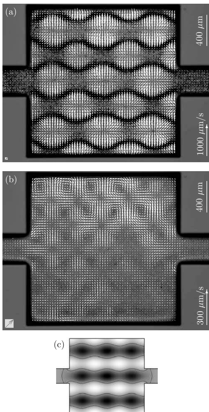
Figure 4.4: Acoustic streaming and radiation forces at the 2.17 MHz acoustic resonance. (a) Experiments on 5 \mu\text{m} beads similar to Fig. 4.3(a) showing that the acoustic radiation force dominates for large particles. (b) Experiments on 1 \mu\text{m} beads. Acoustic streaming dominates and the small beads act as tracers for the motion of the liquid. The resulting vortex structure in the flow-field prevents particle accumulation at the pressure nodes. (c) Gray-scale plot of numerical simulation in the 2D chamber model of the corresponding acoustic pressure eigenmode. Nodal lines are shown in black.
