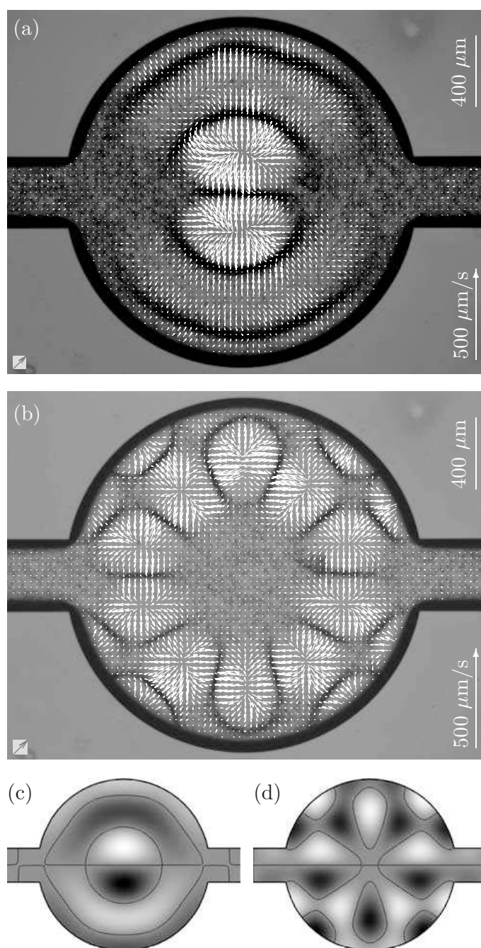
Figure 4.3: Acoustic radiation force. (a) Experiments on 5 \mu\text{m} beads at the 1.936 MHz acoustic resonance. The white PIV-vectors indicate the initial bead velocities pointing away from pressure anti-nodes immediately after the piezo-actuation is applied. The picture underneath the PIV-vector plot shows the particles (black) gathered at the pressure nodal lines 3 seconds later. (b) As in panel (a) but now at 2.417 MHz. (c) and (d) Gray-scale plots of numerical simulations in the 2D chamber model of the corresponding acoustic pressure eigenmodes. Nodal lines are shown in black.
