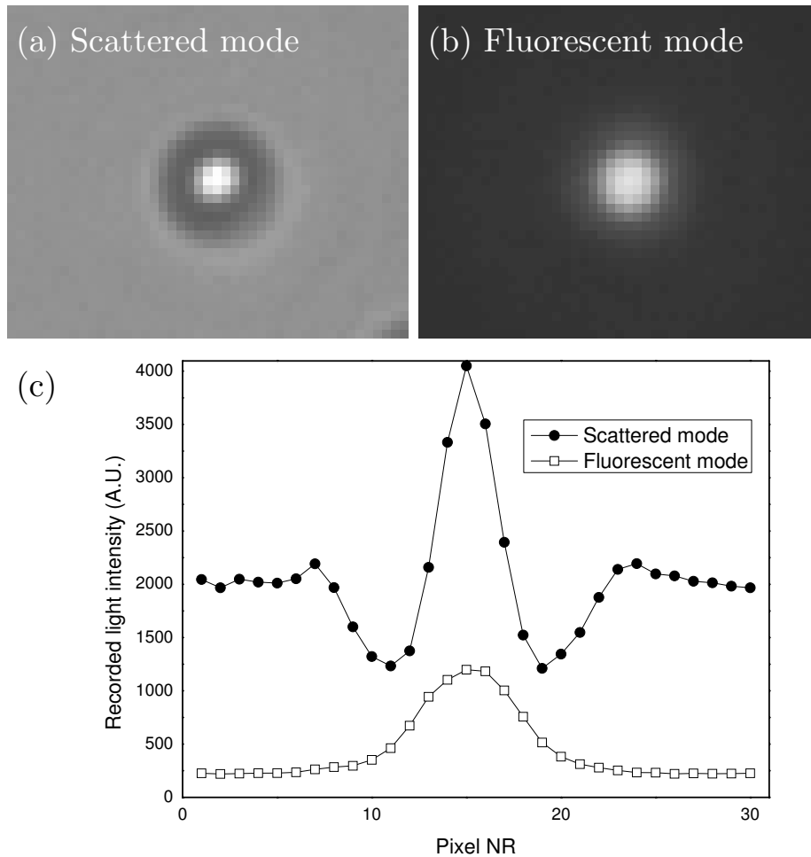
Figure 3.9: Recordings of a 1\ \mu\text{m} particle with a 63\times magnification objective ( 0.63\times tv-adapter) in (a) scattered mode, back-lit ( 50\ \mu\text{s} pulse) and (b) fluorescent mode, front-lit ( 2\ \text{ms} pulse). (c) The respective gray-values on the pixel pitch for a line drawn over the center of the particle.
