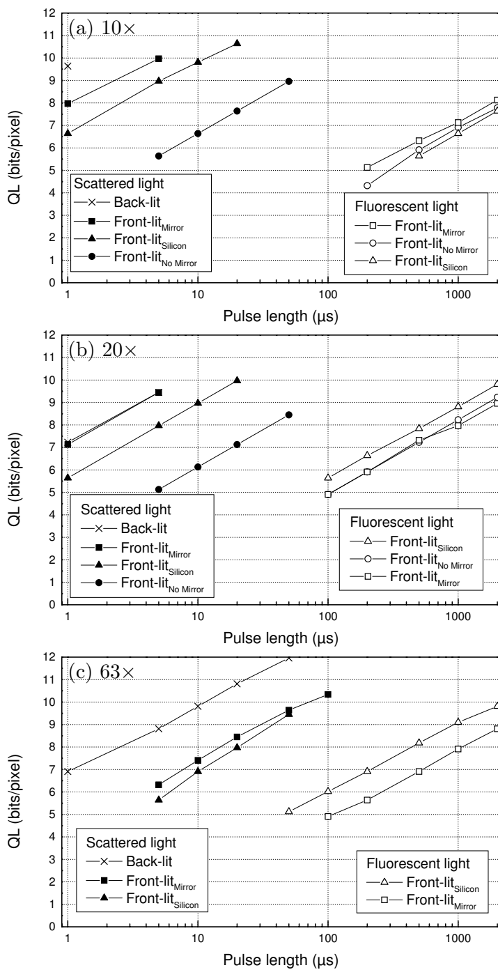
Figure 2.6: Quantization levels ( QL ) for particle images with (a) a 10 \times objective, (b) a 20 \times objective and (c) a 63 \times objective in the front-lit and back-lit configurations. Note that the y-axis increments are not linear but represent a \log_2 scale.
