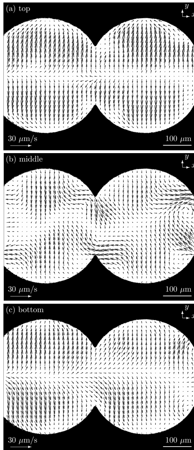
Figure 5.13: Circle chip acoustically actuated at 2.013 MHz. The motion of 1 \mu\text{m} particles is measured at (a) the top, (b) the middle and (c) the bottom of the microchip. The opposing directions of the velocity vectors at the different measurement depths clearly indicates the presence of 3D streaming motion.
