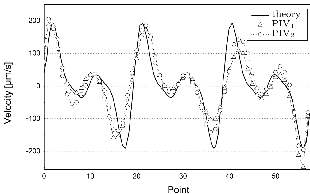
Figure 4.9: Vertical cross-sectional plots of the measured velocity in the y -direction (PIV 1 ) 330 \mu\text{m} left and (PIV 2 ) 330 \mu\text{m} right of the center of the chamber. The full line (theory) is the velocity in the y -direction calculated by Eq. (4.6) as p_2 \nabla p_2 using COMSOL Multiphysics, and with an amplitude fitted to match the velocity measurements.
