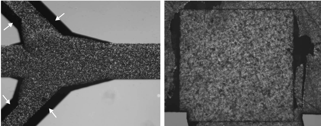
Figure 3.10: Left panel: Recording of a microdevice fabricated in silicon substrate filled with 5\ \mu\text{m} tracer particles. The slanted walls (indicated by the white arrows) from the anisotropic wet etching appear black on the image frame, and no velocity vectors can be obtained from this region when recording in scattered mode. Right panel: Image of a piezo-element inside a microchannel (clear fluid, no particles added). The rough reflecting surface of the piezo-element has a speckled appearance under illumination, which makes recording in scattered mode problematic.
