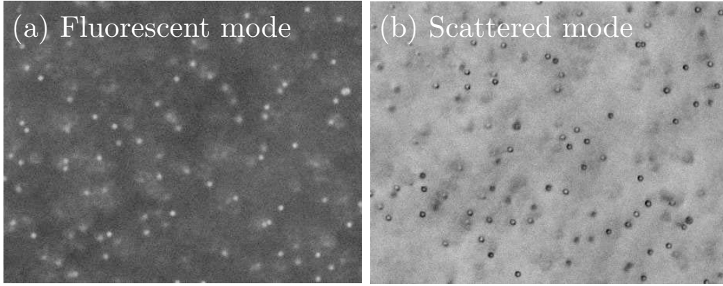
Figure 3.8: Images of particles in a micro-structure recorded with a 63\times magnification objective (mounted with a 0.63\times tv-adaptor) in (a) fluorescent mode and (b) scattered mode. The out-of-focus particles give rise to a background glow in (a) and to a “background shade” in (b), in both cases diminishing the contrast between the particles in focus and the background. The micro-structure was fabricated in a silicon substrate and the images were recorded at a depth of 45\ \mu\text{m} .
