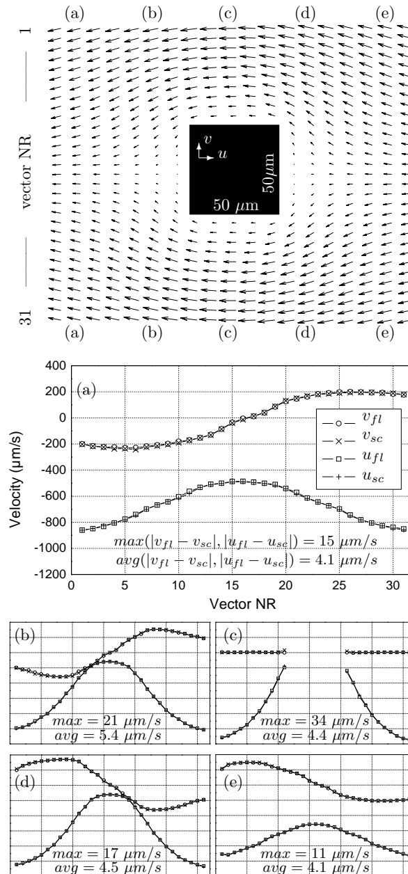
Figure 2.8: Top panel shows velocity vector fields around a 50 \mu\text{m} \times 50 \mu\text{m} pillar recorded in fluorescent mode. For clarity, only every second velocity vector in the channel flow direction is shown. Unit vectors equal 1 \text{ mm/s} . A comparison between velocity vectors calculated from images recorded in fluorescent _{fl} mode and scattered _{sc} mode is seen in panels (a)–(e). The plots are showing the u and v velocities for five different cross sections over the width of the channel. The scale bars and symbols in panels (b)–(e) are the same as in panel (a), even though not shown.
