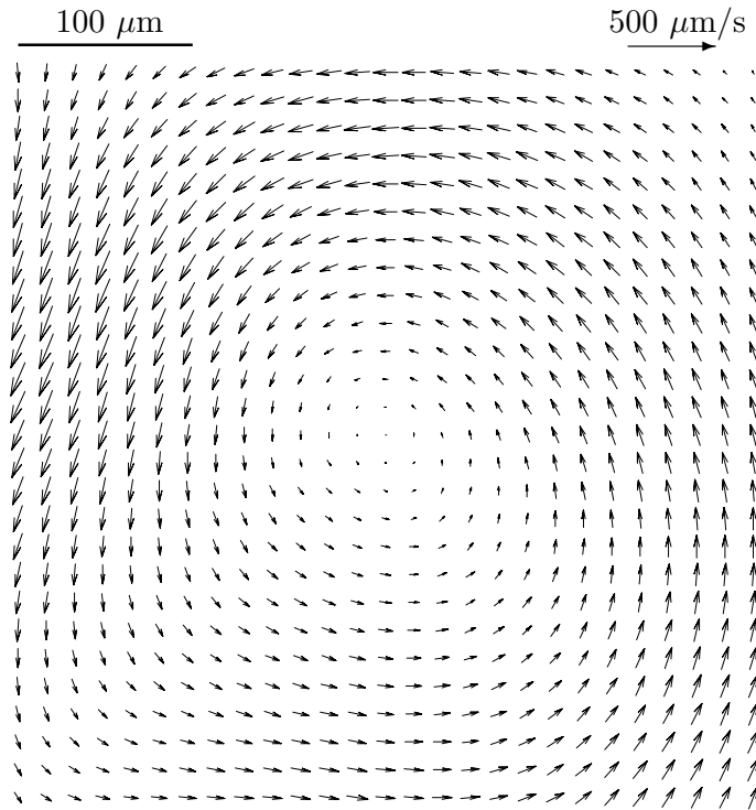
Figure 4.7: Micro-PIV velocity vector plot of streaming motion in the center of the square chamber at 2.17 MHz. Images were recorded with a 20\times objective and a 0.63\times Tv-adaptor, and milk was used as tracer particles.
