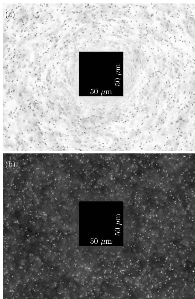
Figure 2.7: Background subtracted image frames of 1\ \mu\text{m} particles flowing around a 50\ \mu\text{m} \times 50\ \mu\text{m} pillar structure at a depth of 45\ \mu\text{m} . (a) Picture recorded in scattered mode, the bright field filter cube is inserted, and the particles appear dark in relation to the background. (b) Picture recorded in fluorescent mode, the I3 filter cube is inserted, and the particles appear bright in relation to the background. Both images are recorded with a t_p of 100\ \mu\text{s} .
