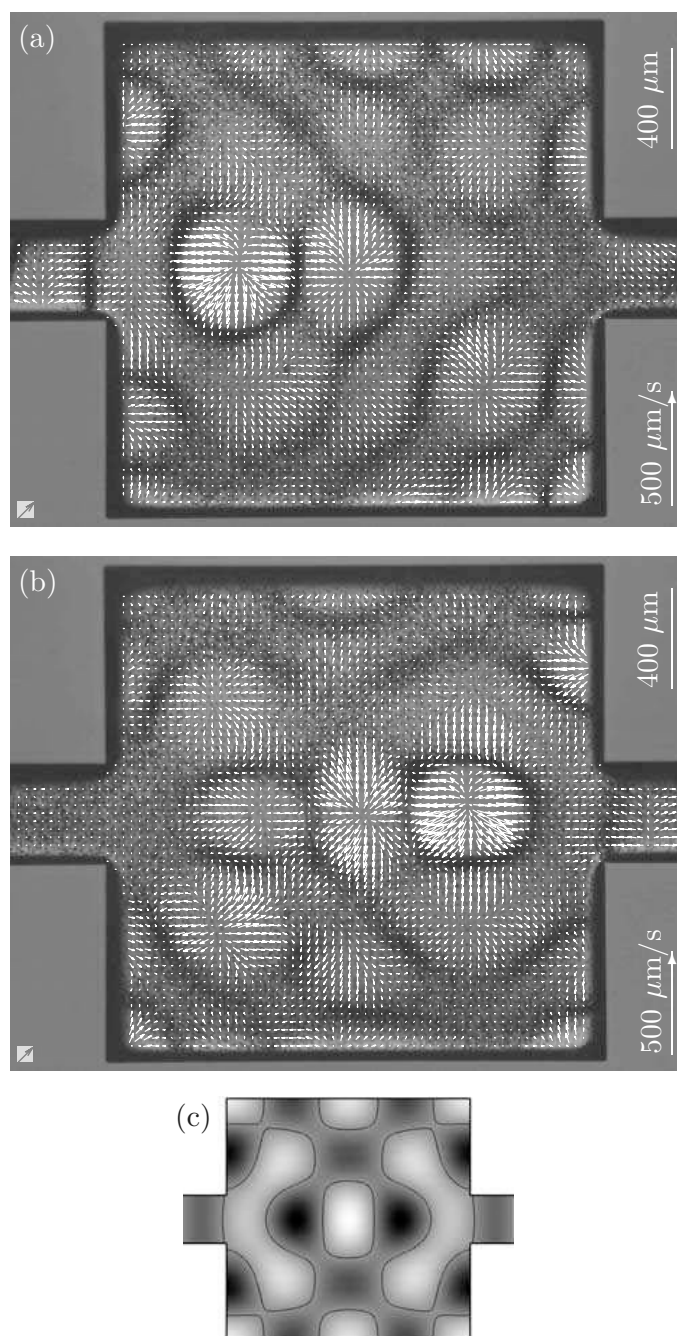
Figure 4.5: Splitting of a two-fold degenerate acoustic resonance due to geometrical asymmetry. (a) Acoustic radiation force as in Fig. 4.4(a) on 5 \mu\text{m} beads at the 2.06 MHz resonance. (b) The closely related 2.08 MHz resonance for the same system. (c) Gray-scale plot of numerical simulation in the left-right symmetric 2D chamber model of the corresponding two-fold degenerate, un-split, acoustic pressure eigenmode. Nodal lines are shown in black.
